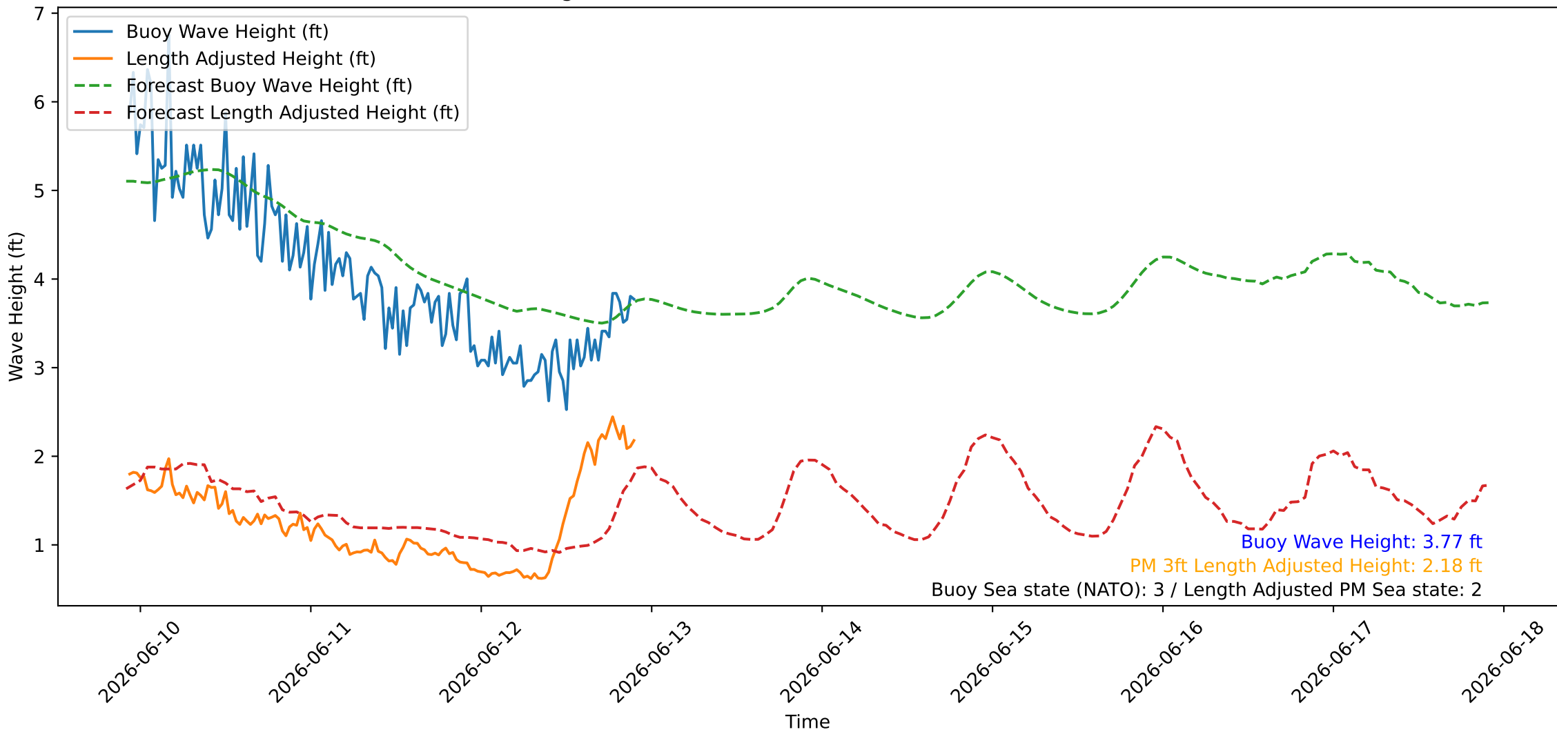
Wave Heights over Time for Red Beach at 2026-06-12 22:20:47
