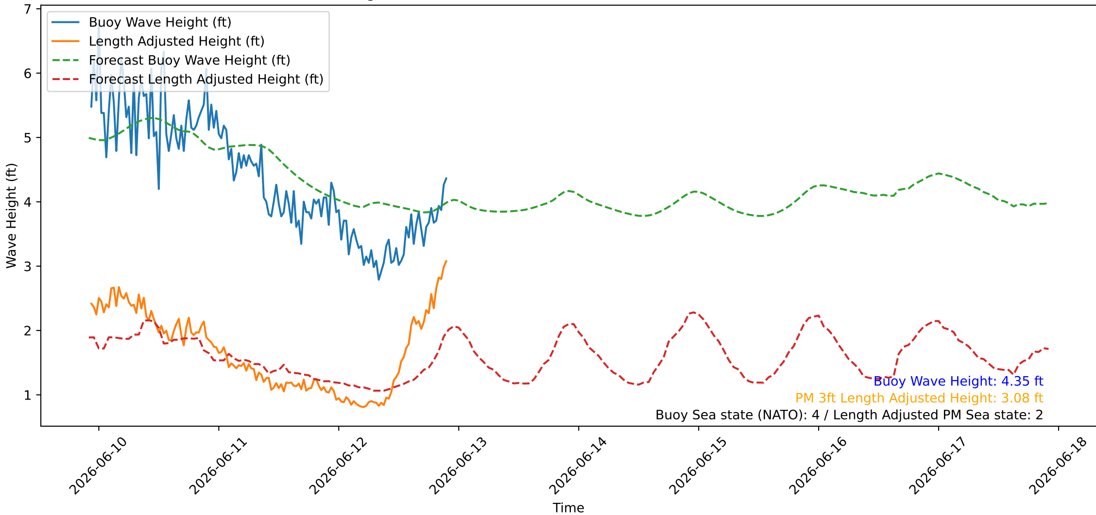
Wave Heights over Time for Oceanside Harbor at 2026-06-12 22:20:26
