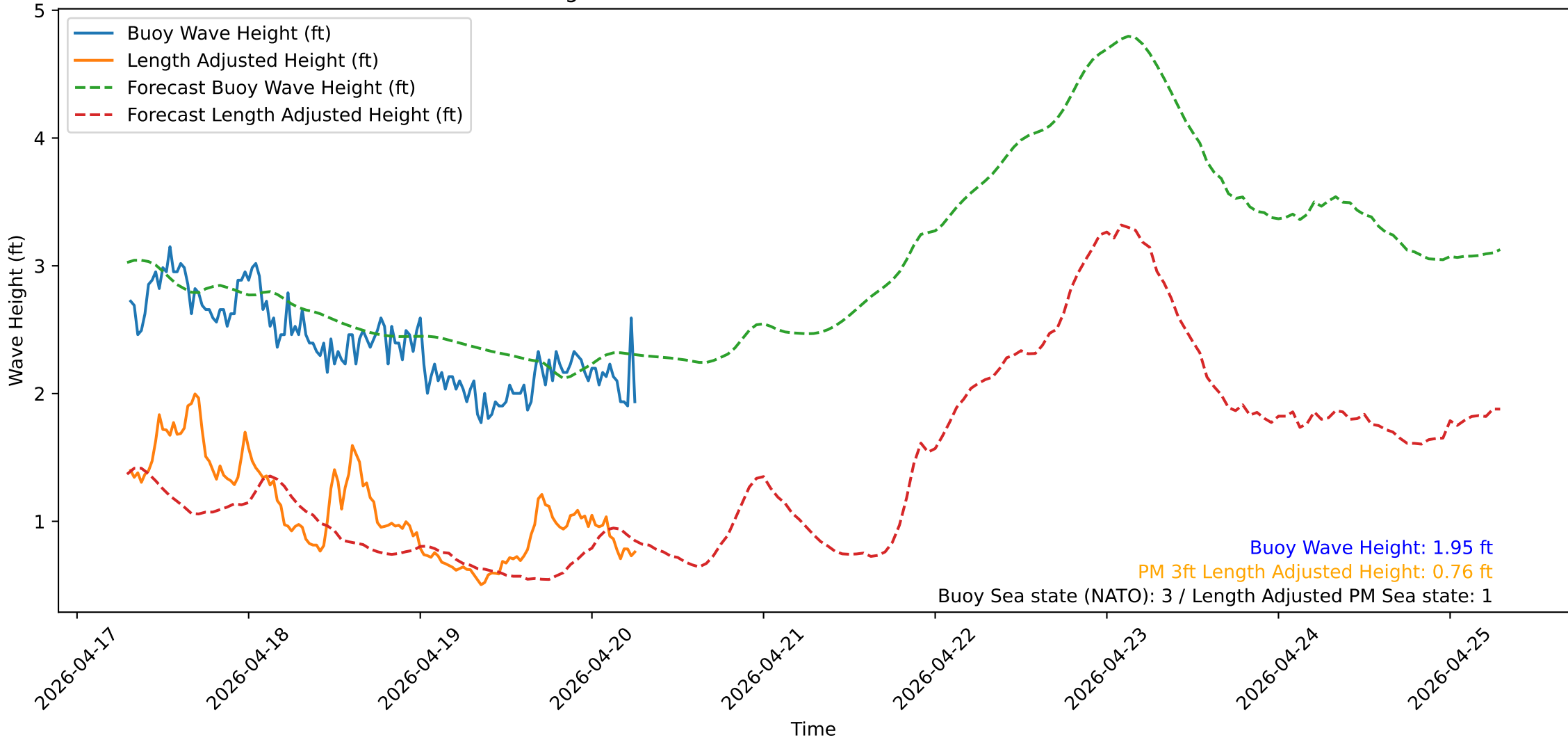
Wave Heights over Time for Red Beach at 2026-04-20 07:00:50
