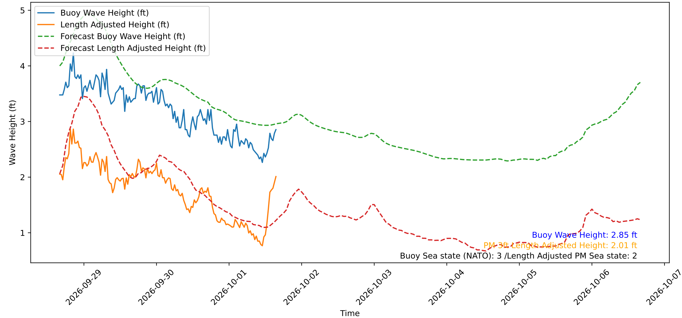
Wave Heights over Time for Oceanside Harbor at 2026-10-01 16:10:29
