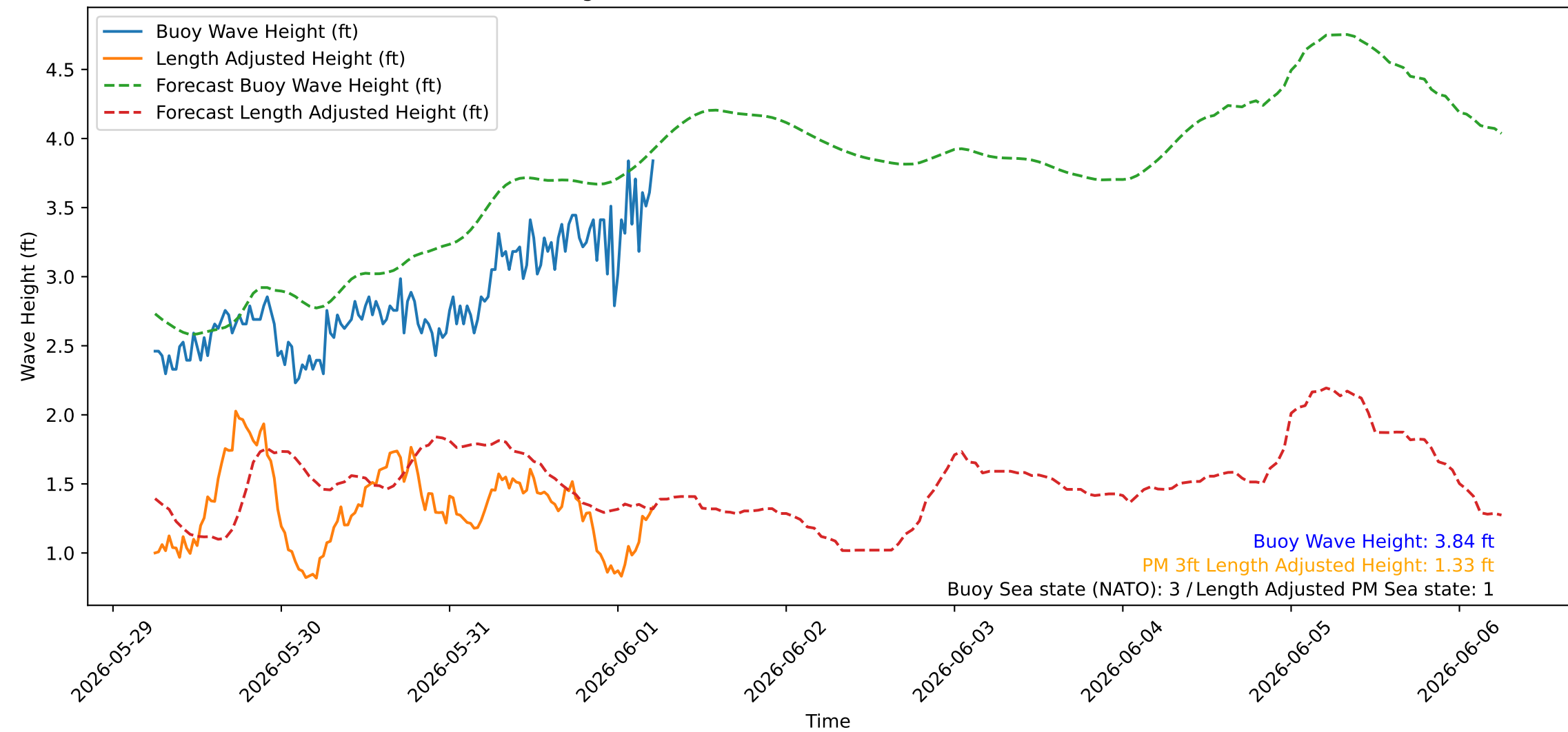
Wave Heights over Time for Red Beach at 2026-06-01 05:50:47
