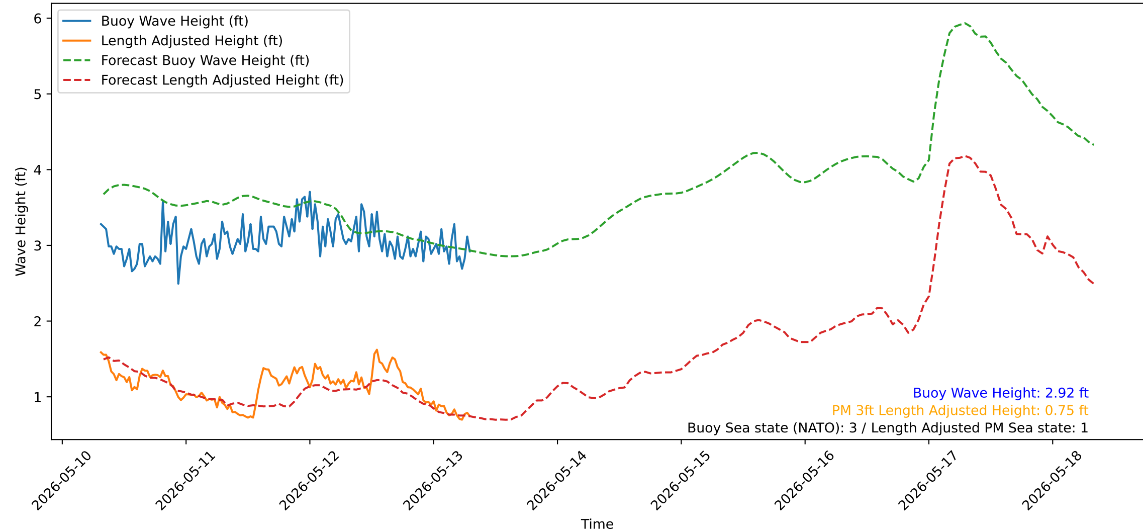
Wave Heights over Time for Oceanside Harbor at 2026-05-13 07:40:31
