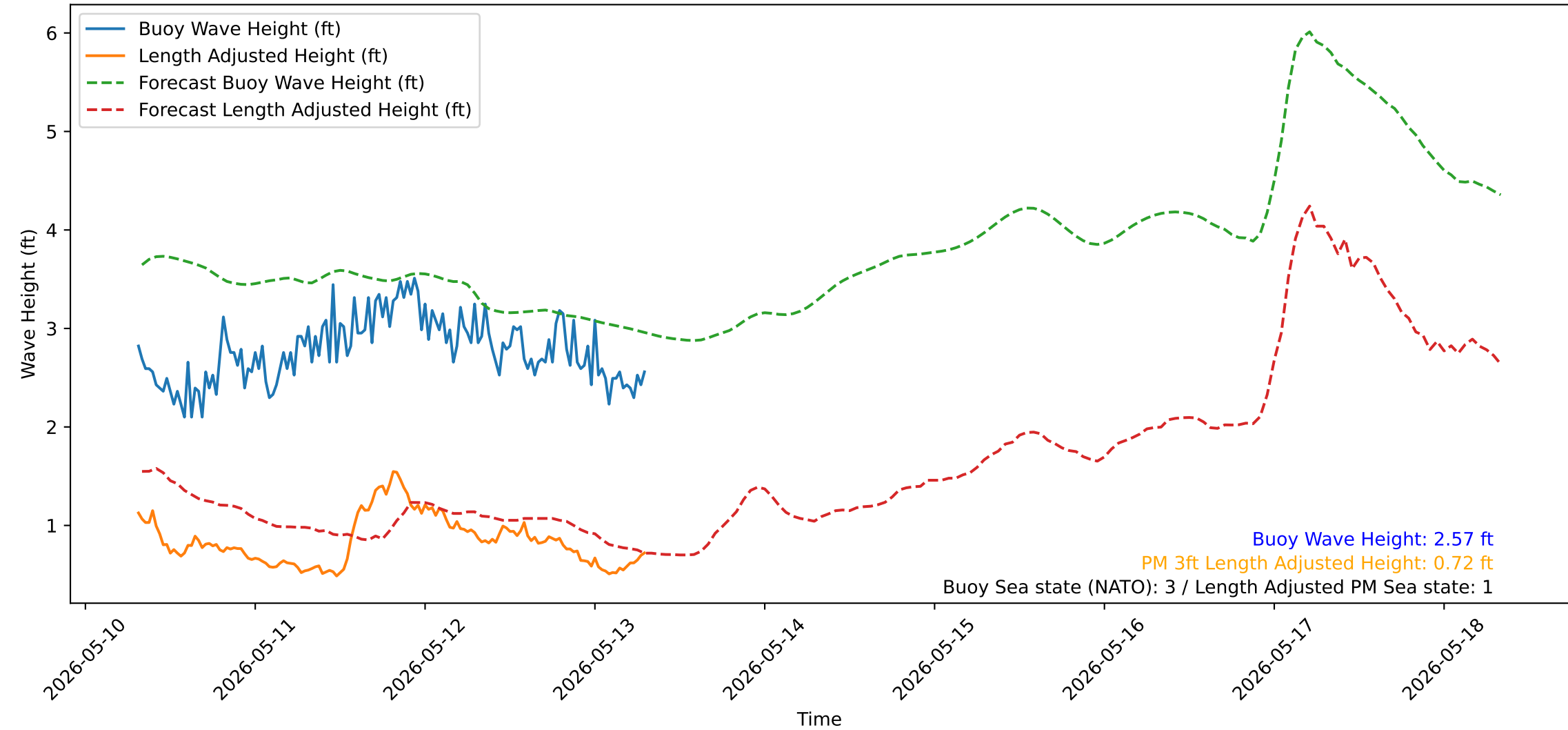
Wave Heights over Time for Green Beach at 2026-05-13 07:41:13
