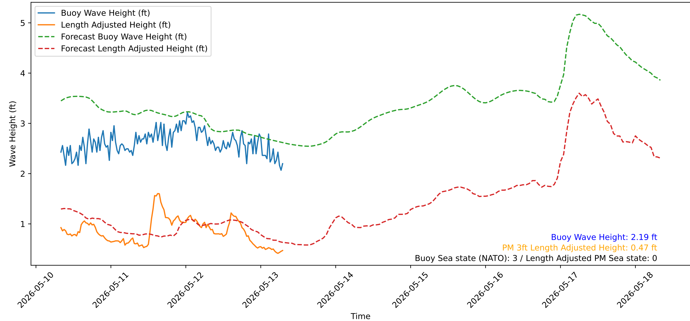
Wave Heights over Time for Red Beach at 2026-05-13 07:40:50
