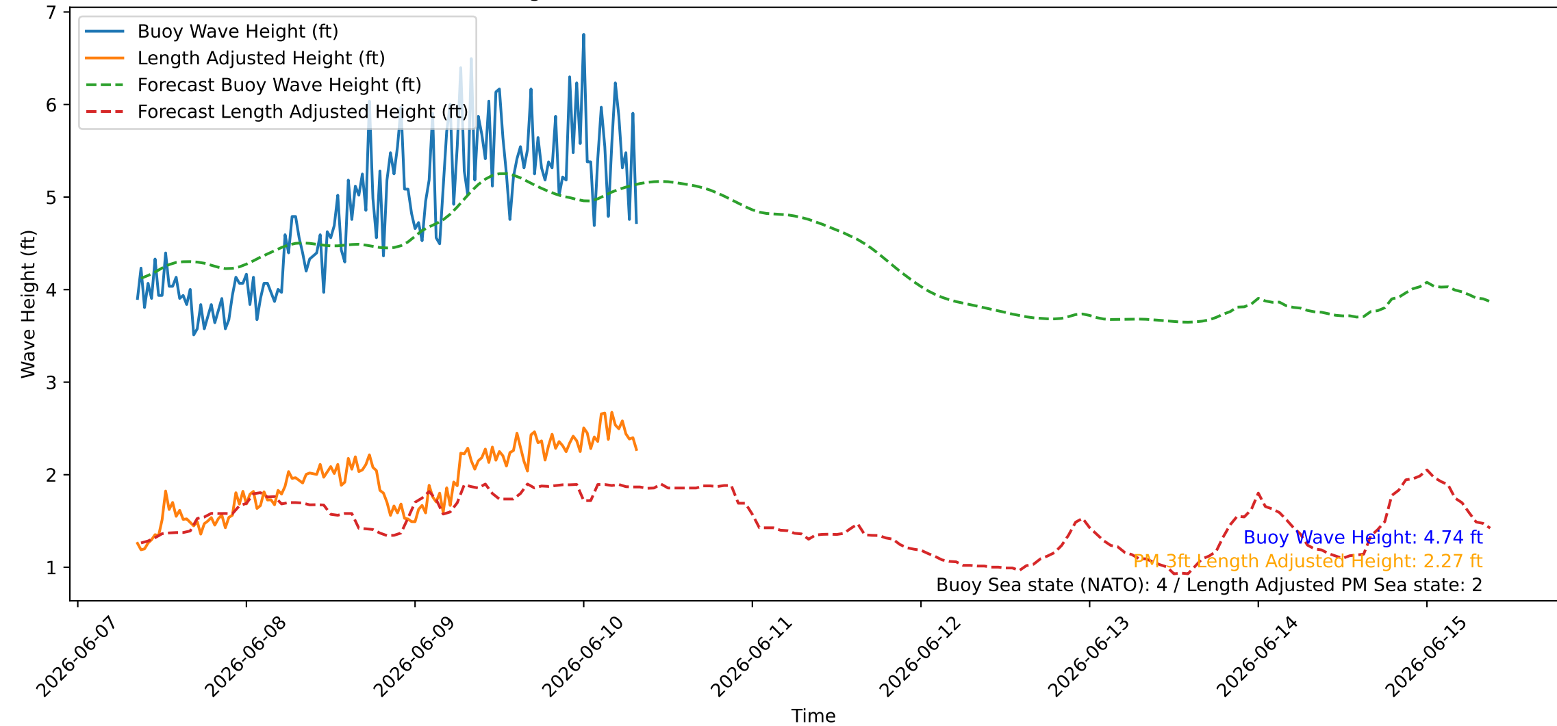
Wave Heights over Time for Oceanside Harbor at 2026-06-10 08:30:26
