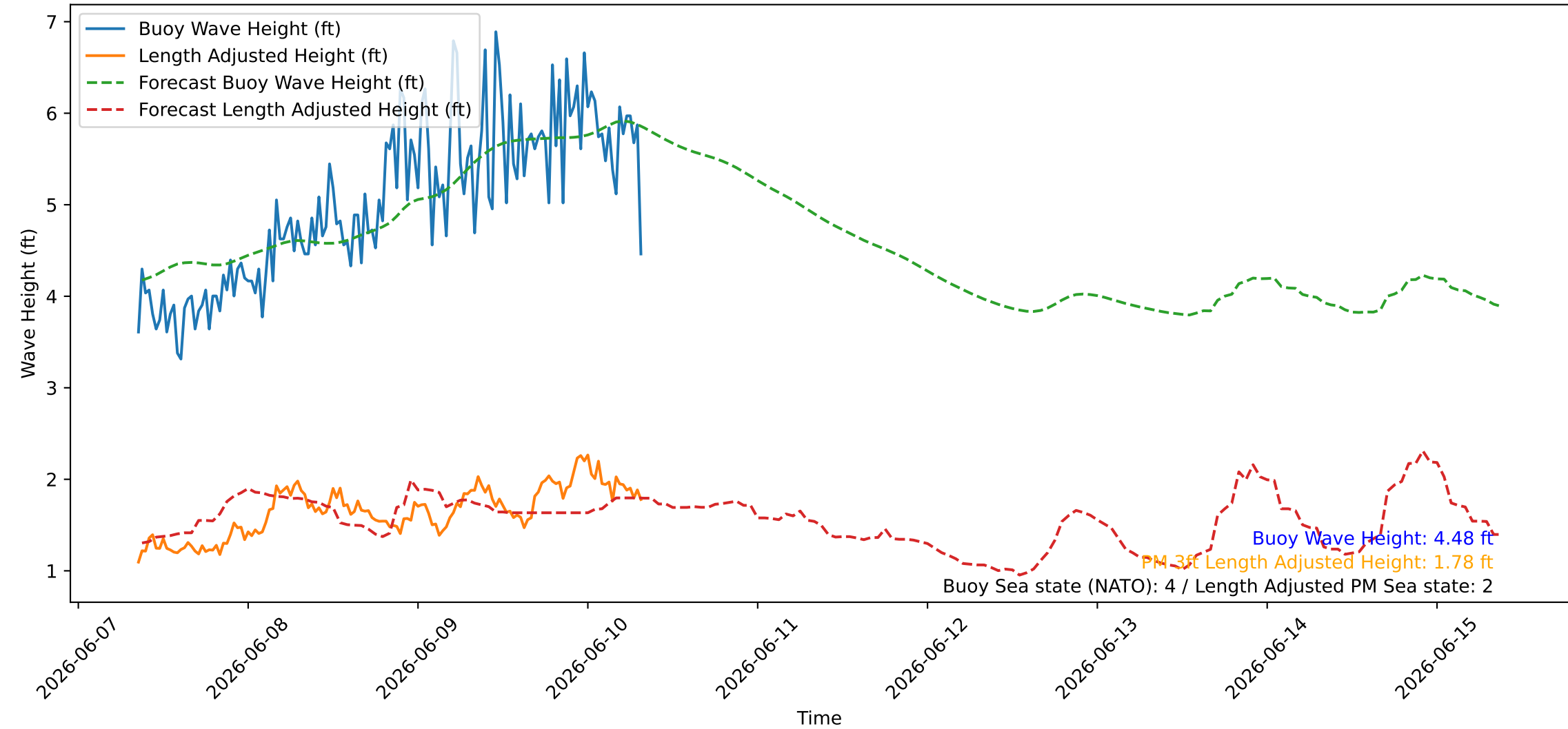
Wave Heights over Time for Green Beach at 2026-06-10 08:31:09
