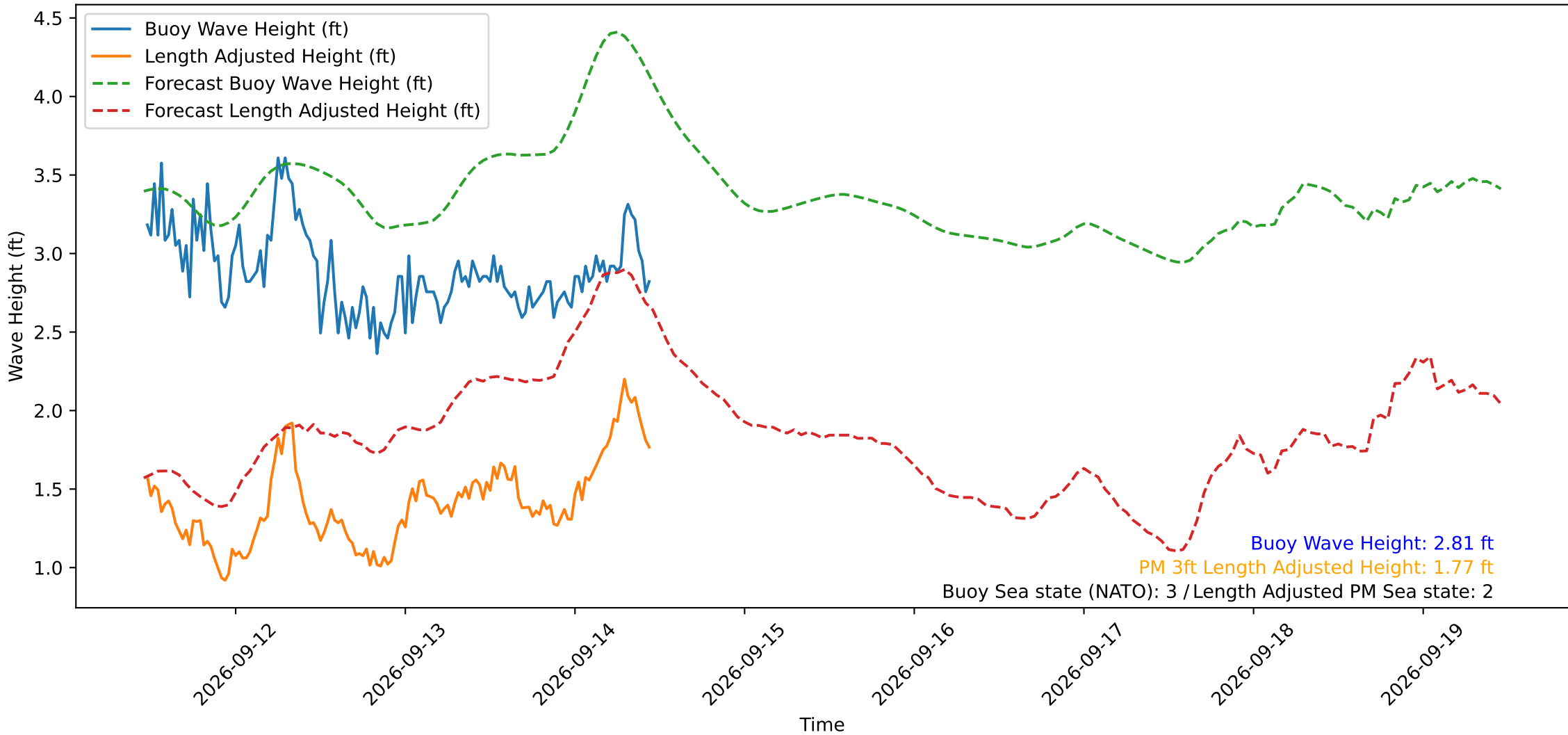
Wave Heights over Time for Green Beach at 2026-09-14 11:21:13
