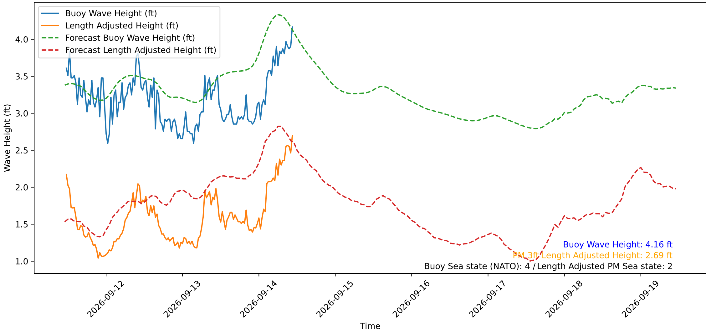
Wave Heights over Time for Oceanside Harbor at 2026-09-14 11:20:29
