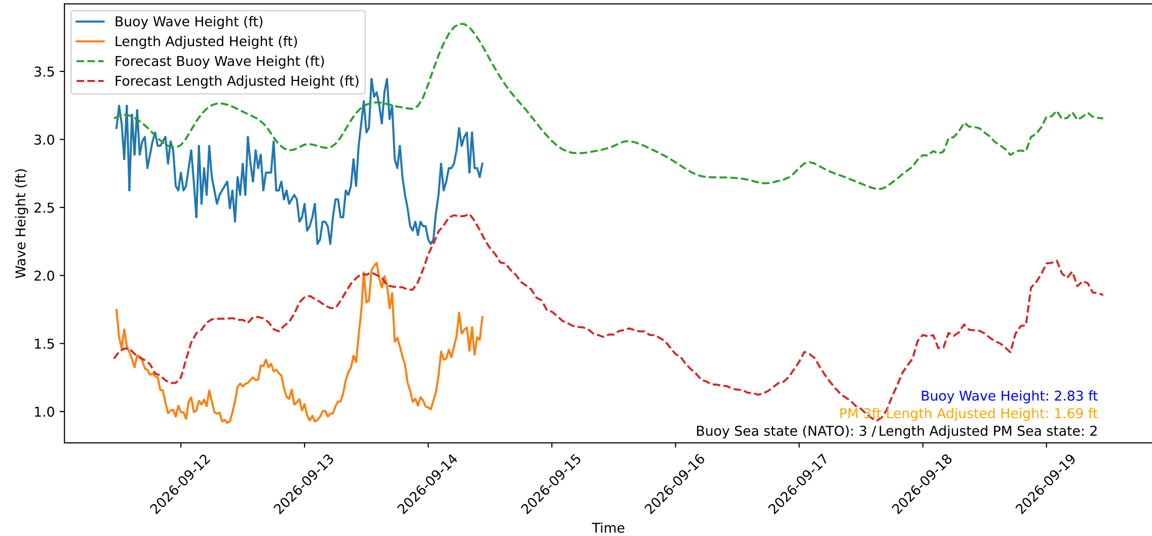
Wave Heights over Time for Red Beach at 2026-09-14 11:20:49
