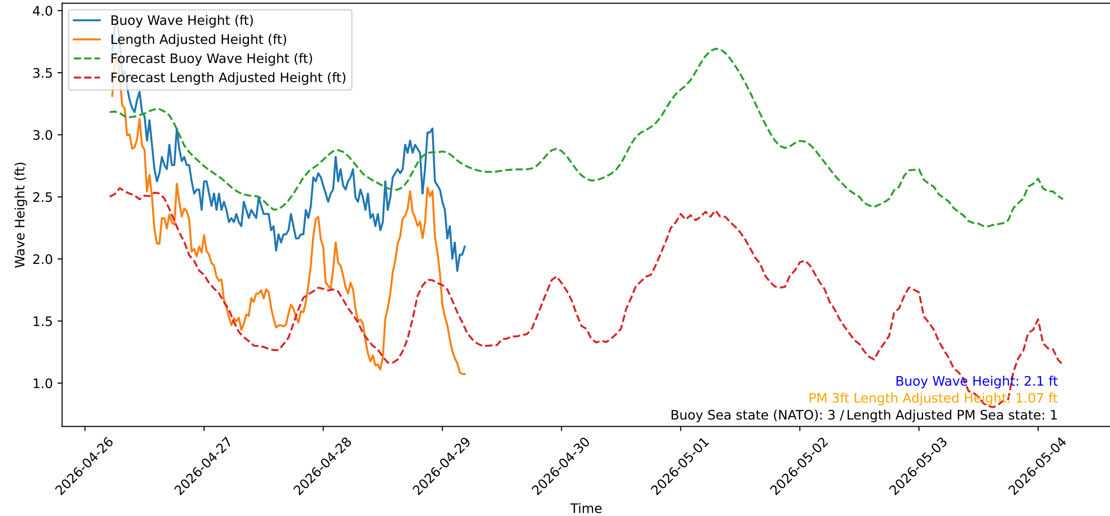
Wave Heights over Time for Oceanside Harbor at 2026-04-29 05:20:31
