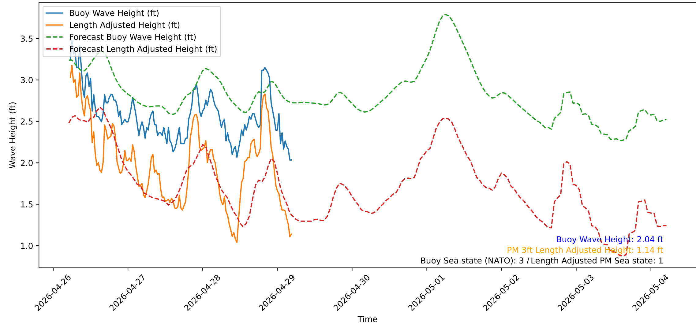
Wave Heights over Time for Green Beach at 2026-04-29 05:21:15
