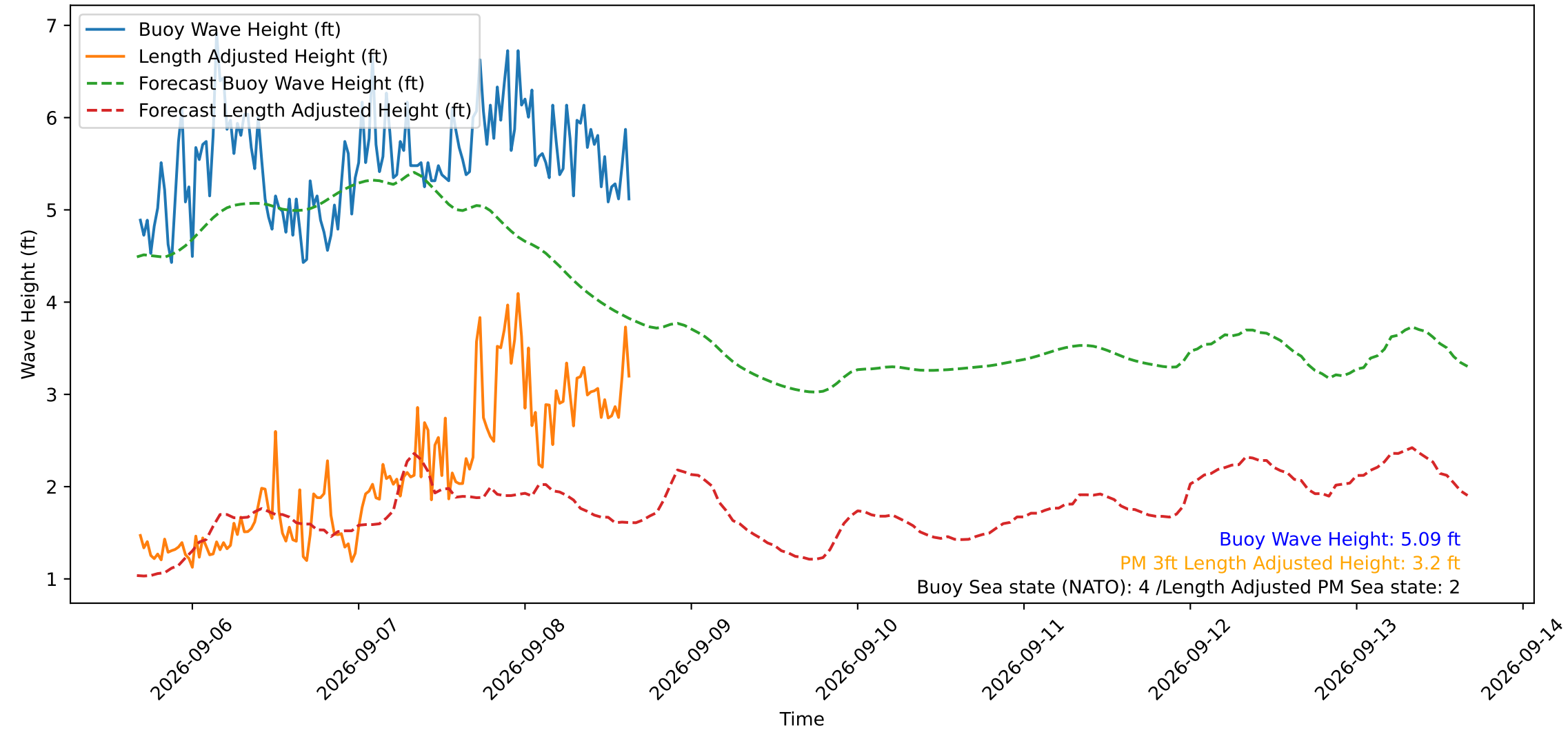
Wave Heights over Time for Red Beach at 2026-09-08 16:00:50
