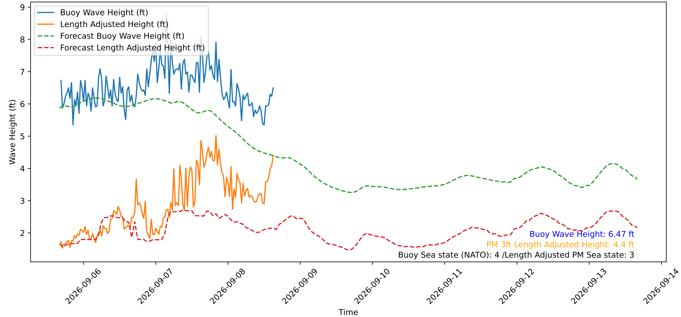
Wave Heights over Time for Green Beach at 2026-09-08 16:01:12
