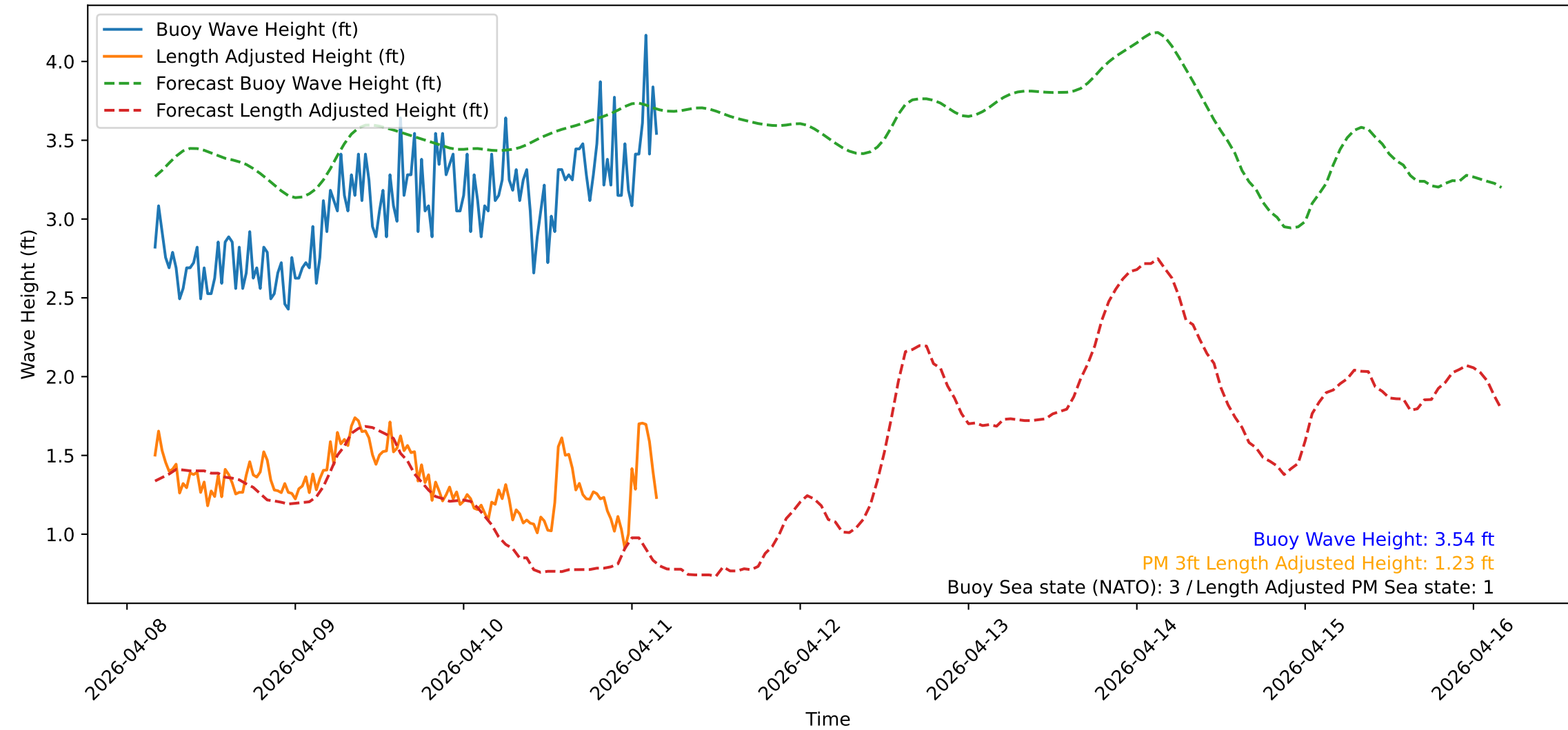
Wave Heights over Time for Oceanside Harbor at 2026-04-11 04:00:32
