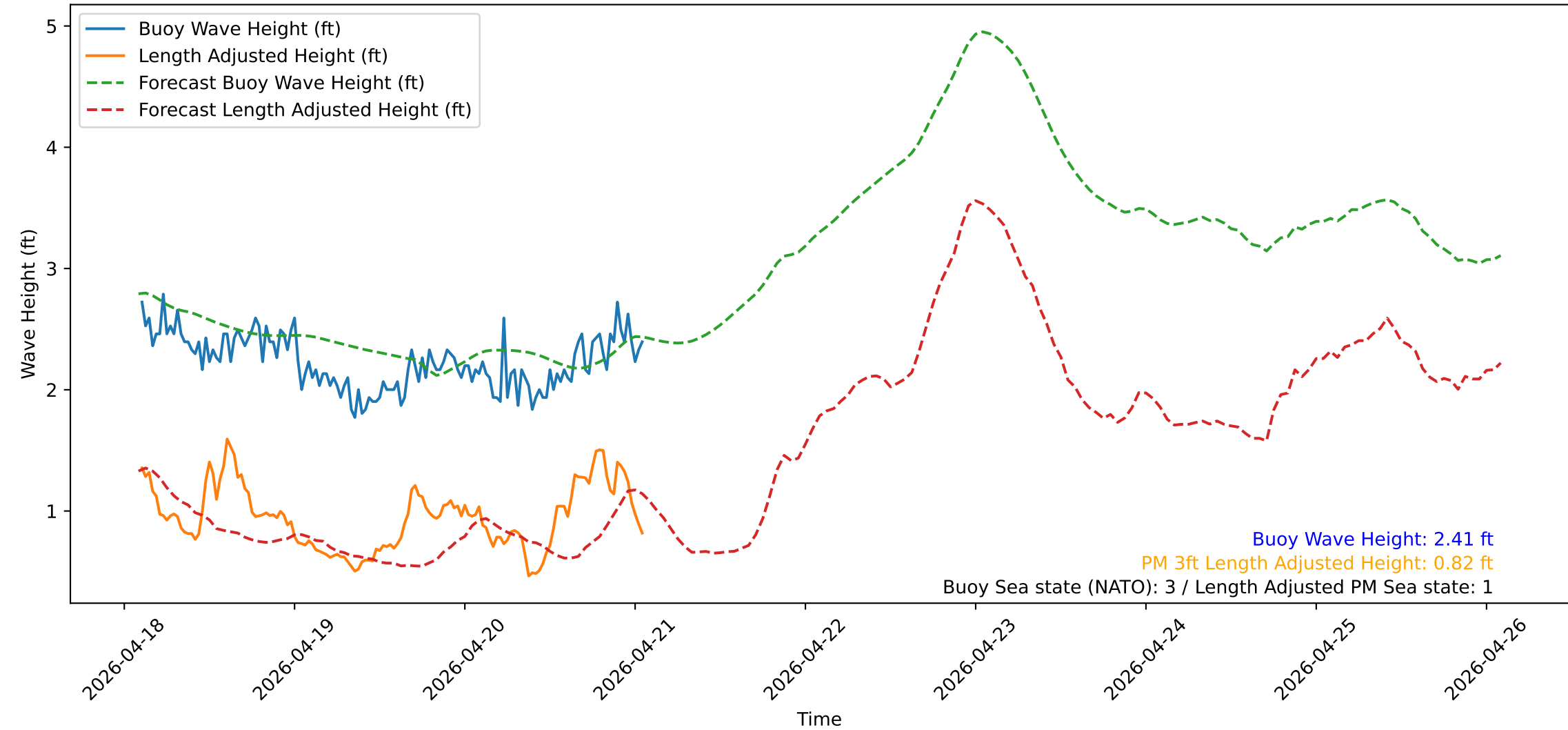
Wave Heights over Time for Red Beach at 2026-04-21 02:00:50
