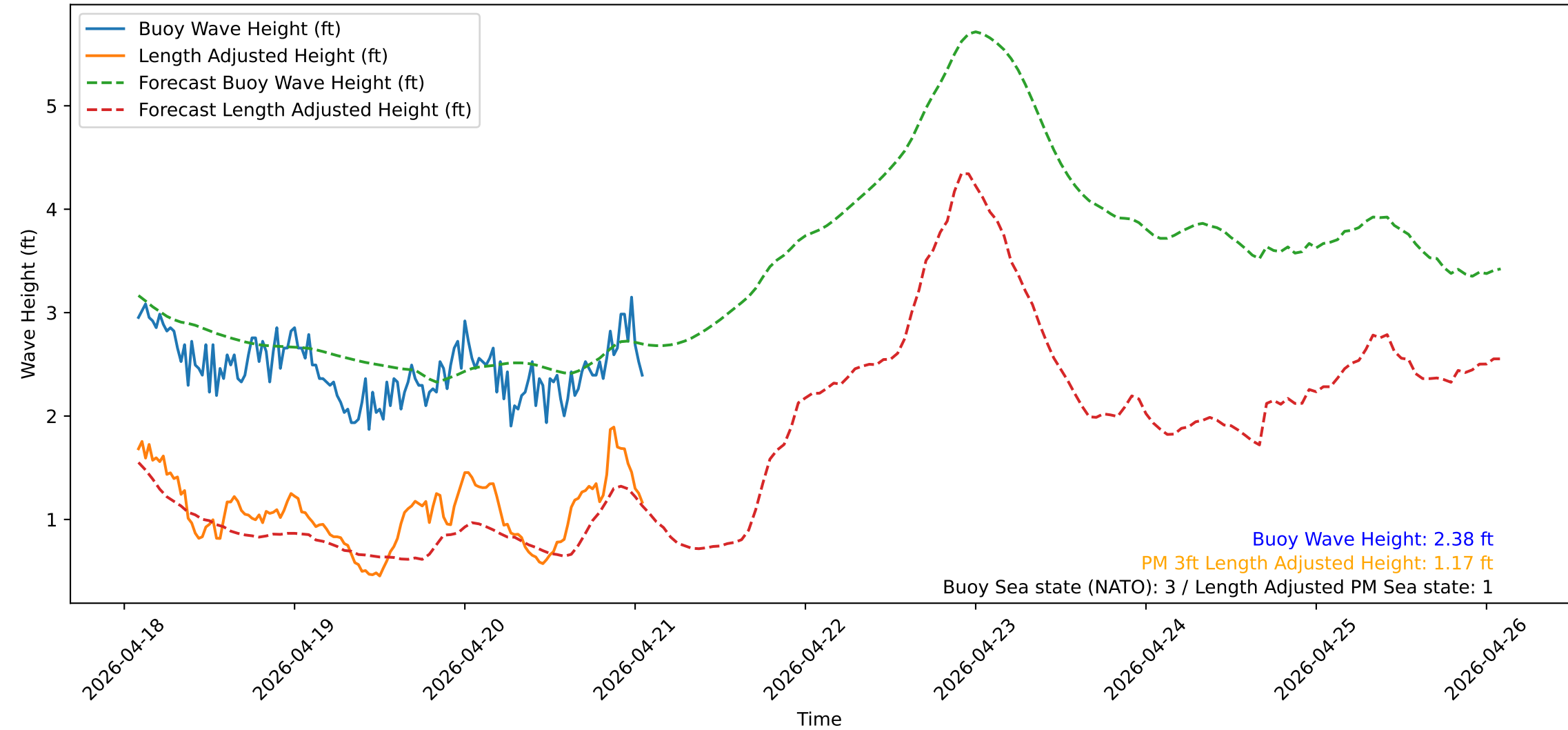
Wave Heights over Time for Green Beach at 2026-04-21 02:01:12
