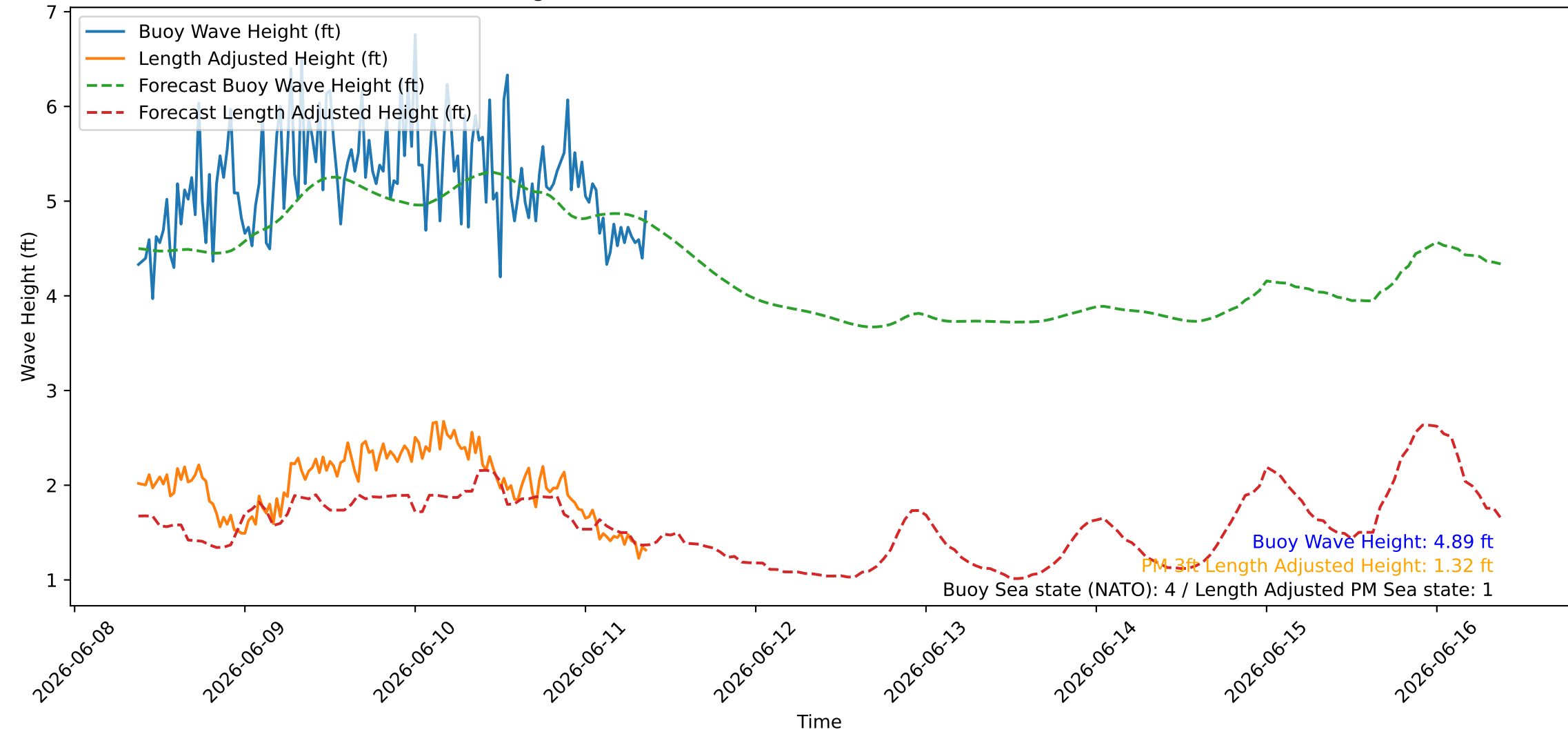
Wave Heights over Time for Oceanside Harbor at 2026-06-11 09:10:27
