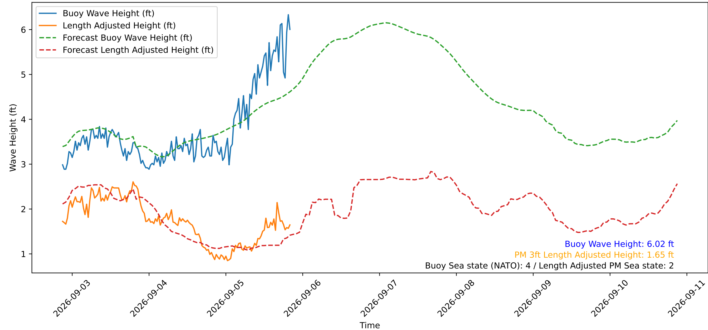
Wave Heights over Time for Oceanside Harbor at 2026-09-05 21:00:29
