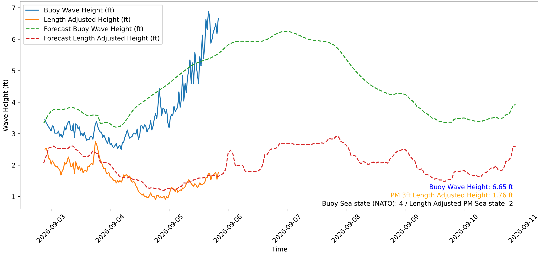
Wave Heights over Time for Green Beach at 2026-09-05 21:01:12
