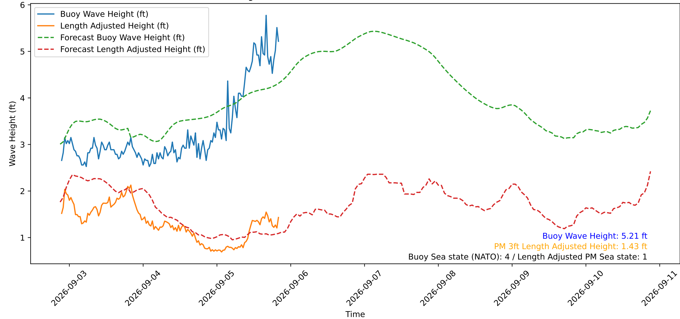
Wave Heights over Time for Red Beach at 2026-09-05 21:00:49
