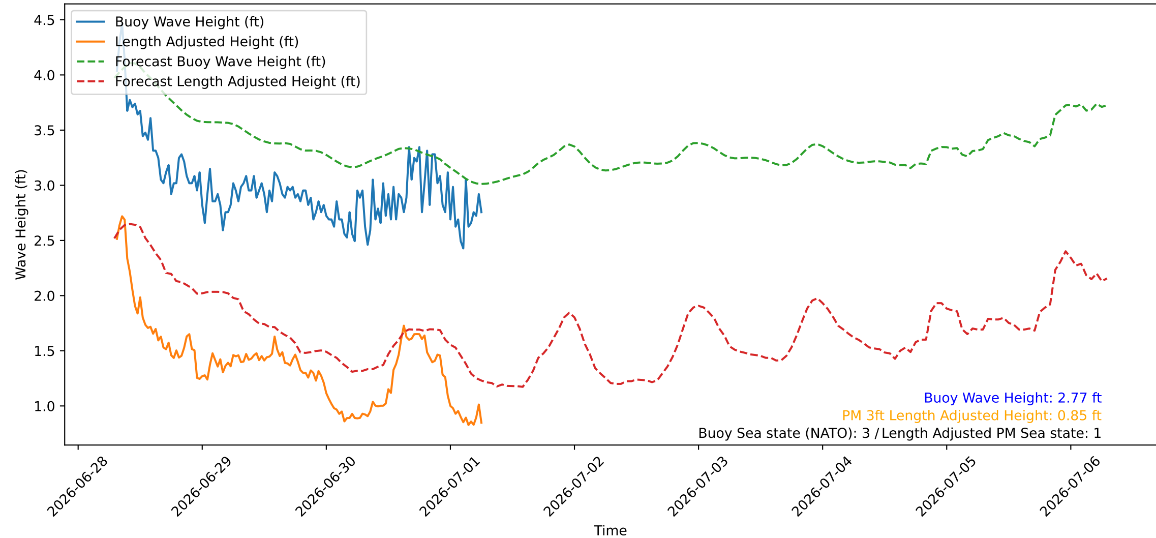
Wave Heights over Time for Red Beach at 2026-07-01 07:00:46
