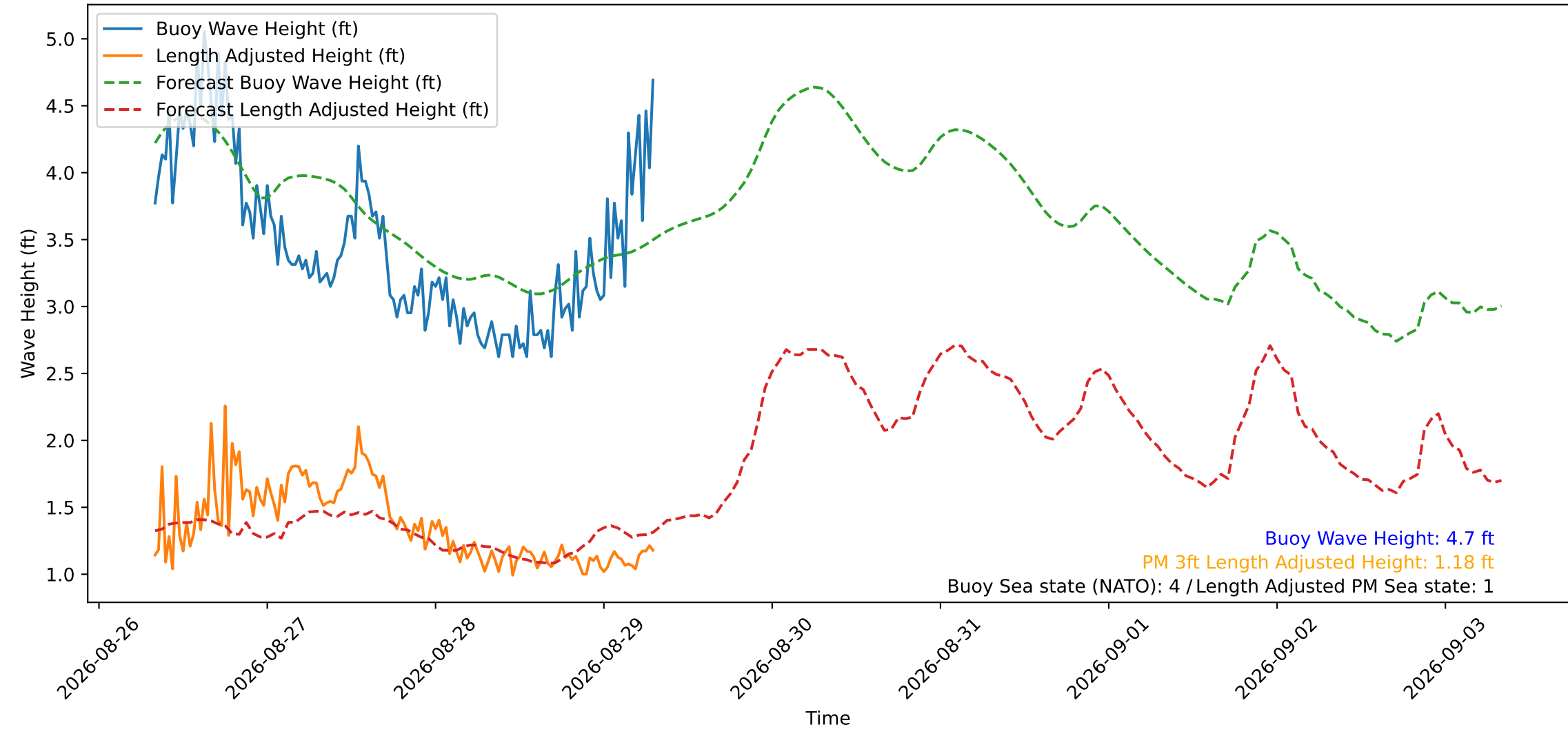
Wave Heights over Time for Red Beach at 2026-08-29 07:50:51
