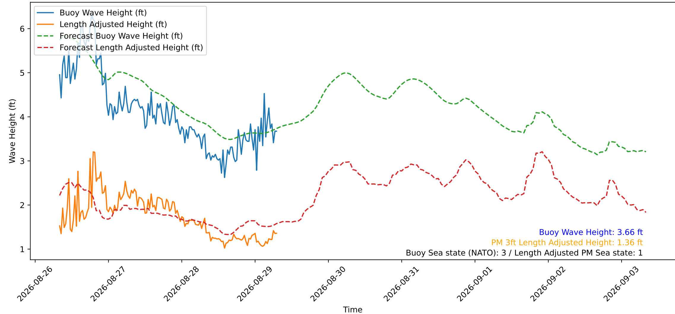
Wave Heights over Time for Green Beach at 2026-08-29 07:51:15
