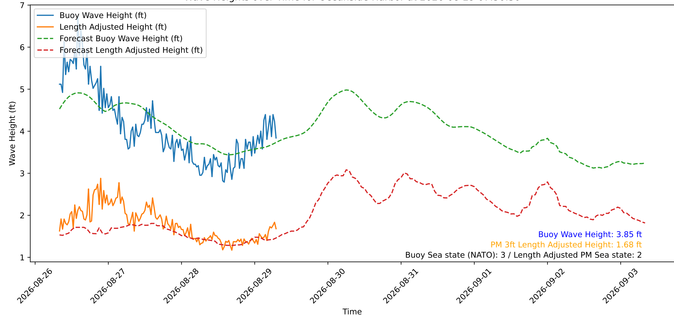
Wave Heights over Time for Oceanside Harbor at 2026-08-29 07:50:30
