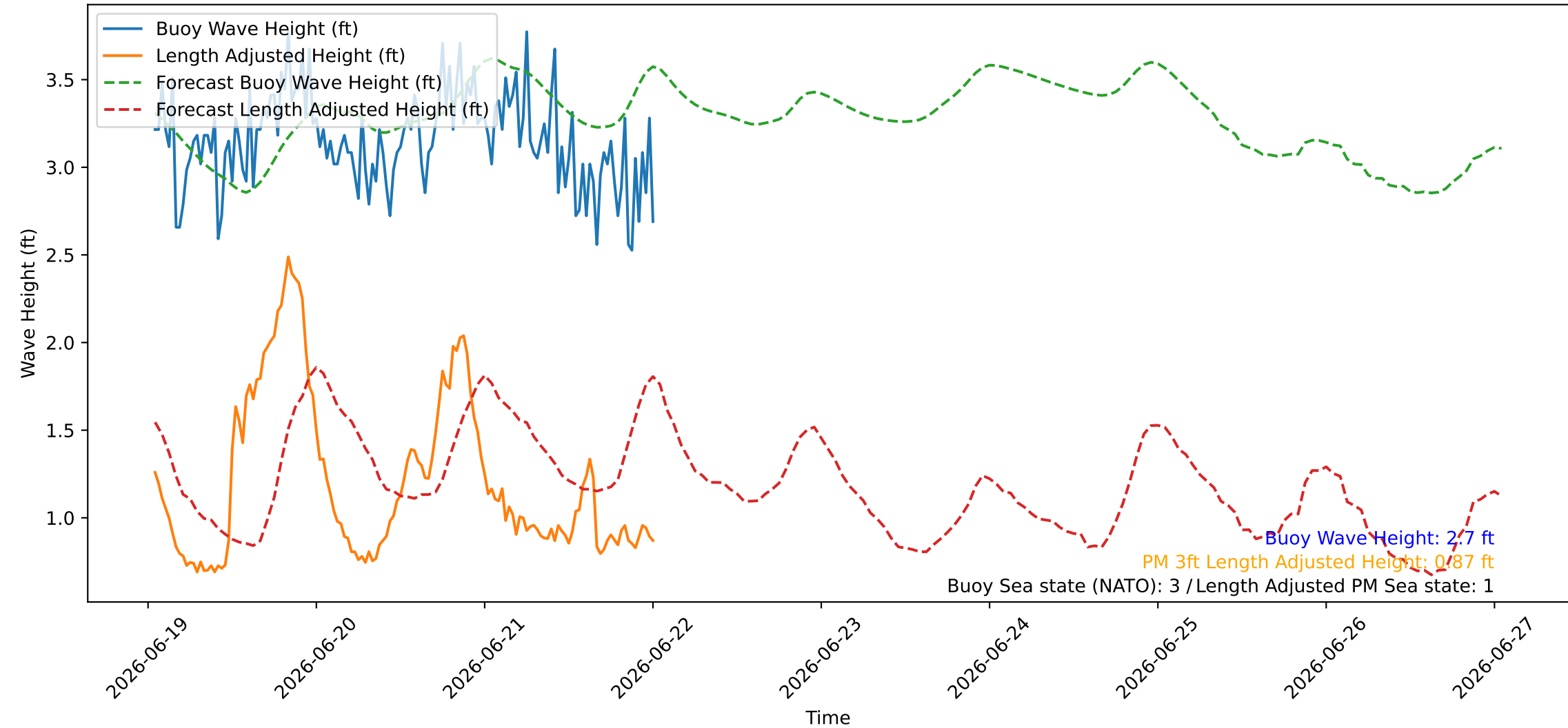
Wave Heights over Time for Red Beach at 2026-06-22 00:50:47
