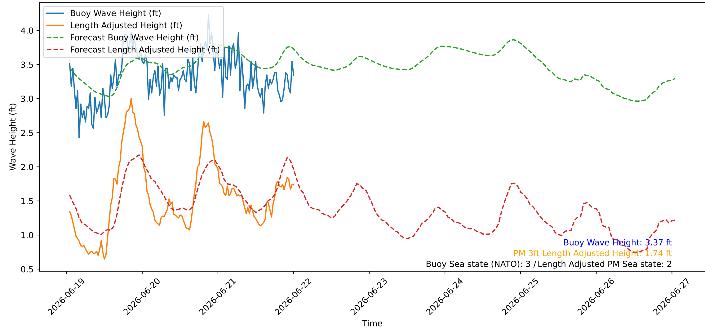
Wave Heights over Time for Green Beach at 2026-06-22 00:51:09
