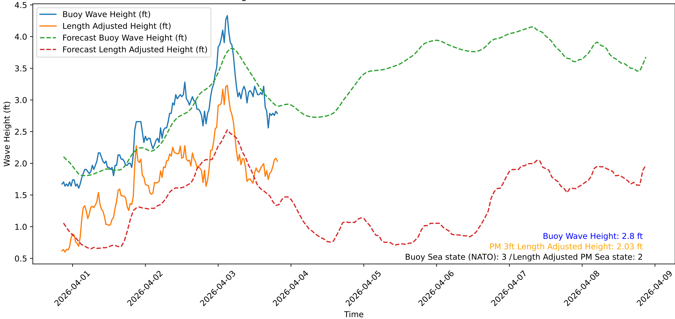
Wave Heights over Time for Green Beach at 2026-04-03 20:31:30
