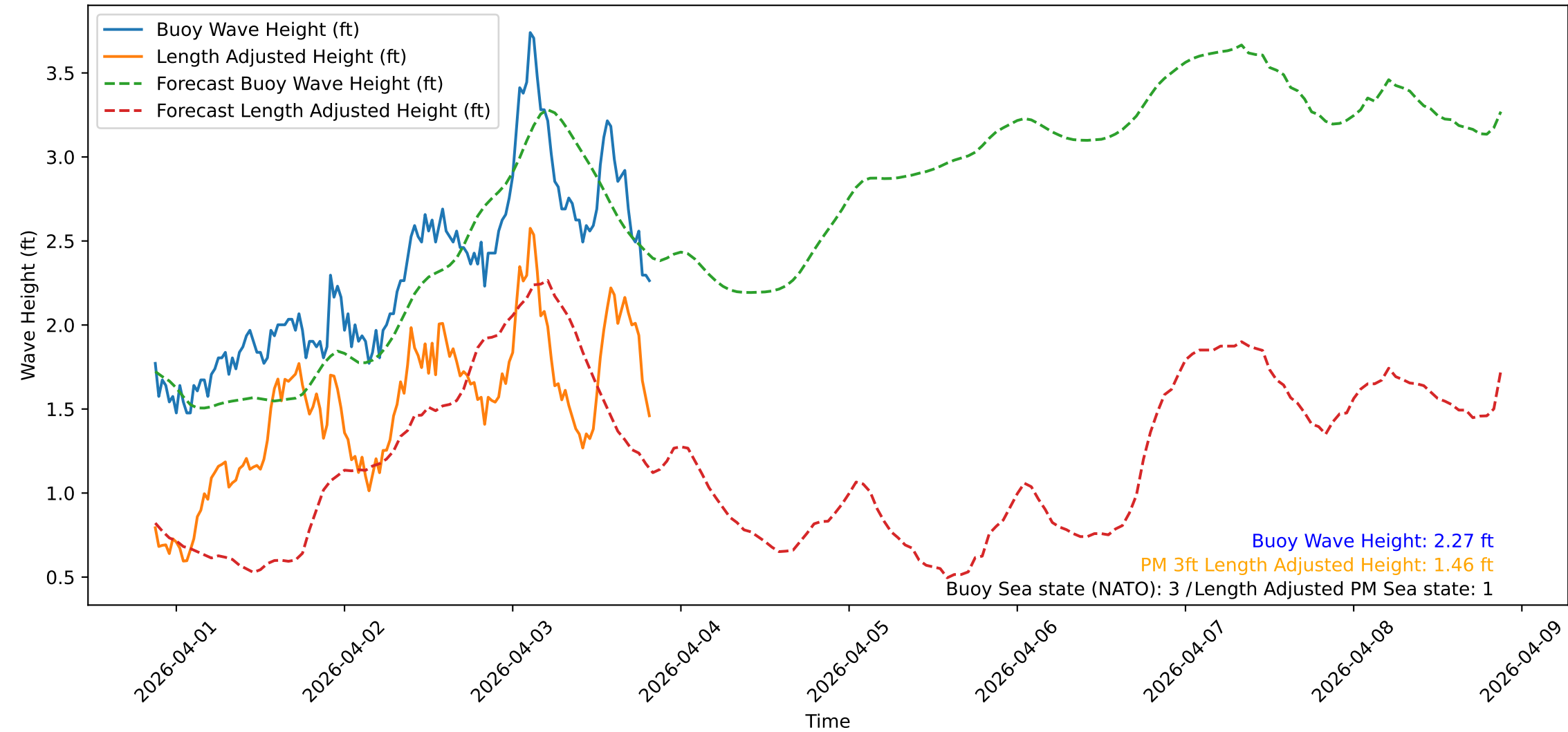
Wave Heights over Time for Red Beach at 2026-04-03 20:31:01
