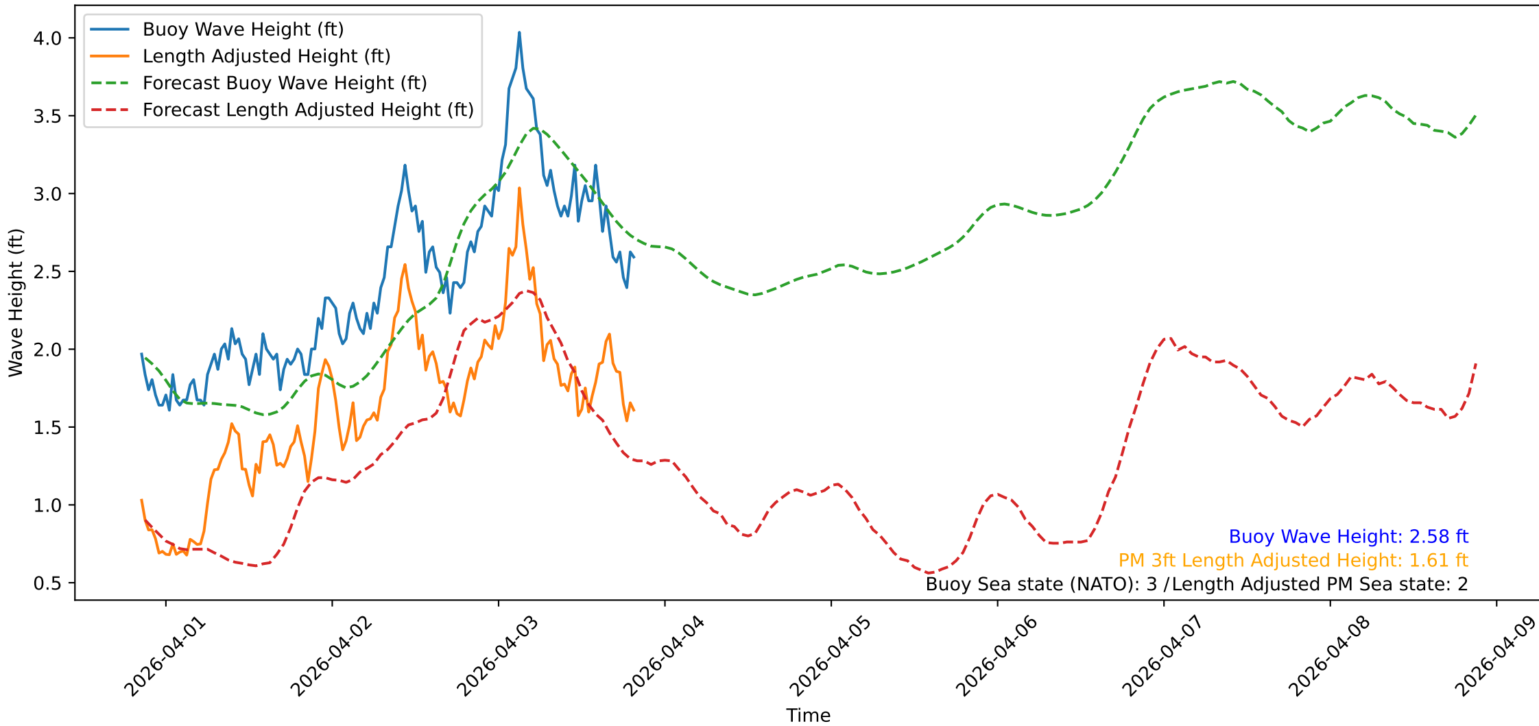
Wave Heights over Time for Oceanside Harbor at 2026-04-03 20:30:38
