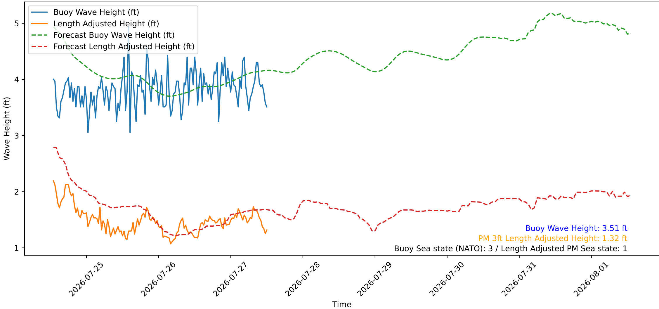
Wave Heights over Time for Oceanside Harbor at 2026-07-27 12:50:26
