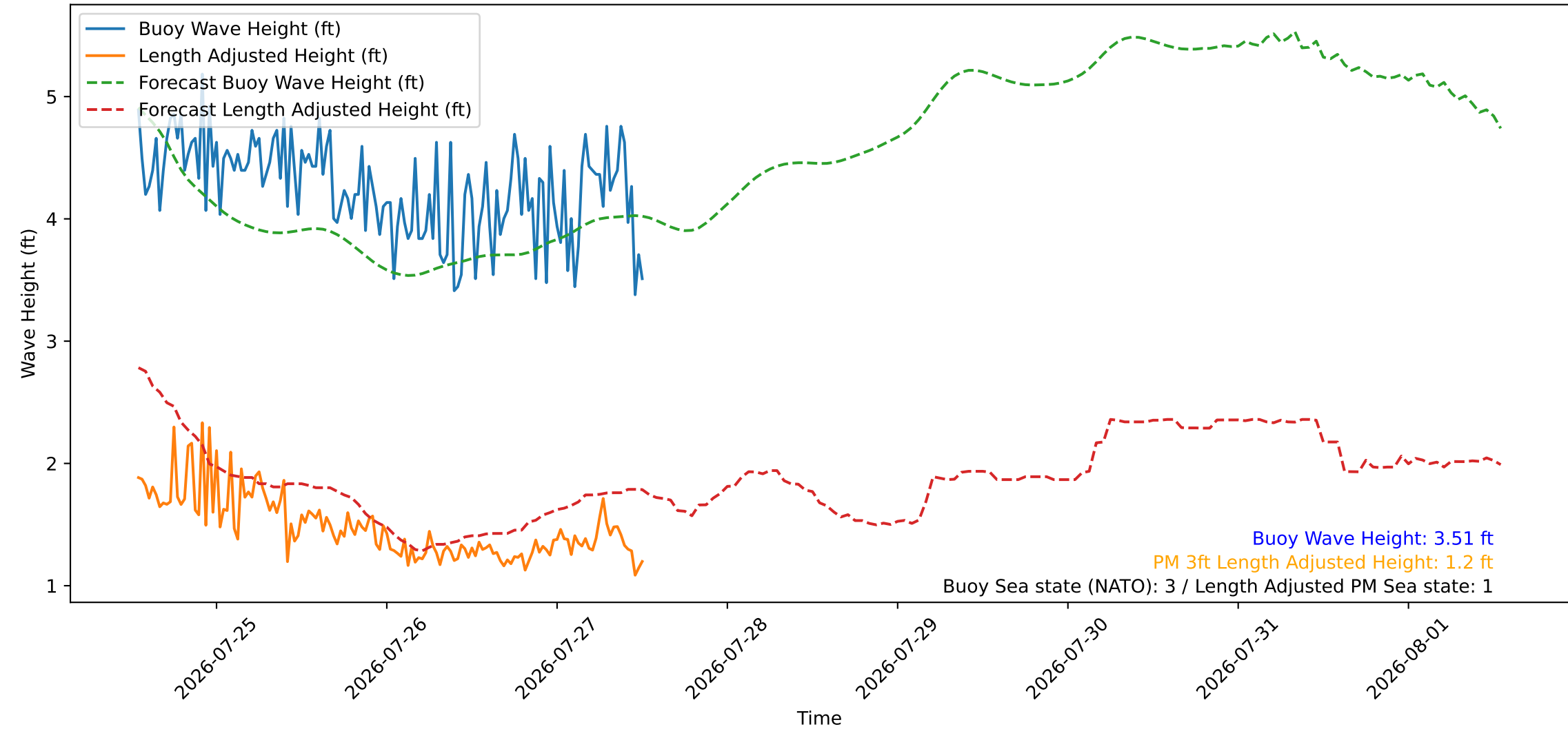
Wave Heights over Time for Green Beach at 2026-07-27 12:51:09
