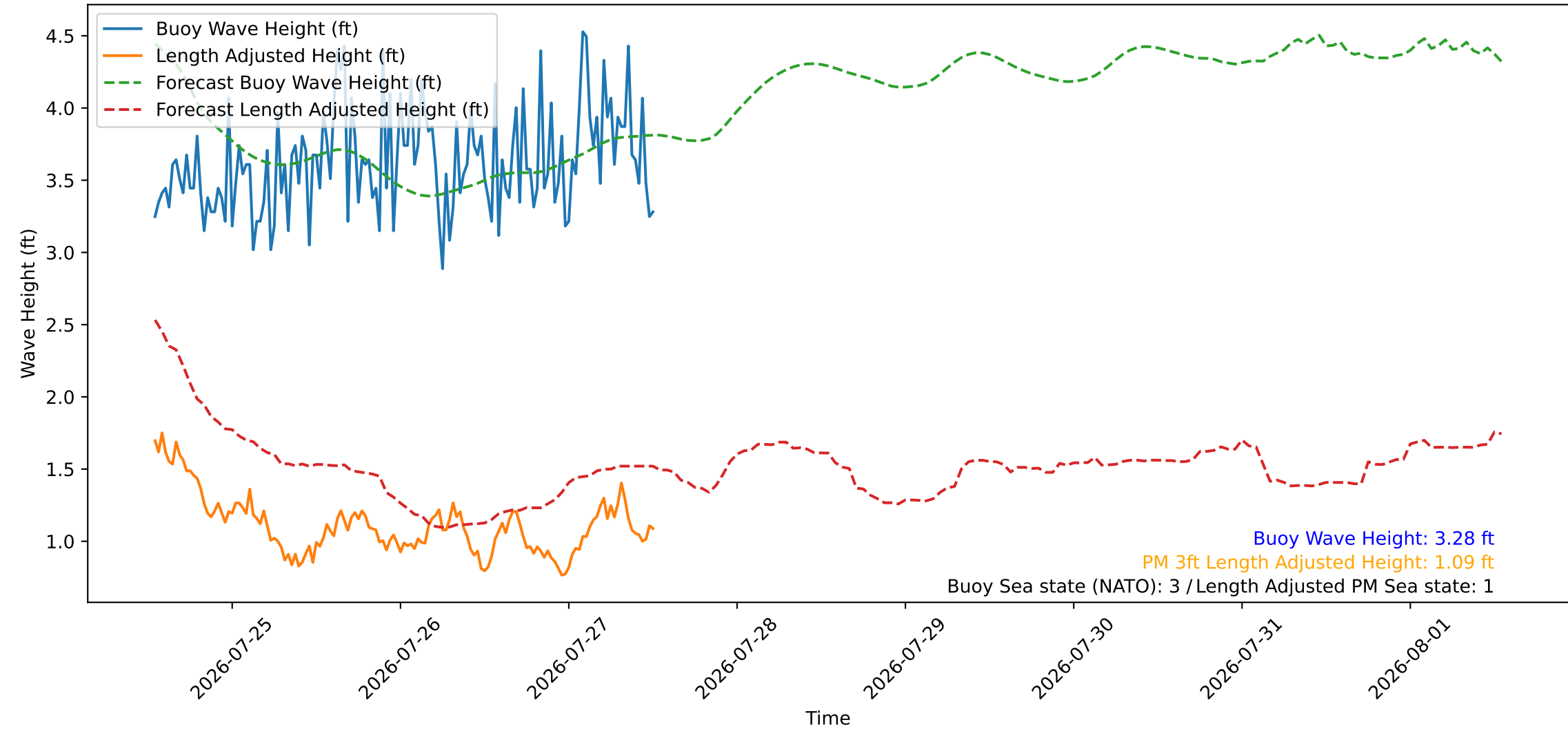
Wave Heights over Time for Red Beach at 2026-07-27 12:50:47
