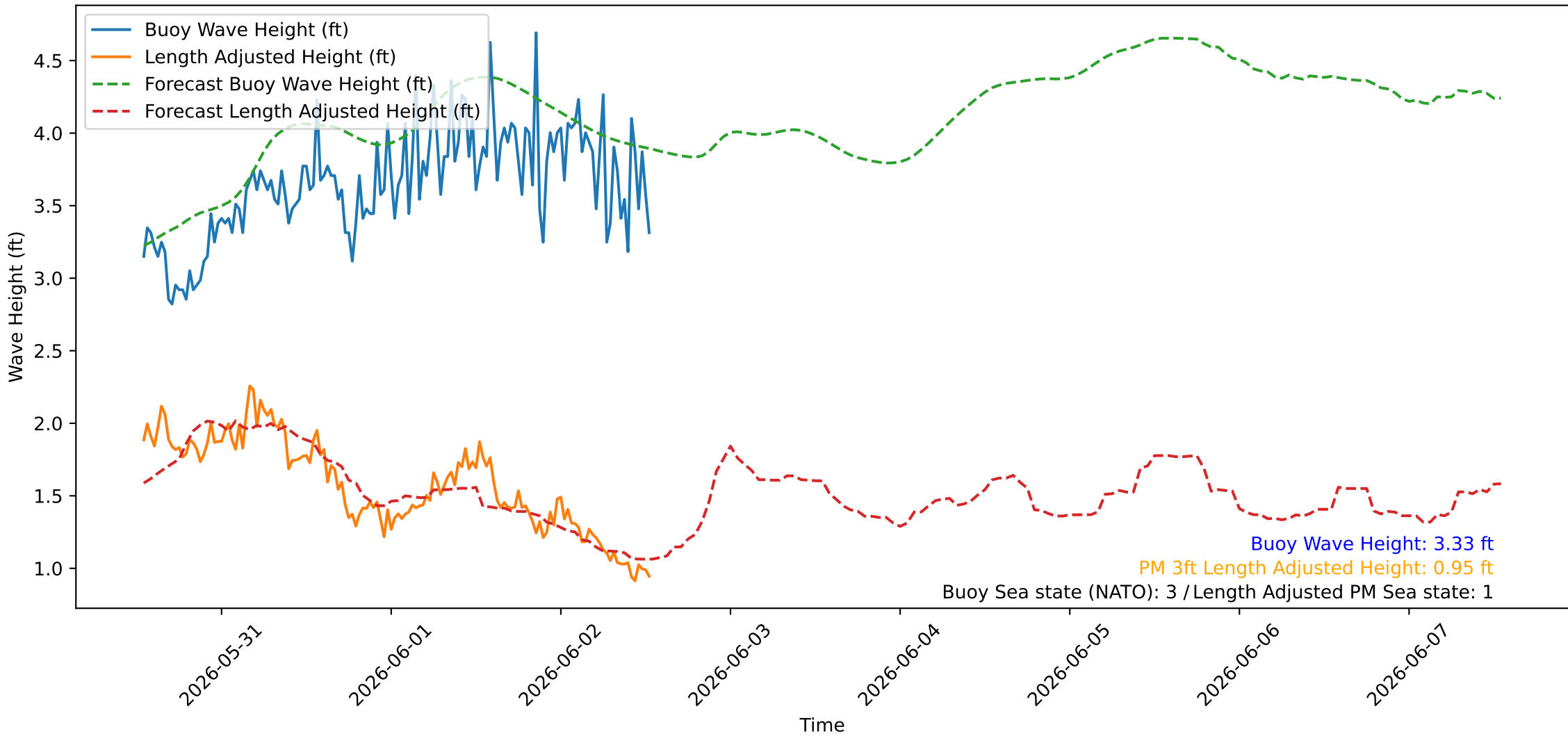
Wave Heights over Time for Oceanside Harbor at 2026-06-02 13:10:25
