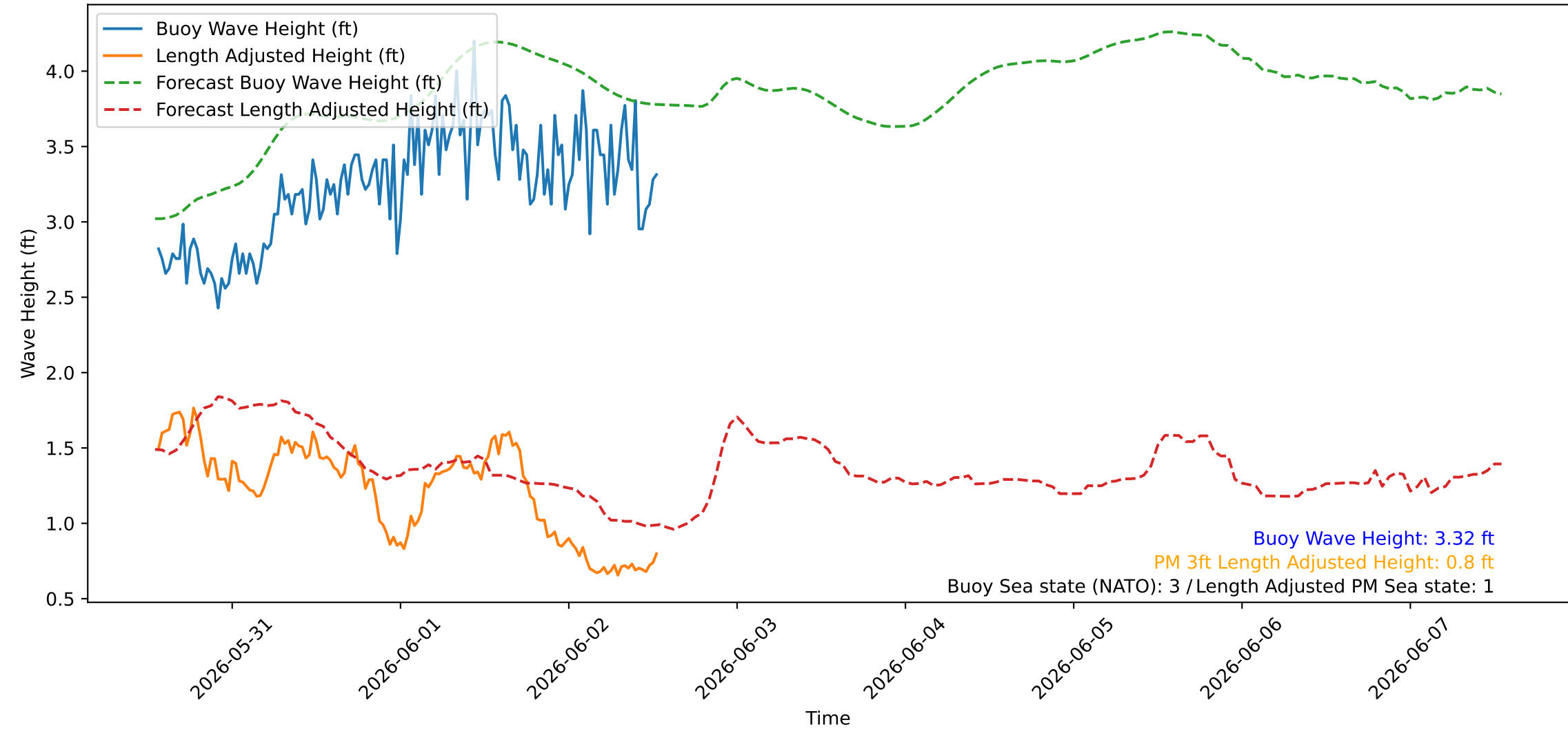
Wave Heights over Time for Red Beach at 2026-06-02 13:10:44
