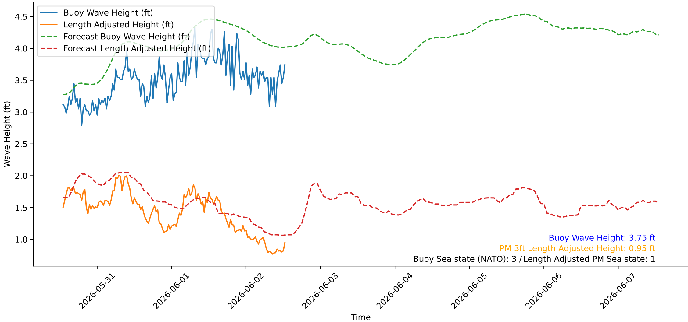
Wave Heights over Time for Green Beach at 2026-06-02 13:11:07
