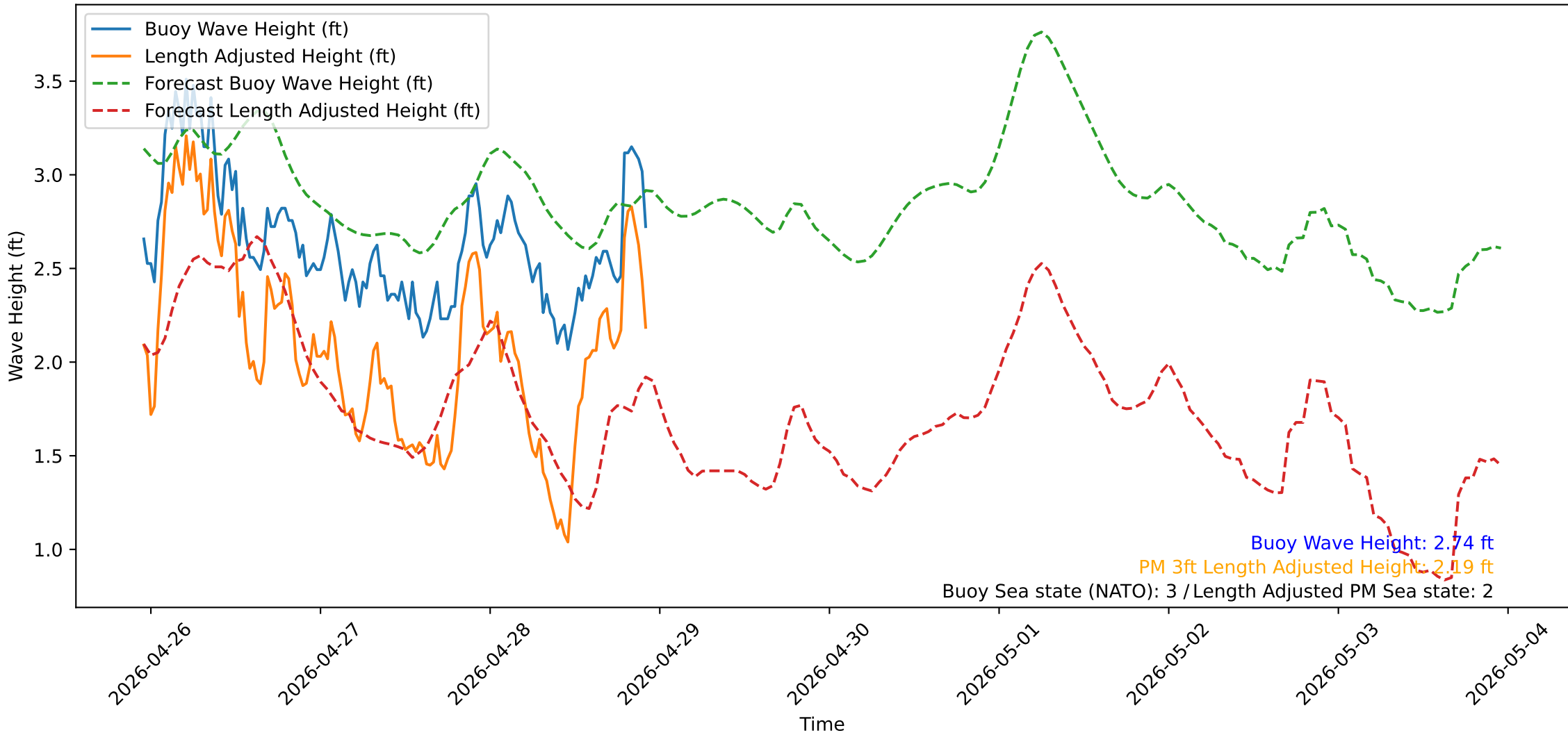
Wave Heights over Time for Green Beach at 2026-04-28 23:01:13
