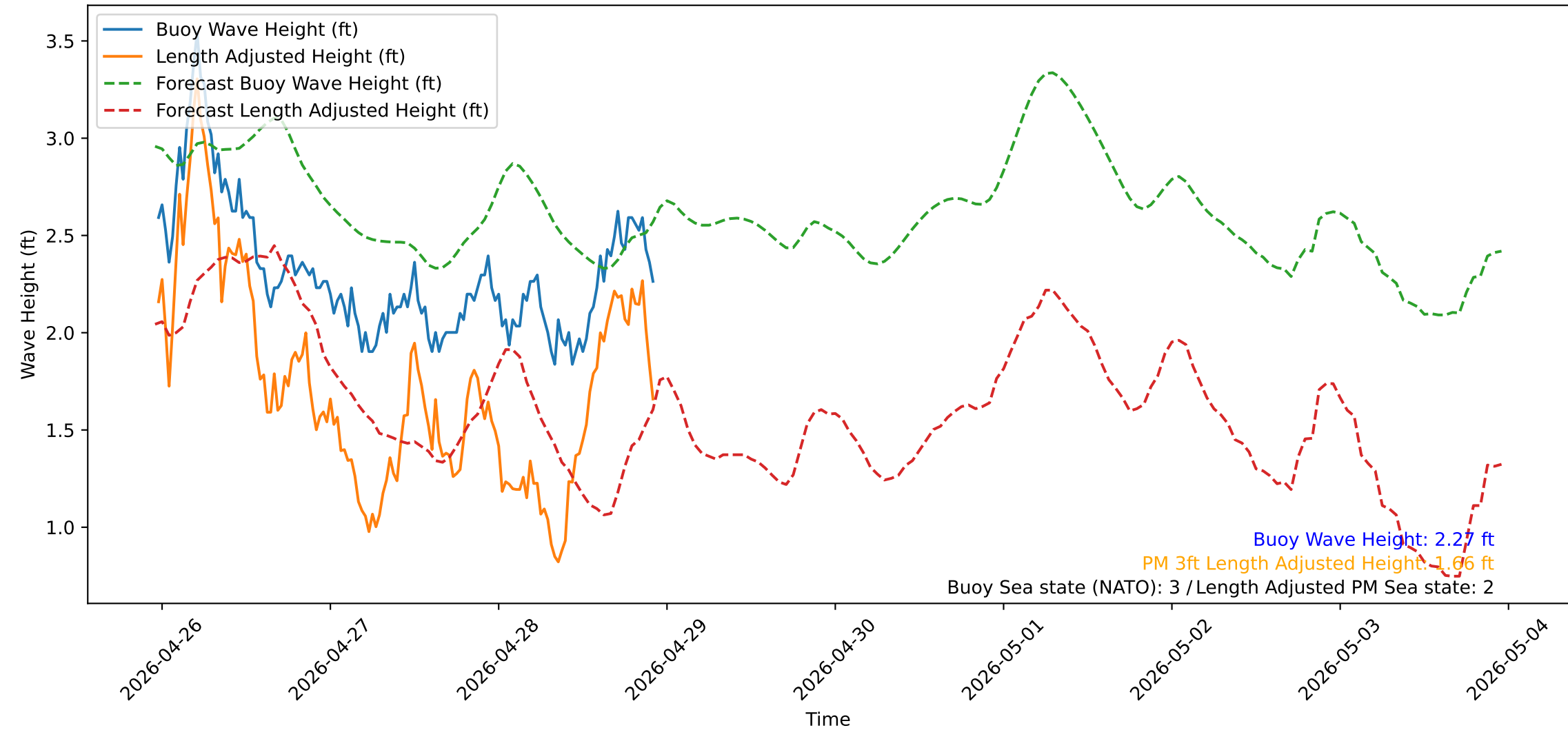
Wave Heights over Time for Red Beach at 2026-04-28 23:00:50
