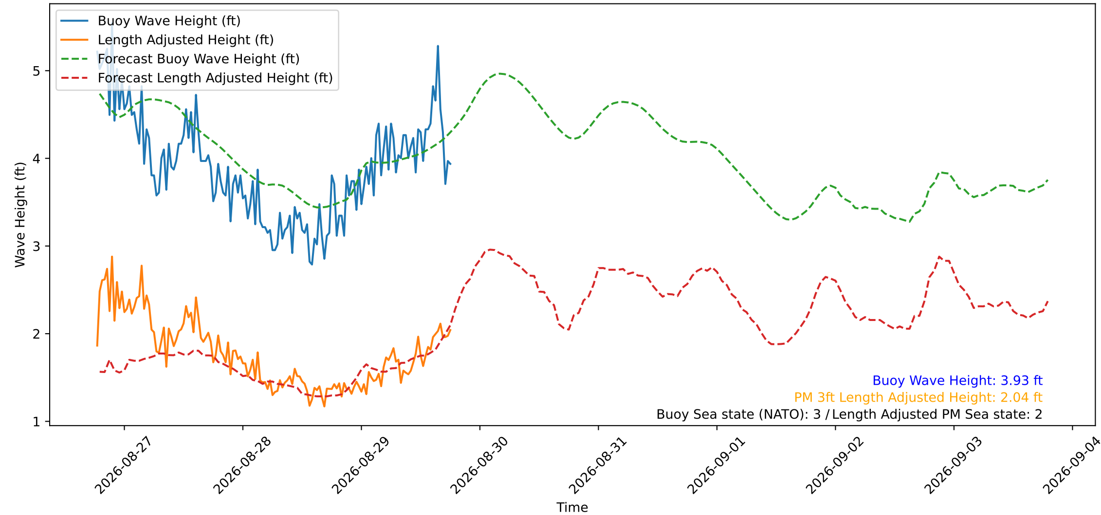
Wave Heights over Time for Oceanside Harbor at 2026-08-29 18:30:30
