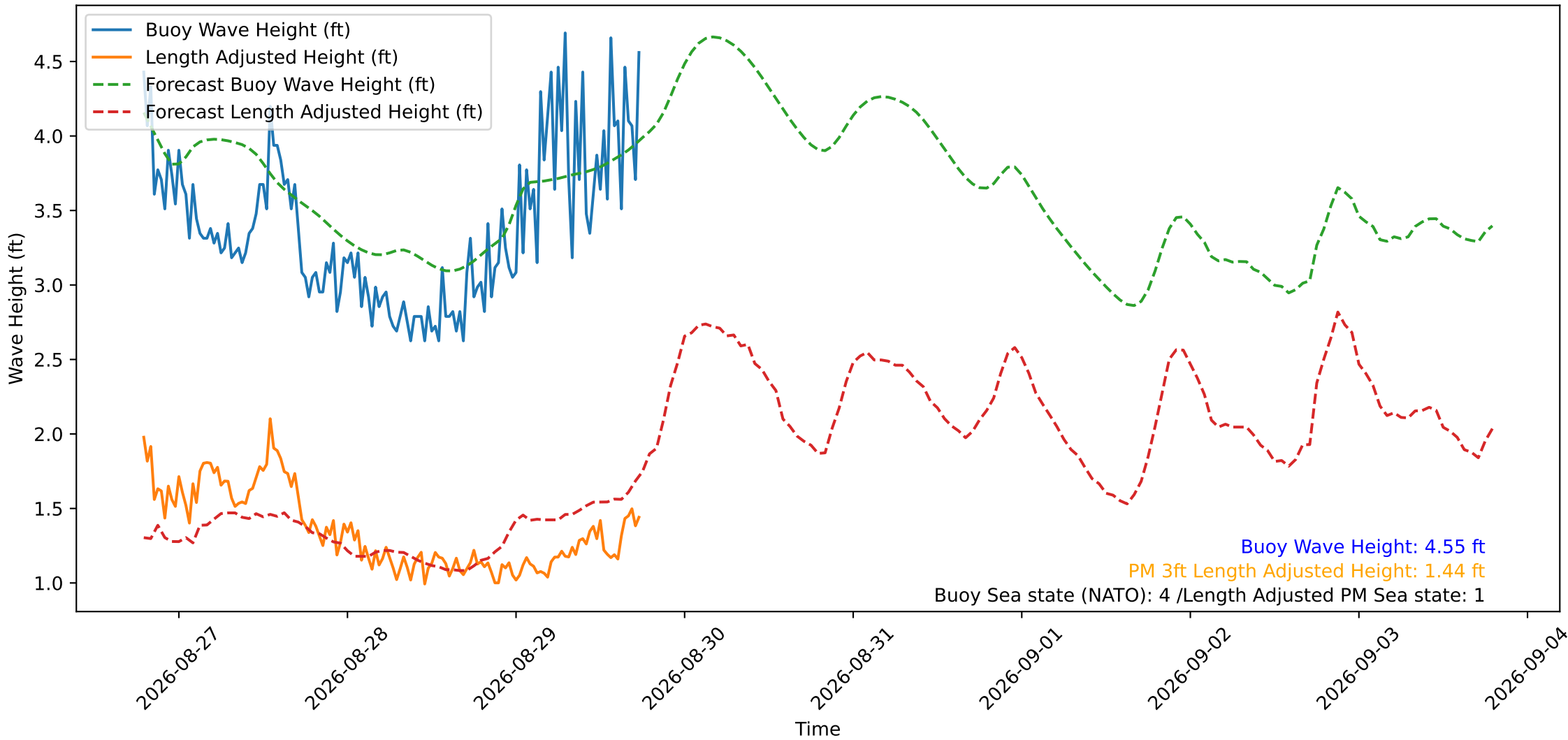
Wave Heights over Time for Red Beach at 2026-08-29 18:30:49
