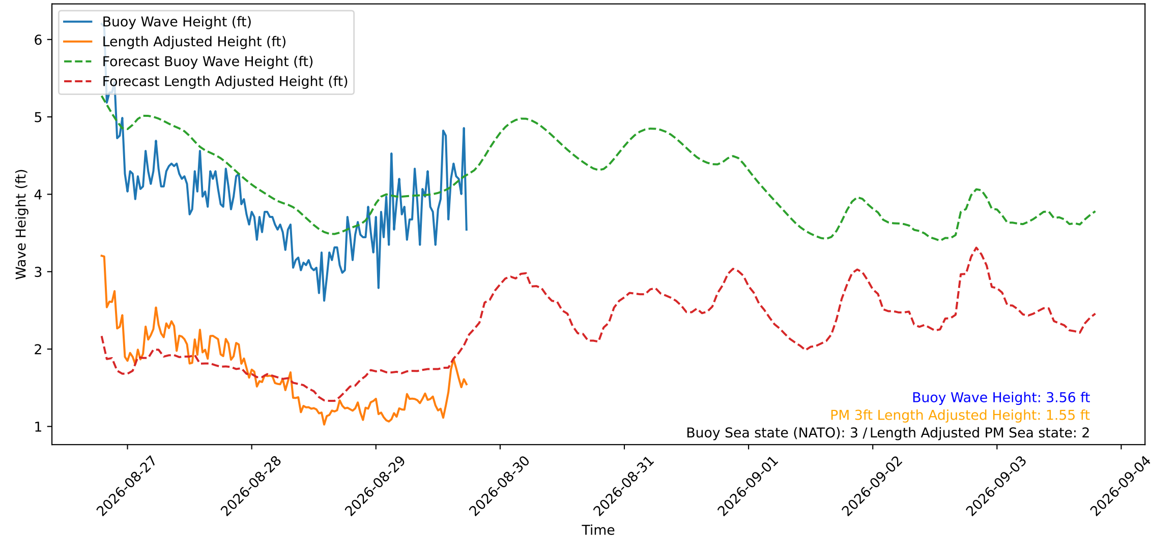
Wave Heights over Time for Green Beach at 2026-08-29 18:31:12
