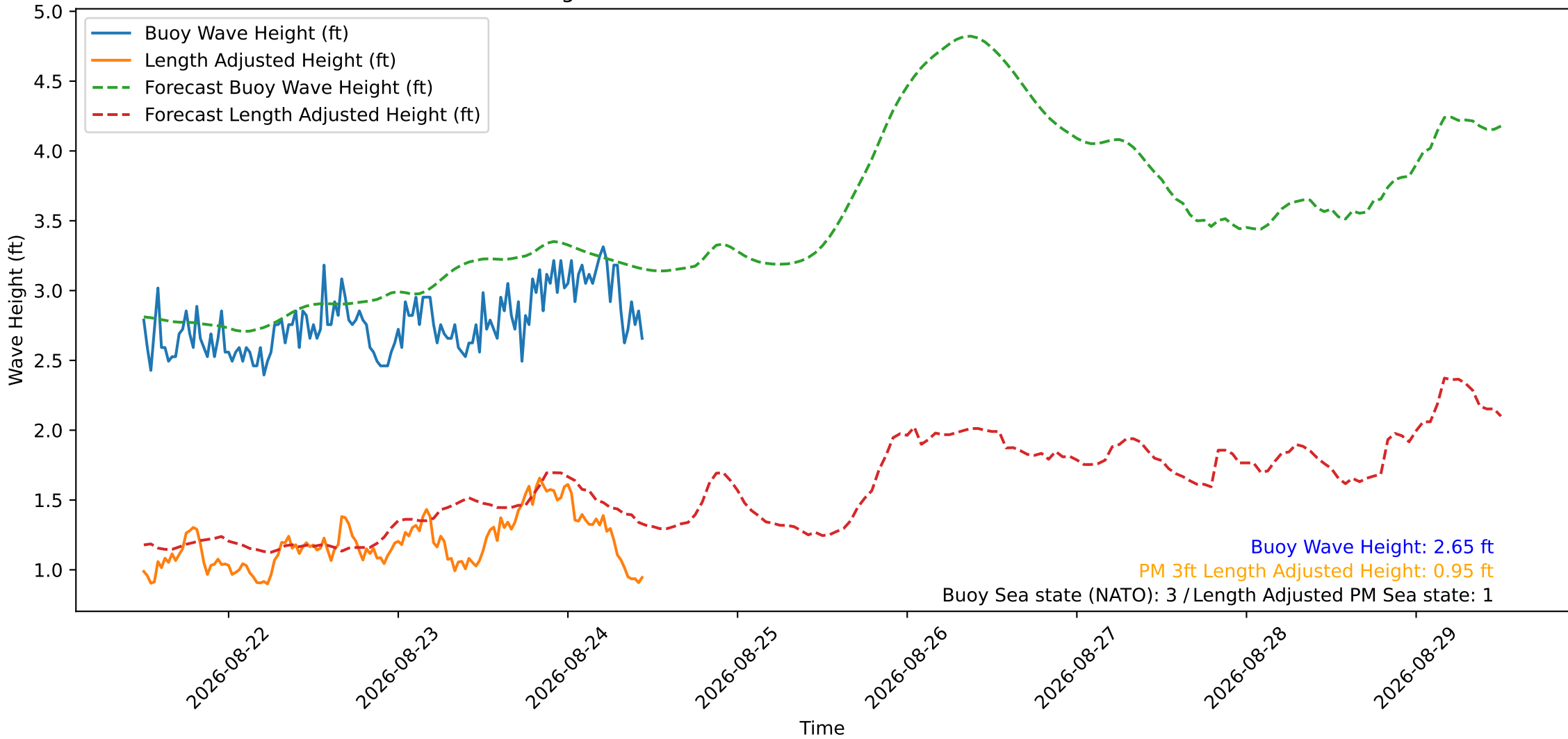
Wave Heights over Time for Green Beach at 2026-08-24 11:31:11
