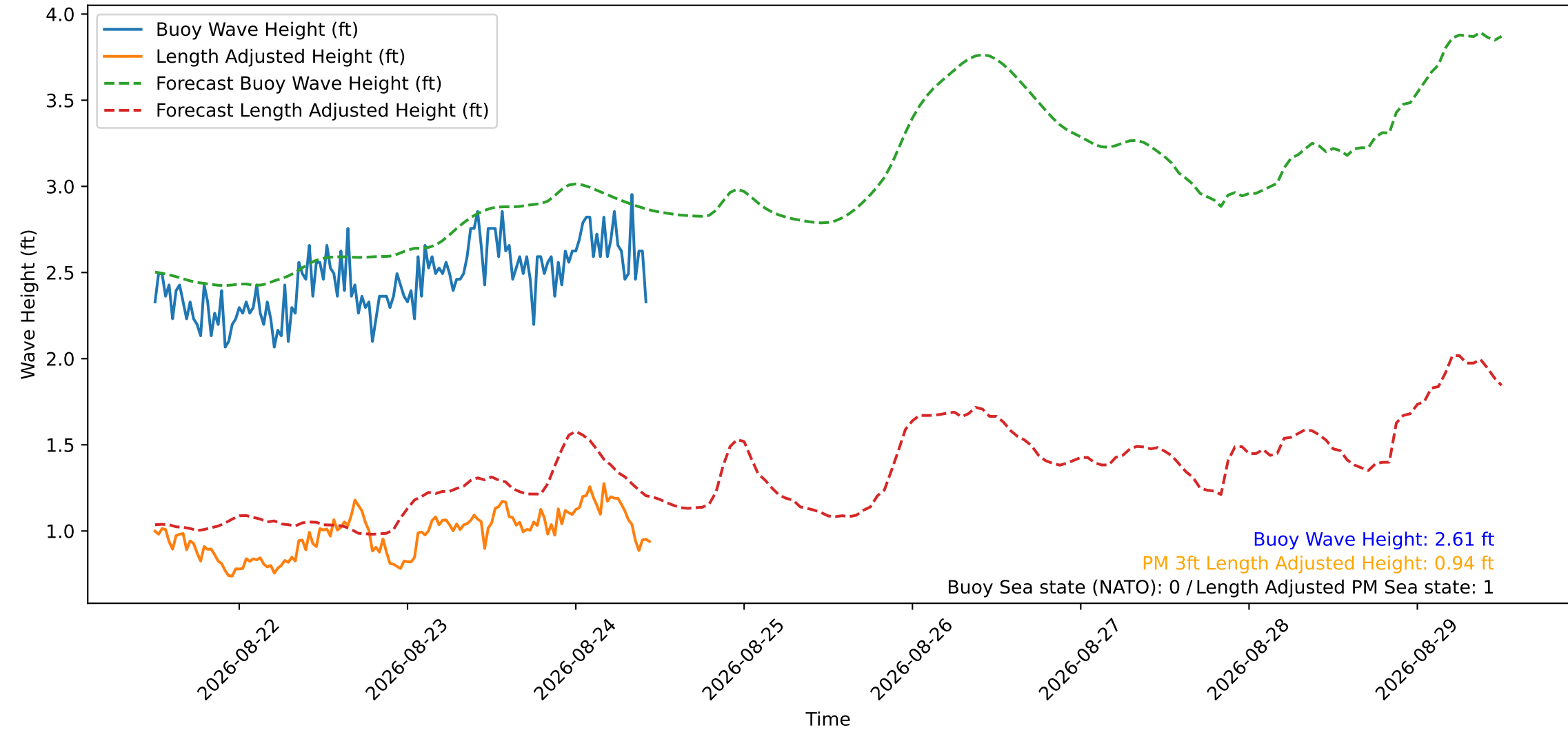
Wave Heights over Time for Red Beach at 2026-08-24 11:30:49
