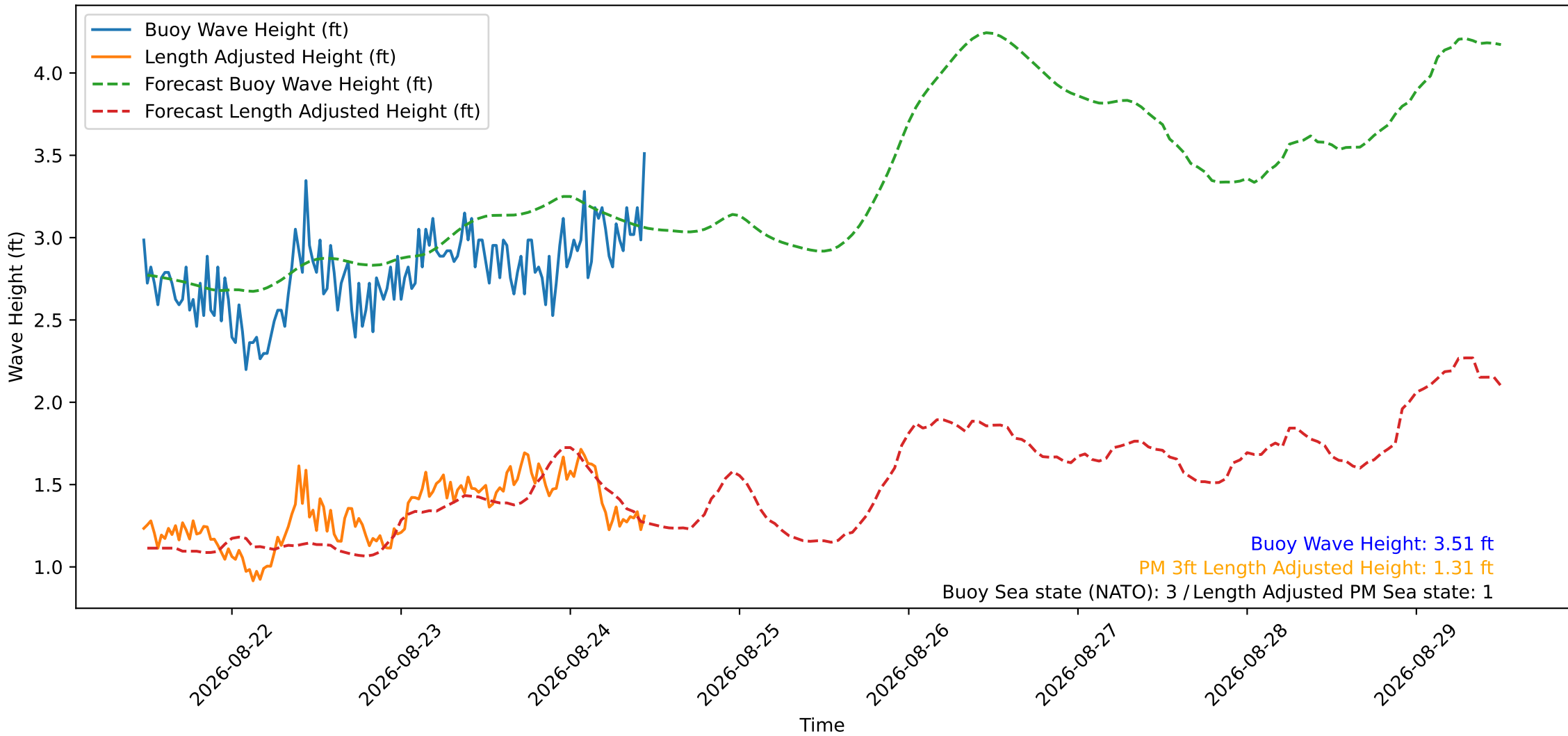
Wave Heights over Time for Oceanside Harbor at 2026-08-24 11:30:30
