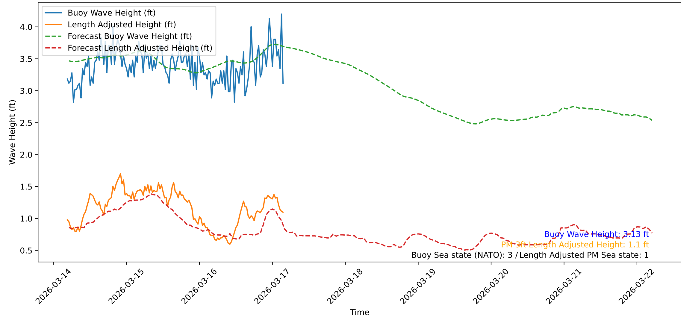
Wave Heights over Time for Green Beach at 2026-03-17 04:31:48
