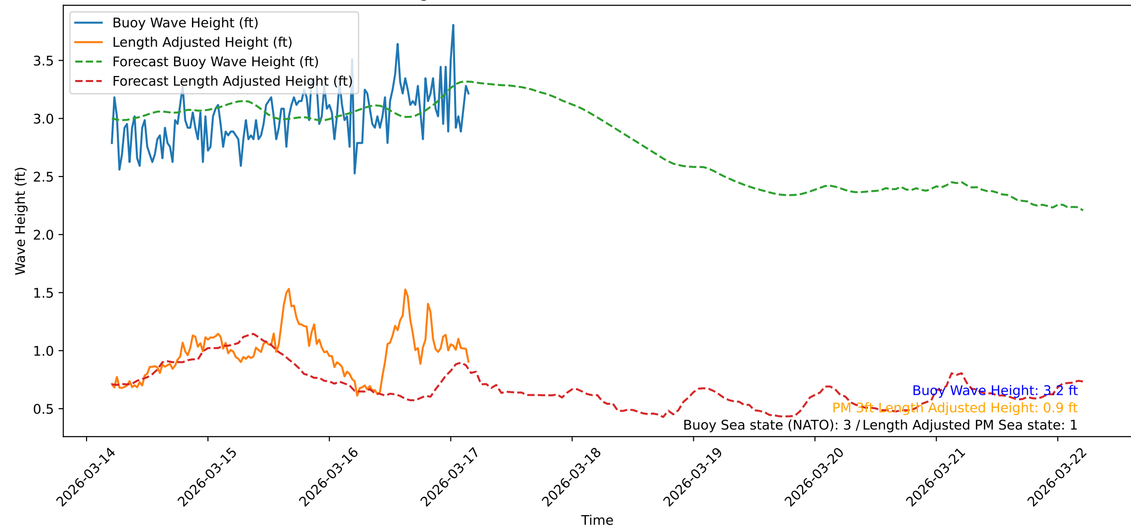
Wave Heights over Time for Red Beach at 2026-03-17 04:31:09
