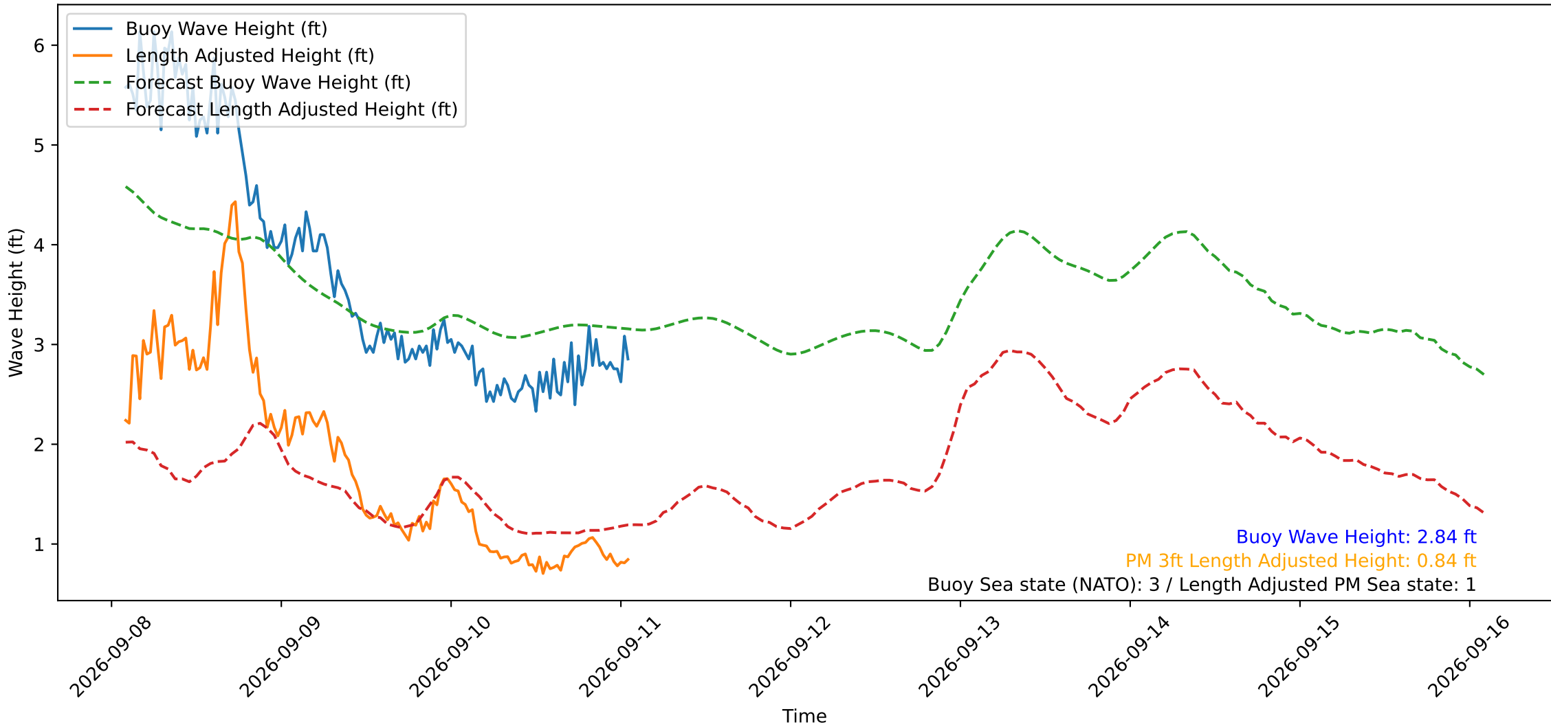
Wave Heights over Time for Red Beach at 2026-09-11 01:50:57
