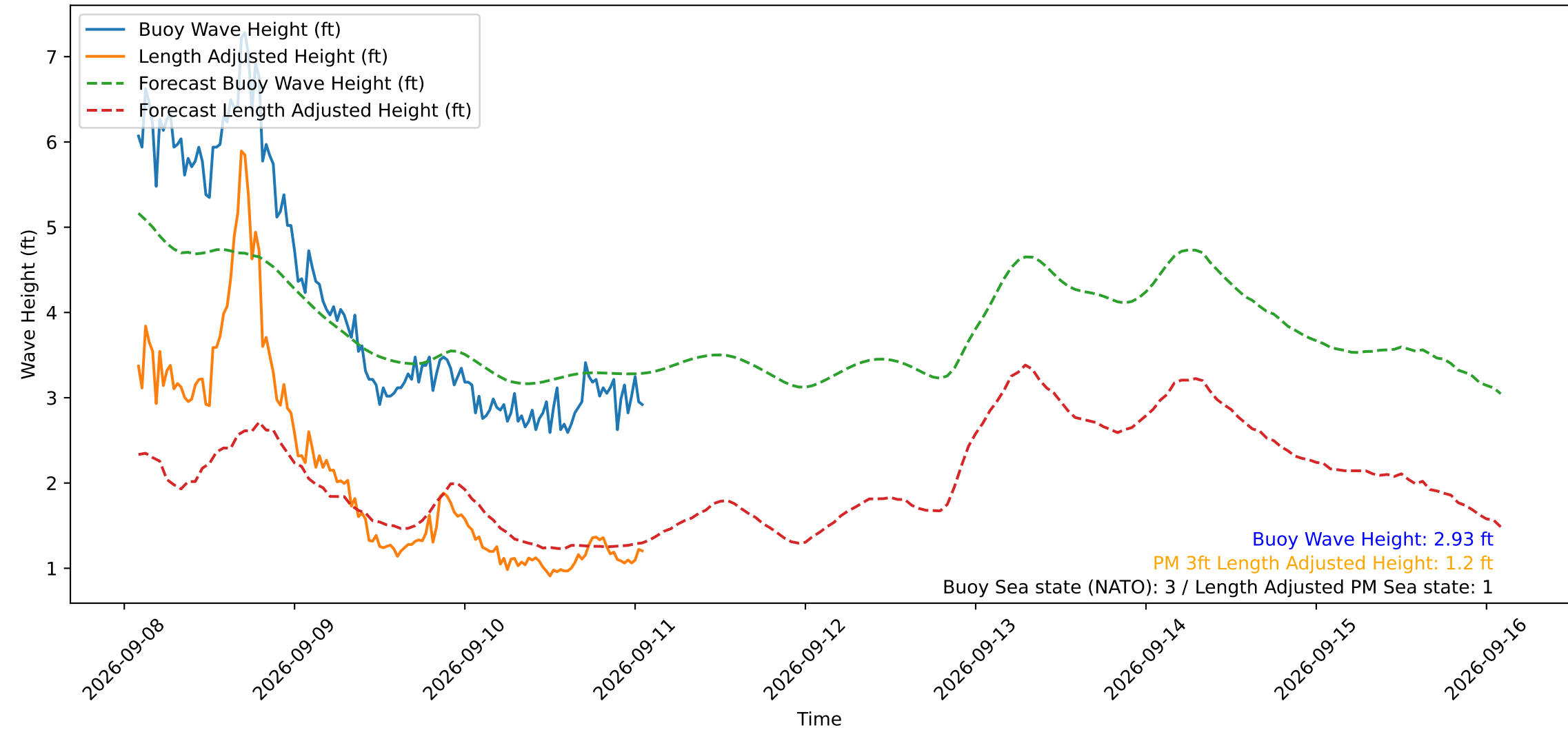
Wave Heights over Time for Green Beach at 2026-09-11 01:51:20
