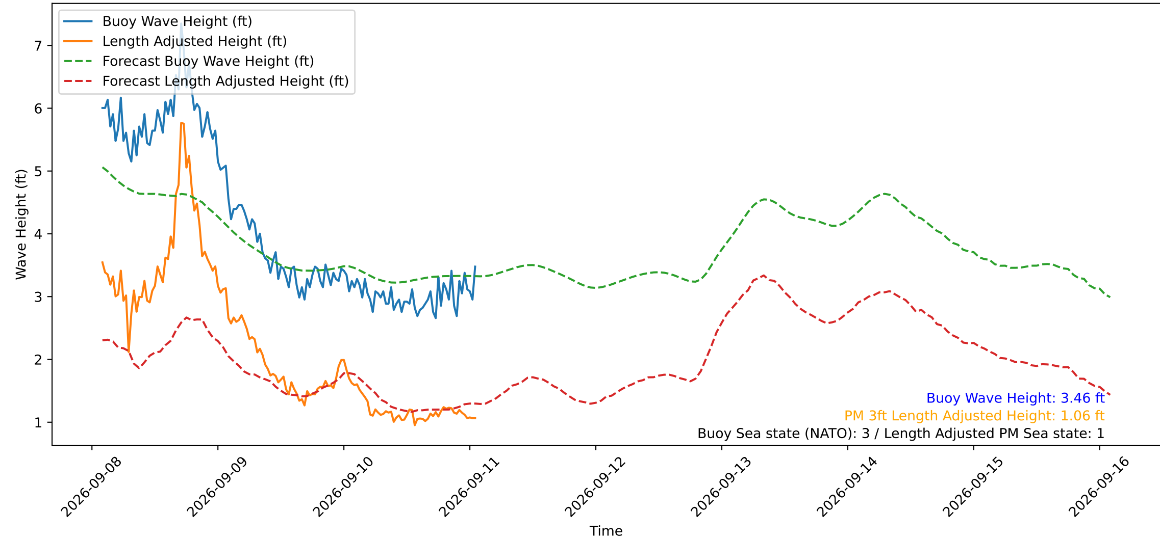
Wave Heights over Time for Oceanside Harbor at 2026-09-11 01:50:36
