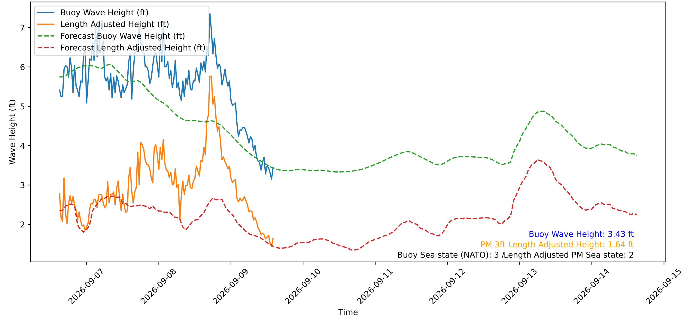
Wave Heights over Time for Oceanside Harbor at 2026-09-09 15:00:29
