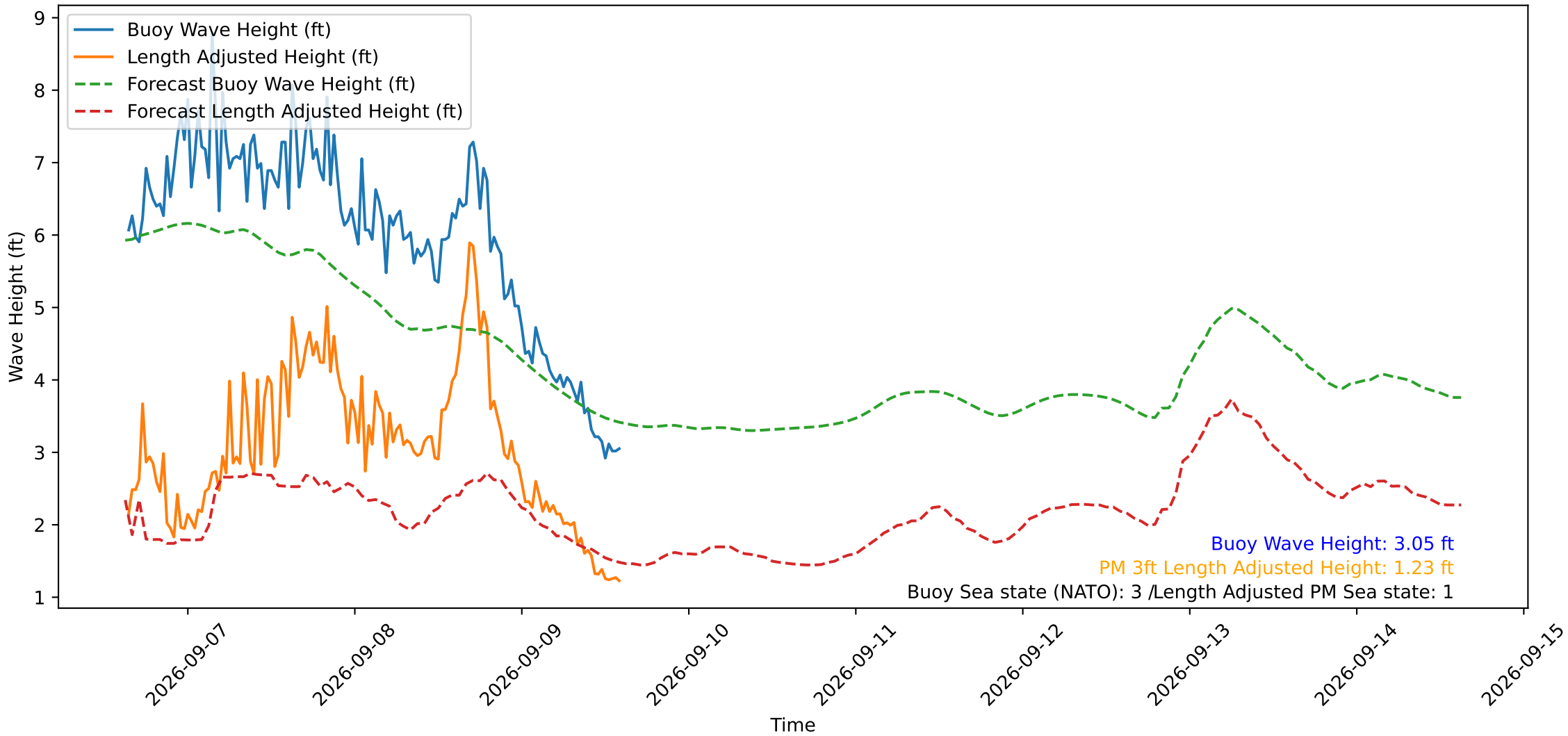
Wave Heights over Time for Green Beach at 2026-09-09 15:01:12
