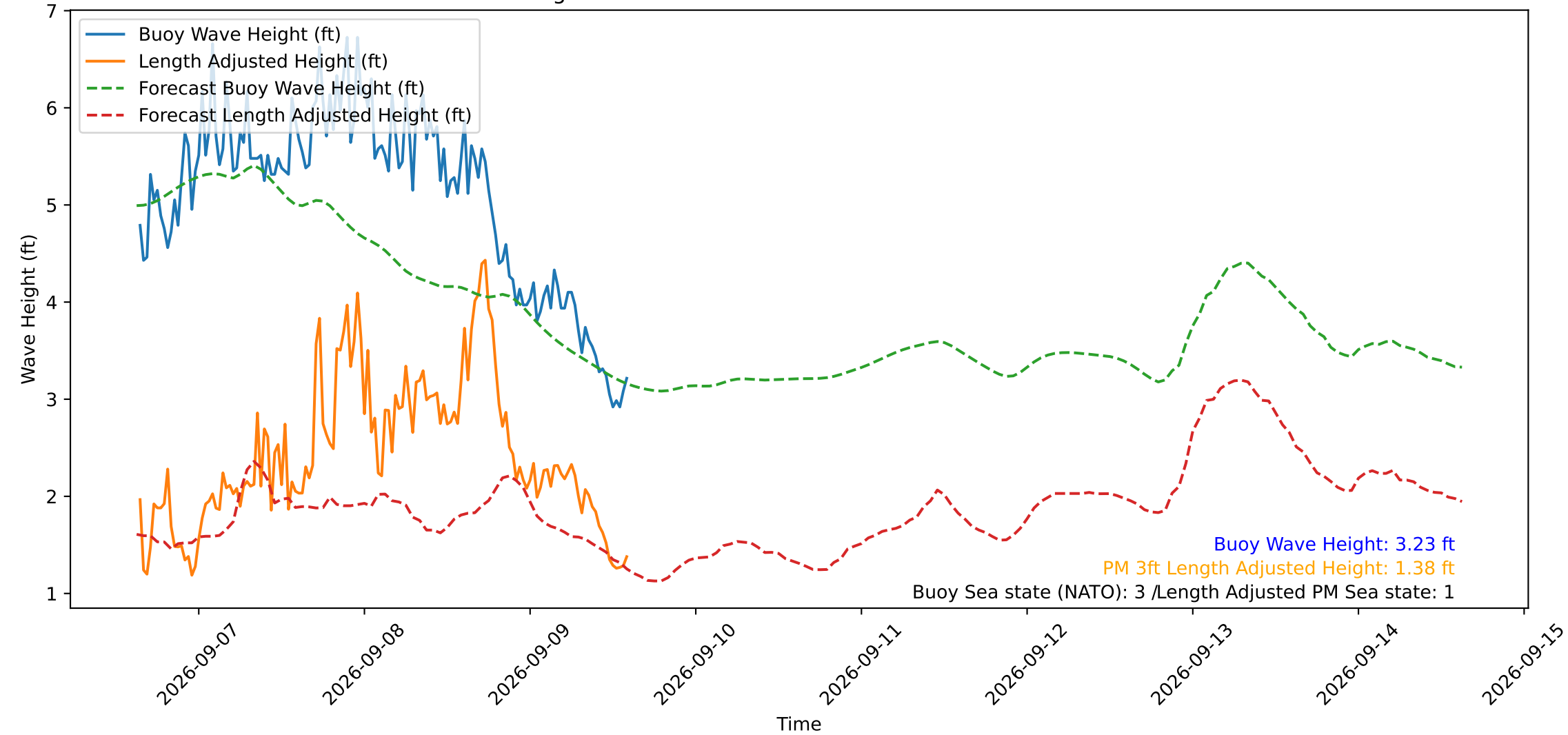
Wave Heights over Time for Red Beach at 2026-09-09 15:00:49
