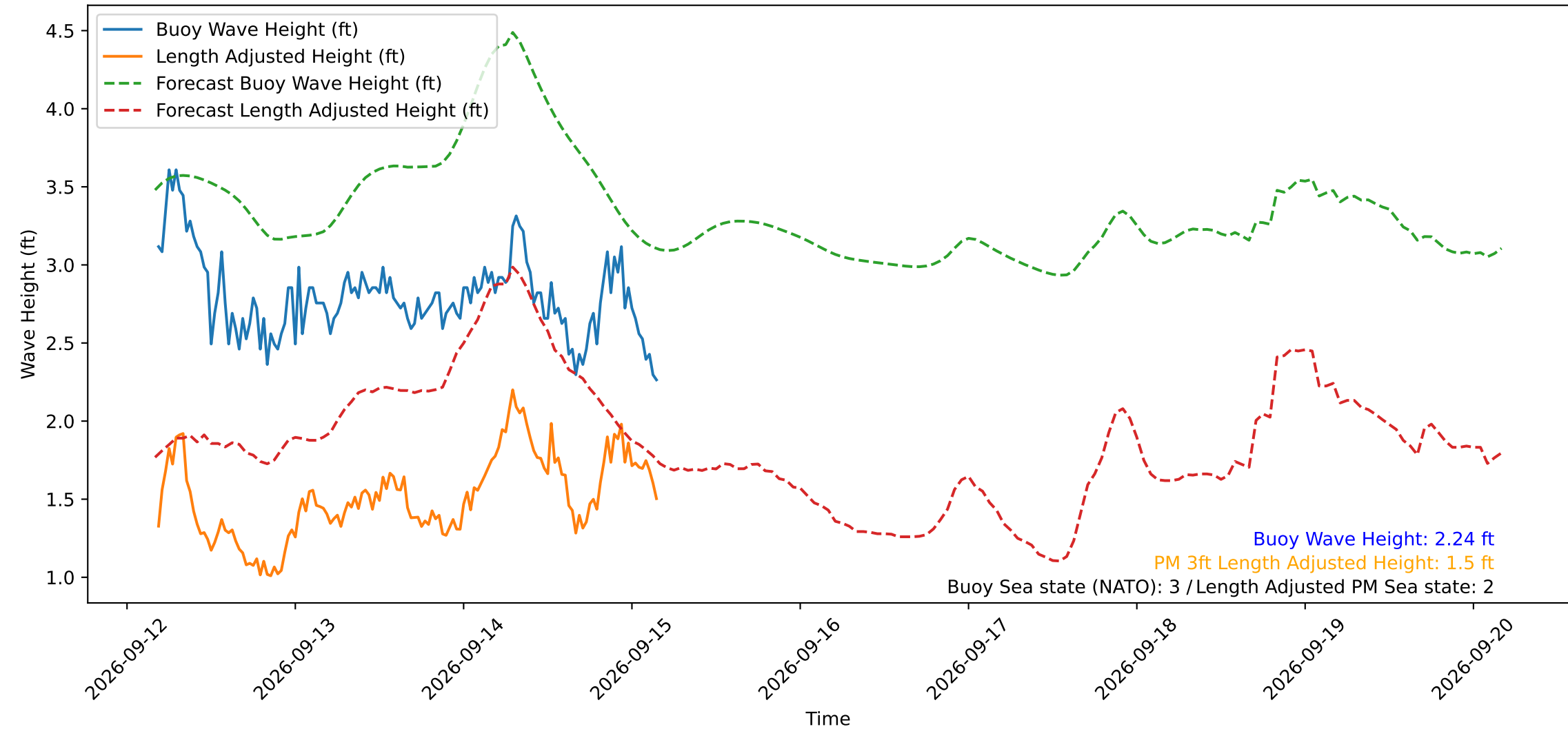
Wave Heights over Time for Green Beach at 2026-09-15 04:11:12
