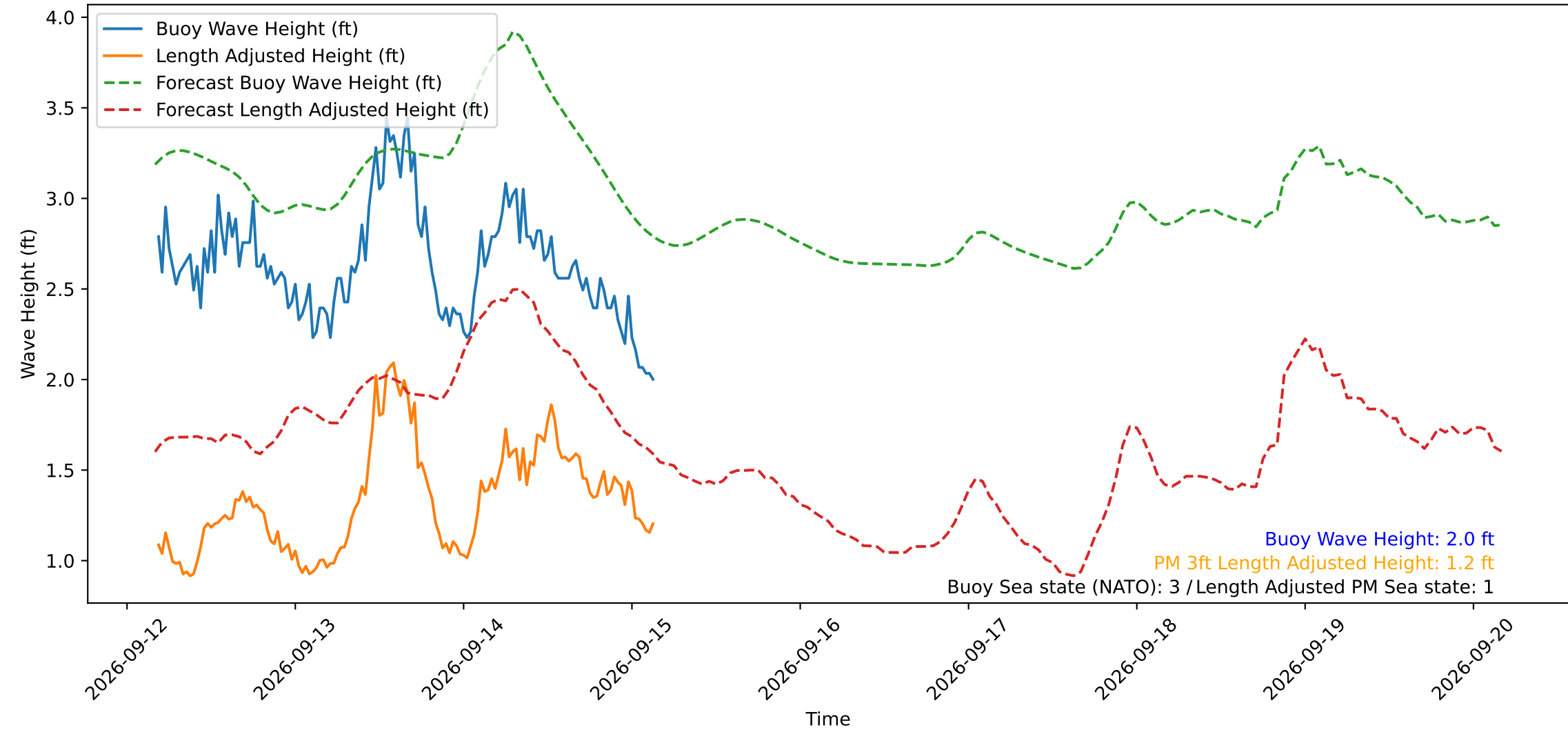
Wave Heights over Time for Red Beach at 2026-09-15 04:10:49
