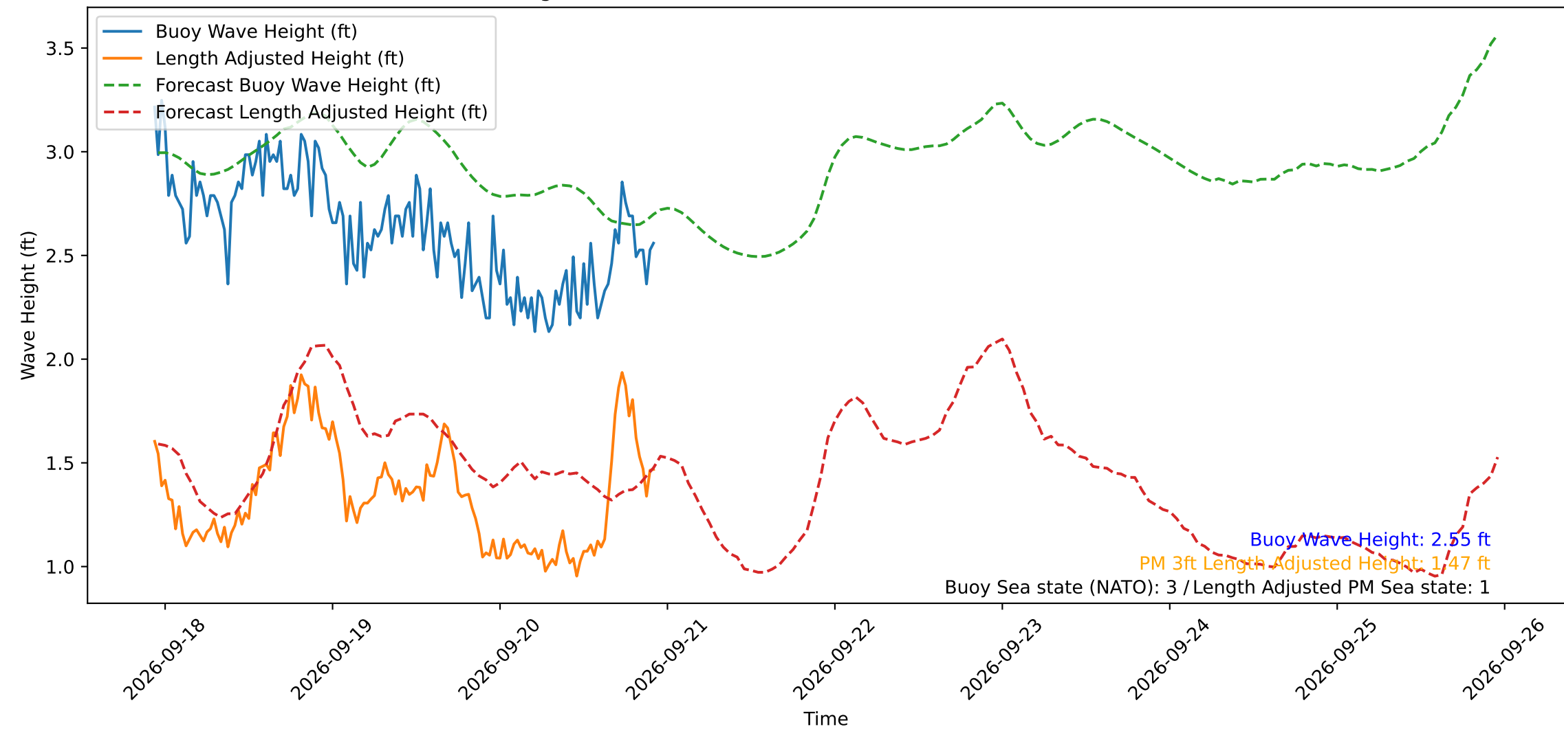
Wave Heights over Time for Oceanside Harbor at 2026-09-20 22:40:30
