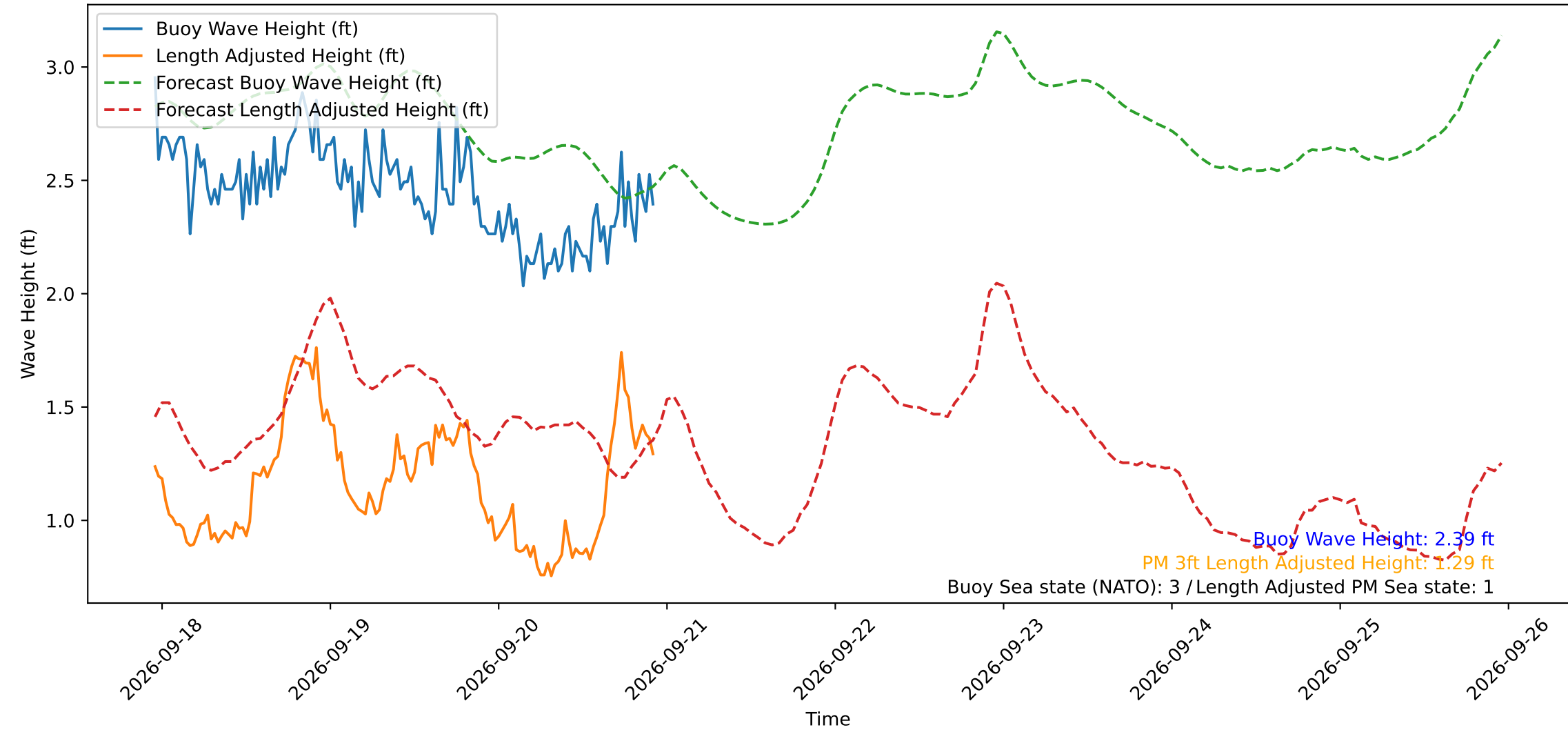
Wave Heights over Time for Red Beach at 2026-09-20 22:40:50
