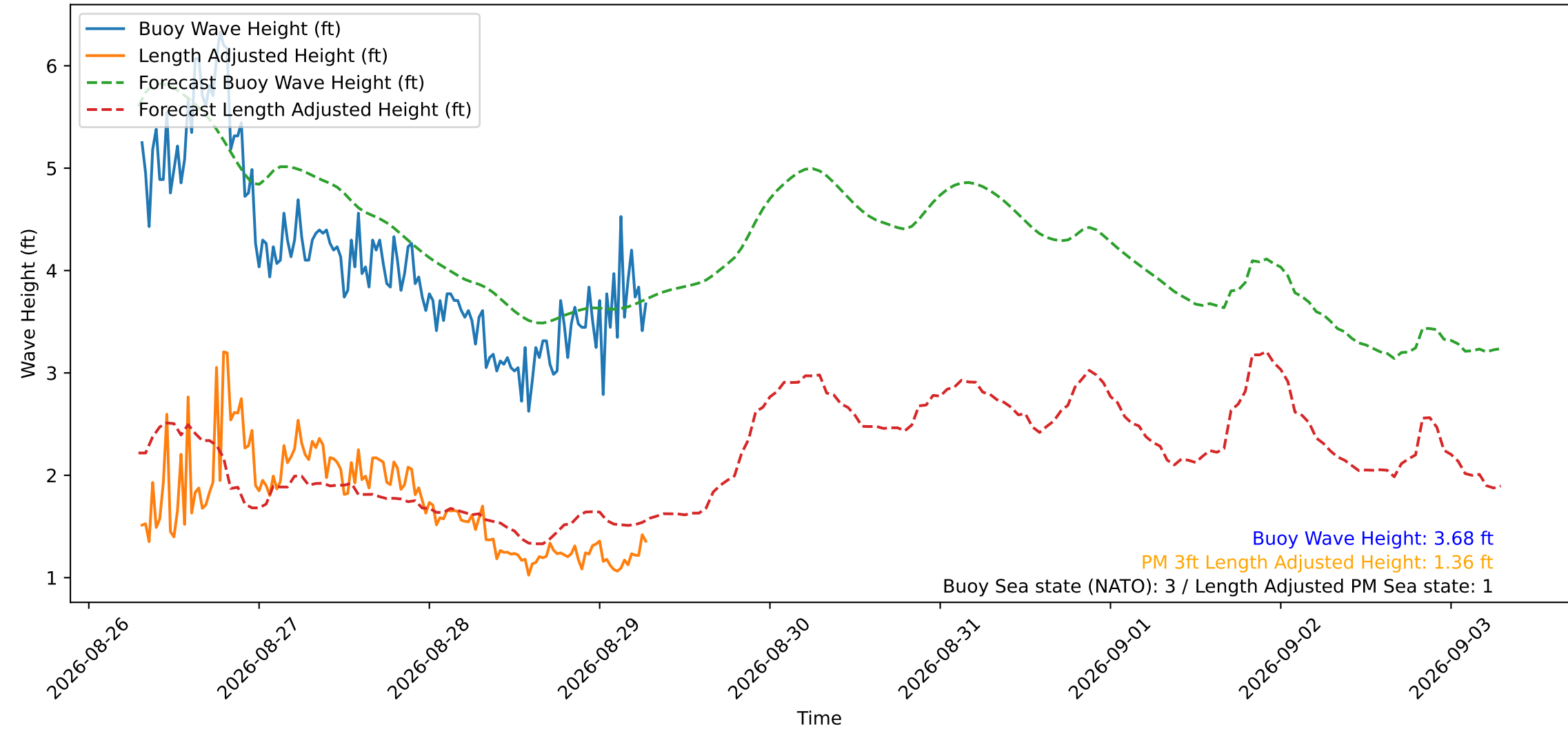
Wave Heights over Time for Green Beach at 2026-08-29 07:21:15
