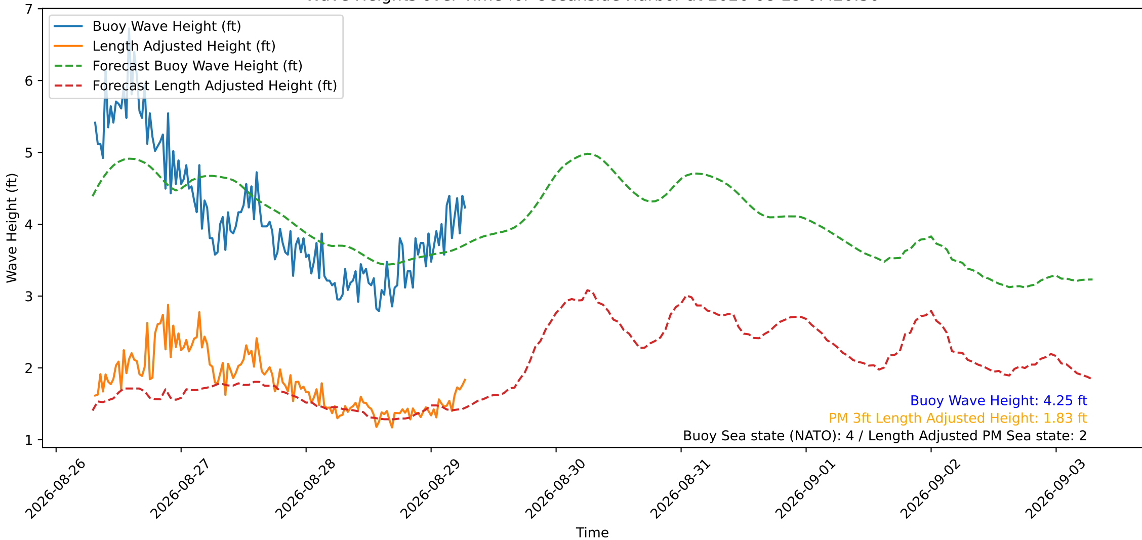
Wave Heights over Time for Oceanside Harbor at 2026-08-29 07:20:30
