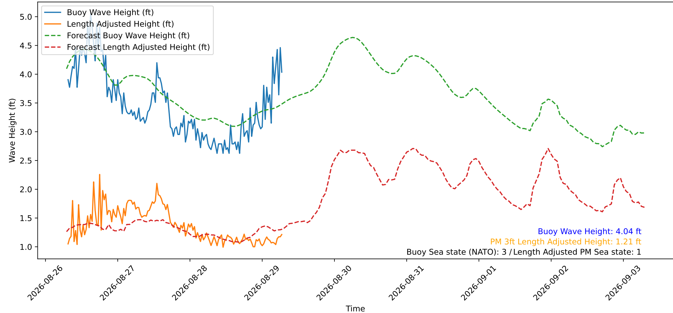
Wave Heights over Time for Red Beach at 2026-08-29 07:20:50
