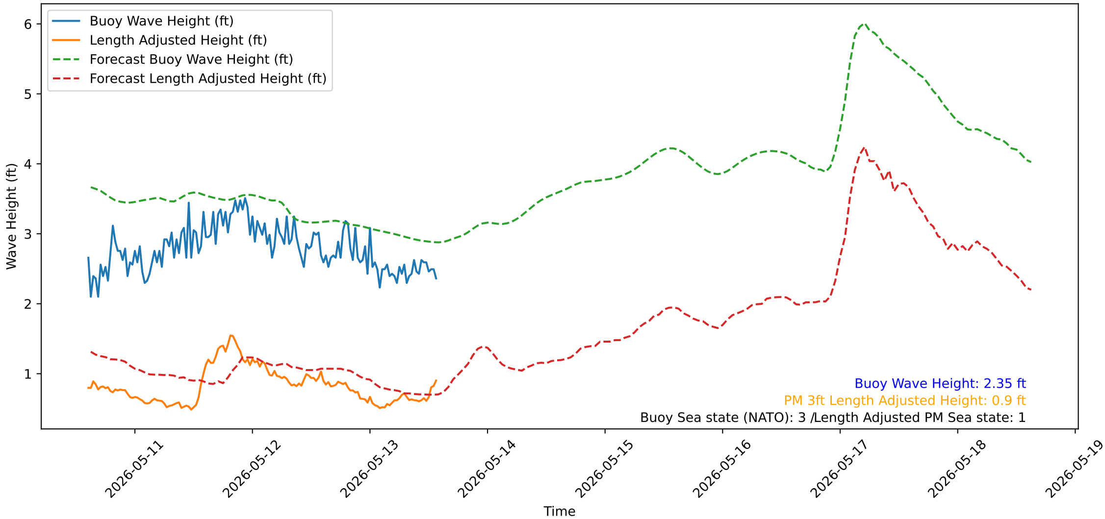
Wave Heights over Time for Green Beach at 2026-05-13 14:31:13
