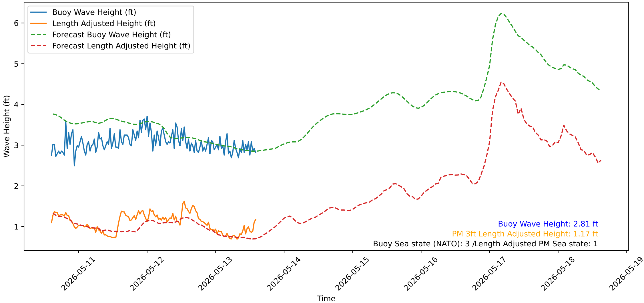
Wave Heights over Time for Oceanside Harbor at 2026-05-13 14:30:32
