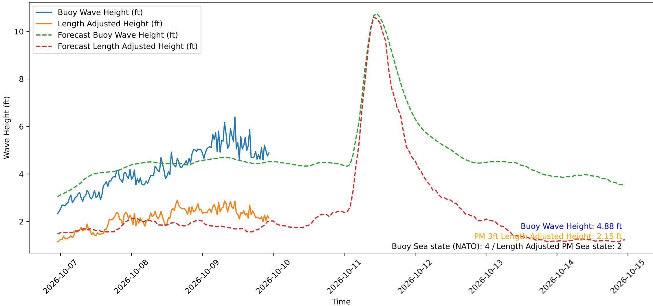
Wave Heights over Time for Oceanside Harbor at 2026-10-09 23:10:30
