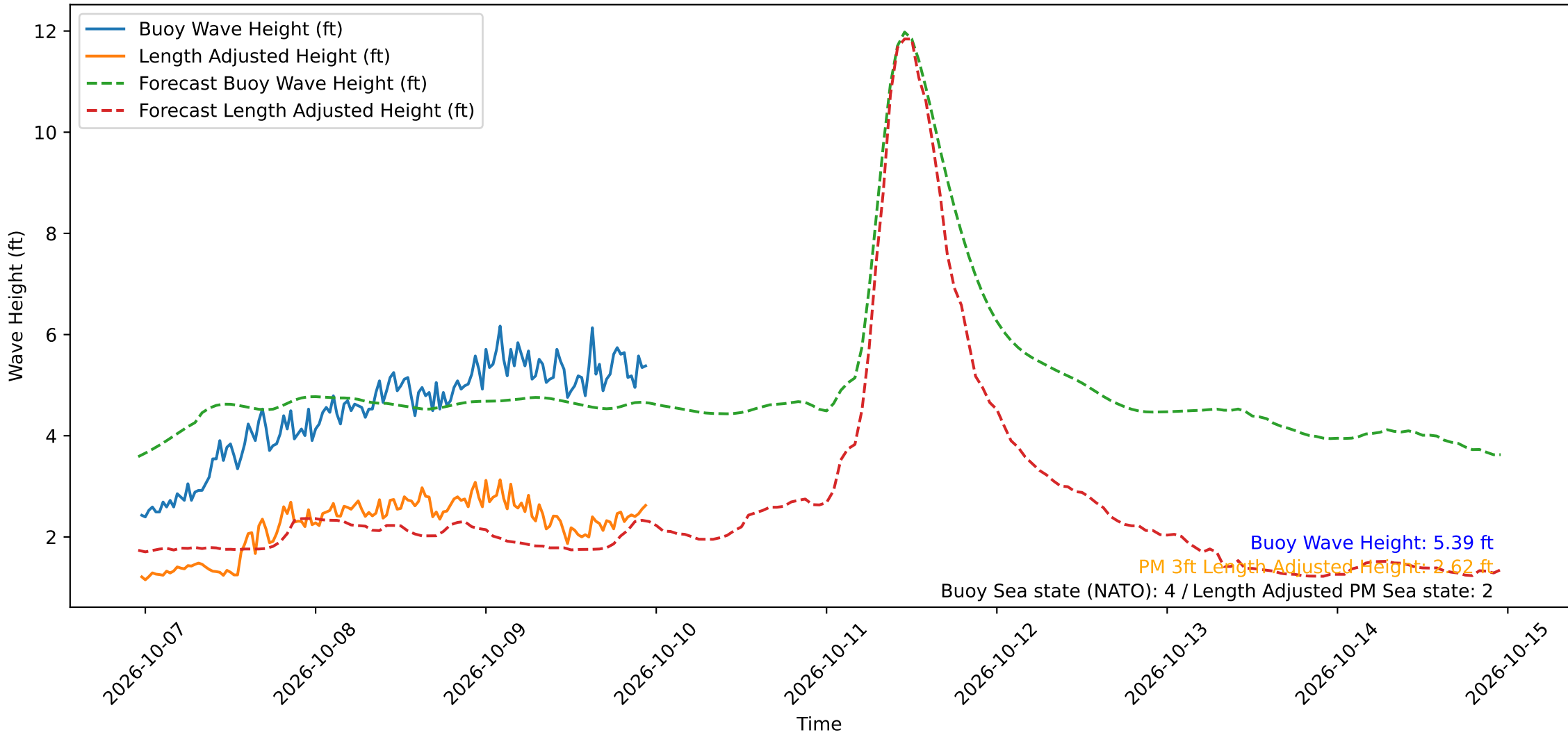
Wave Heights over Time for Green Beach at 2026-10-09 23:11:12
