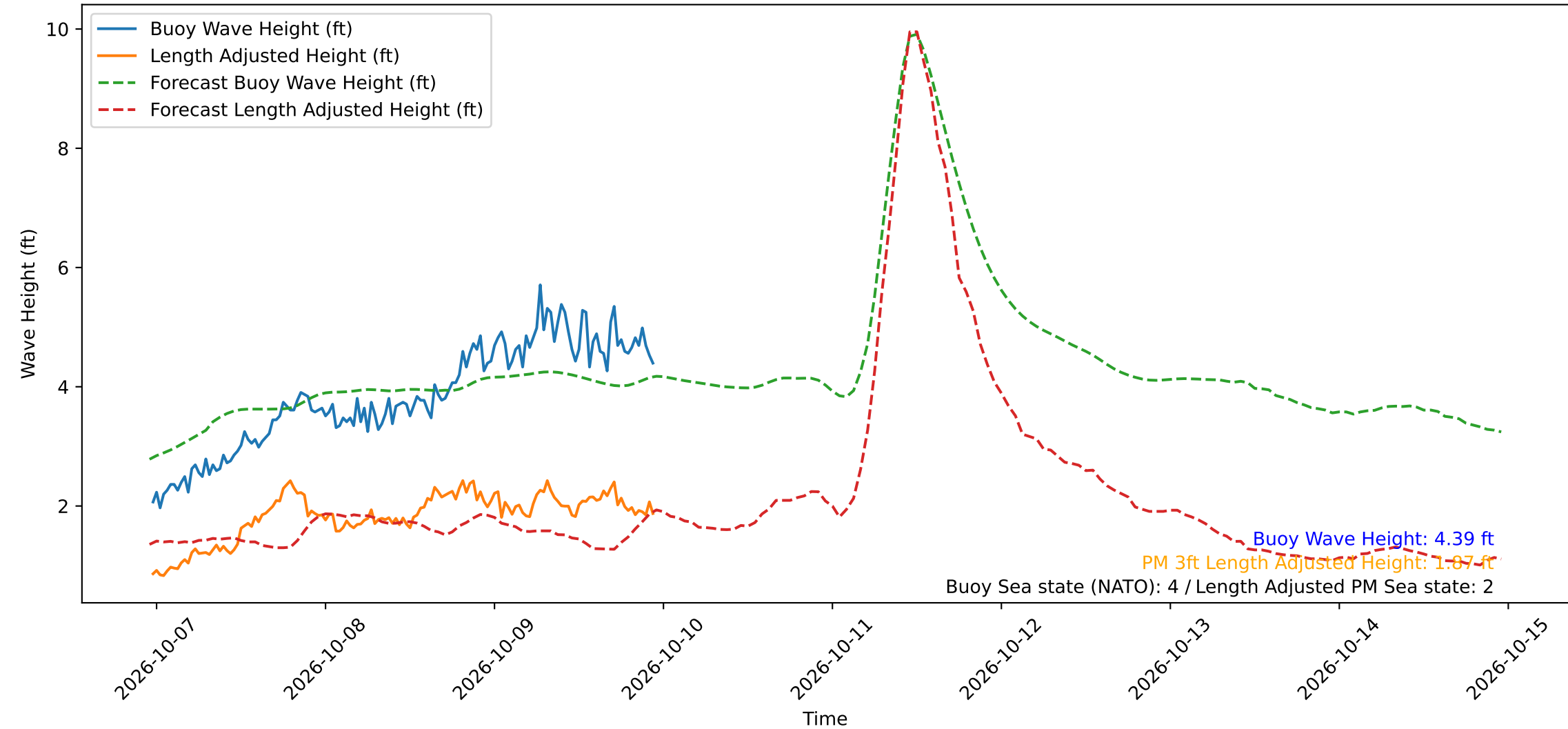
Wave Heights over Time for Red Beach at 2026-10-09 23:10:49
