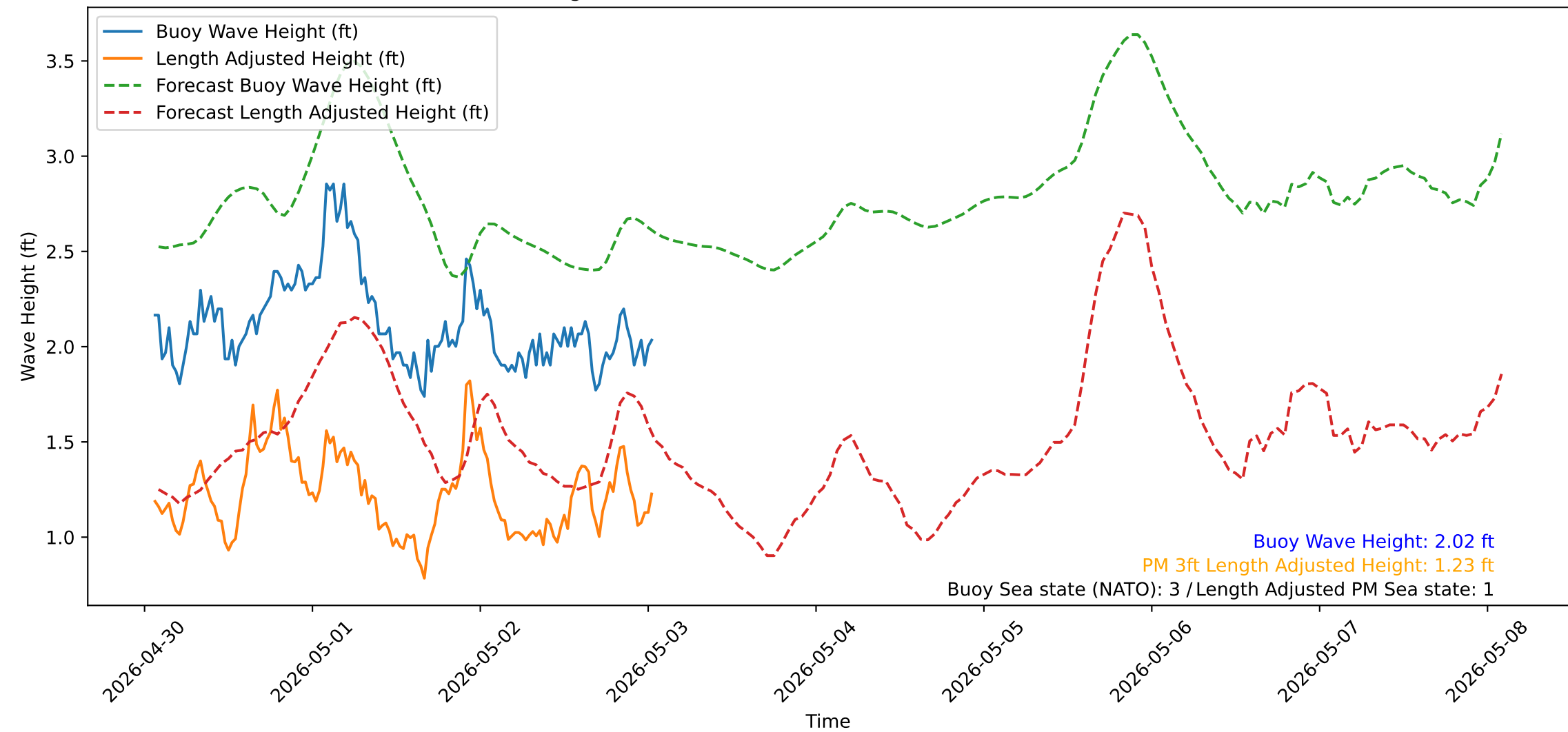
Wave Heights over Time for Green Beach at 2026-05-03 01:31:12
