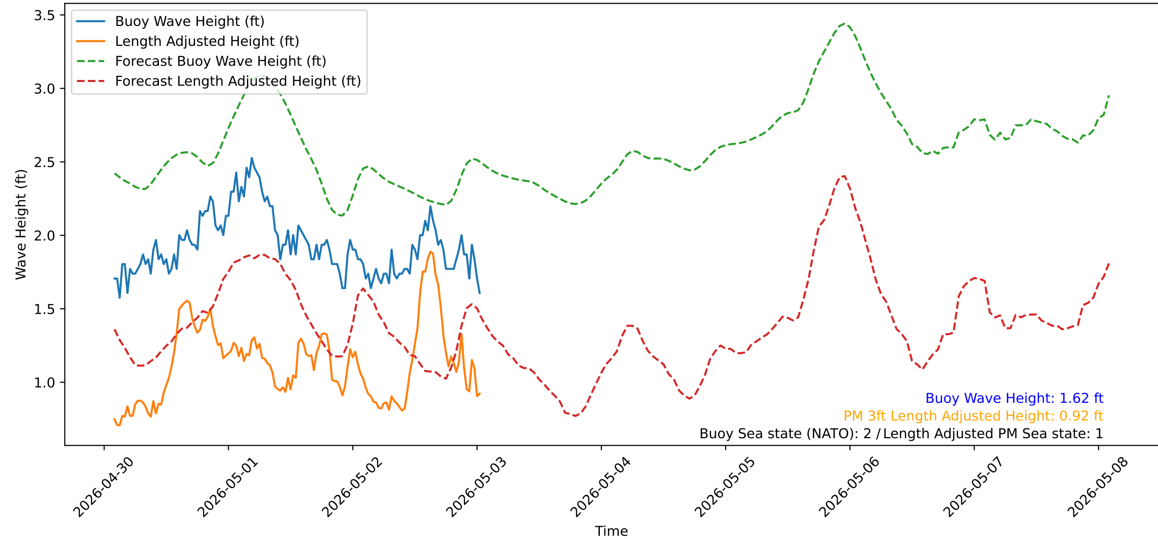
Wave Heights over Time for Red Beach at 2026-05-03 01:30:50
