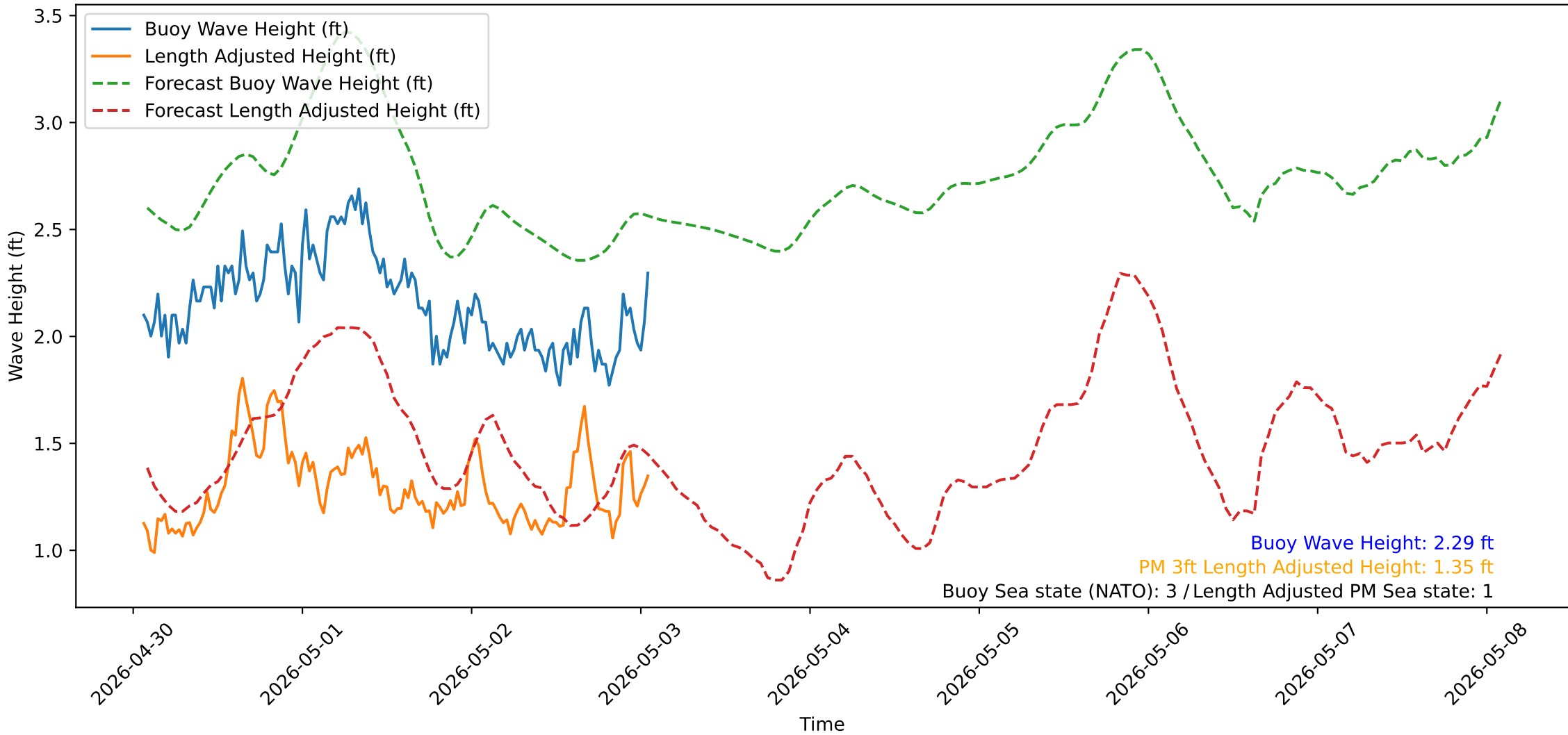
Wave Heights over Time for Oceanside Harbor at 2026-05-03 01:30:31
