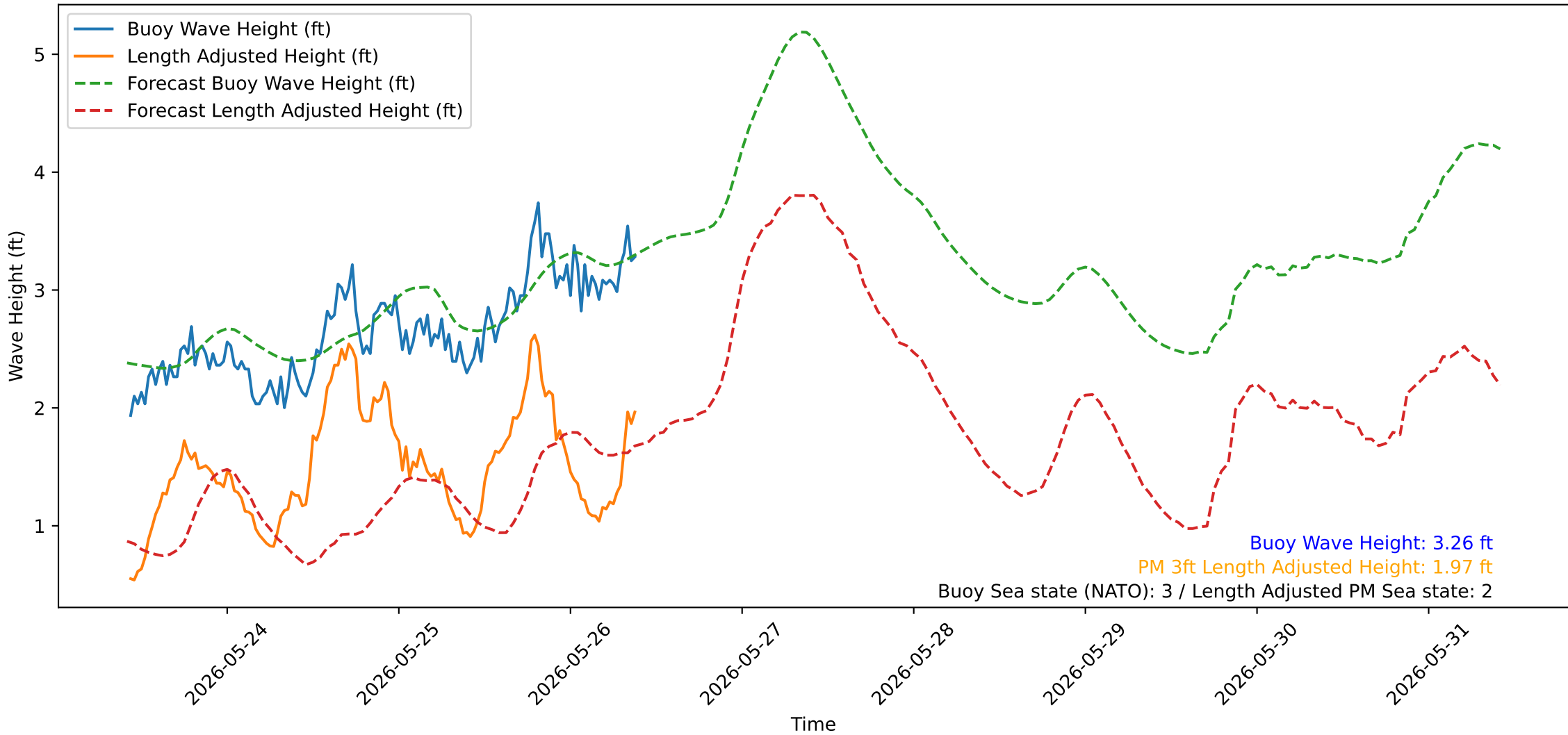
Wave Heights over Time for Red Beach at 2026-05-26 10:20:49
