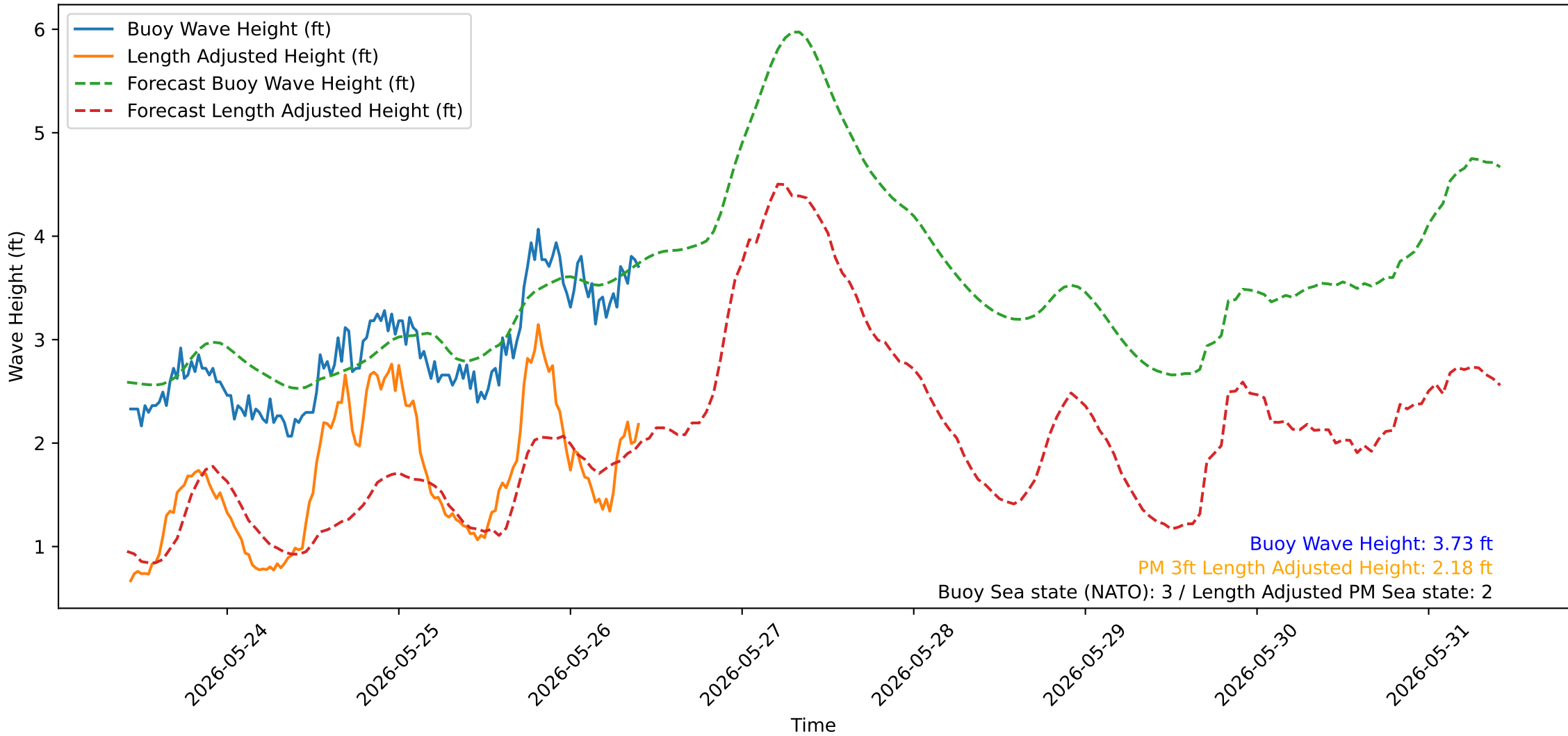
Wave Heights over Time for Green Beach at 2026-05-26 10:21:13
