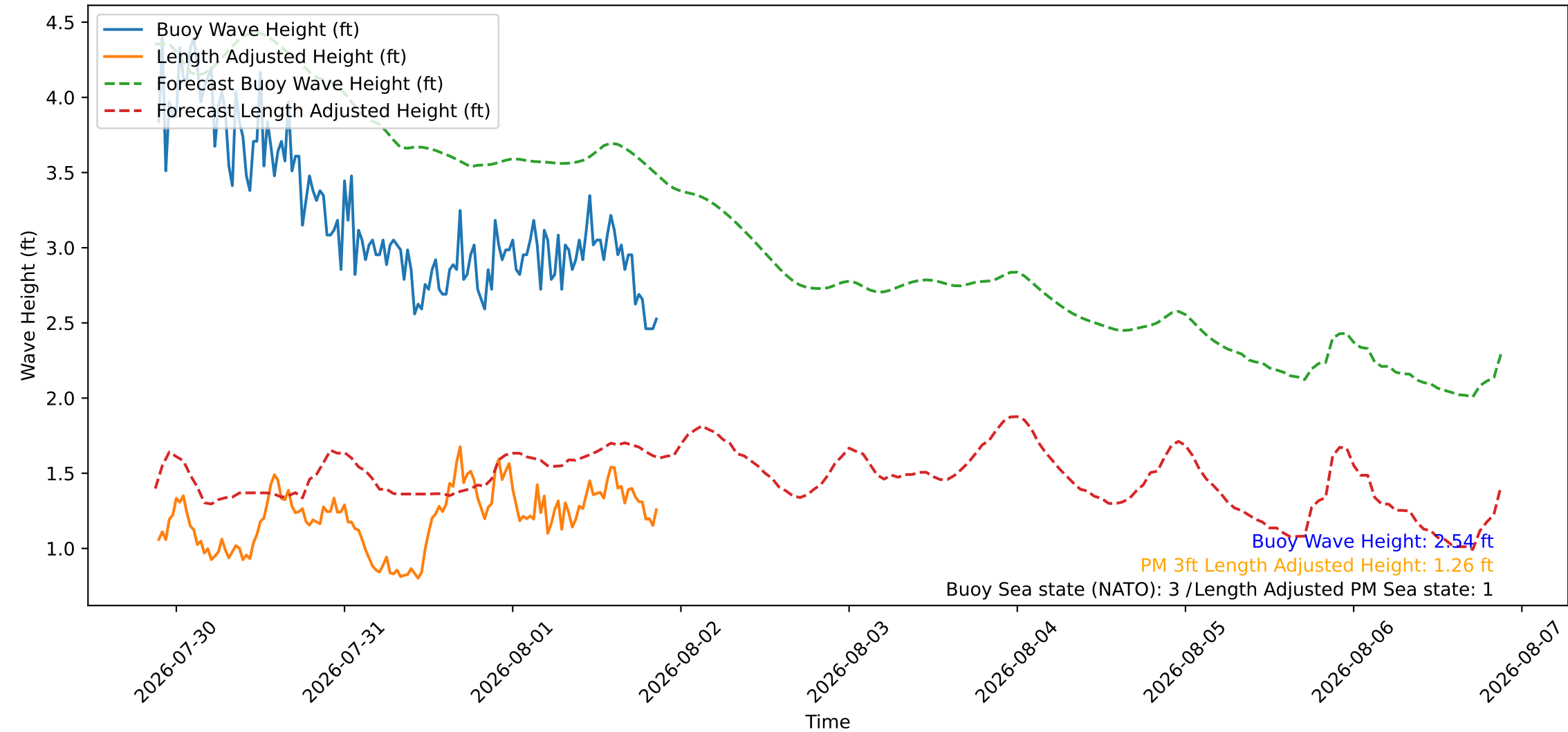
Wave Heights over Time for Red Beach at 2026-08-01 21:20:47
