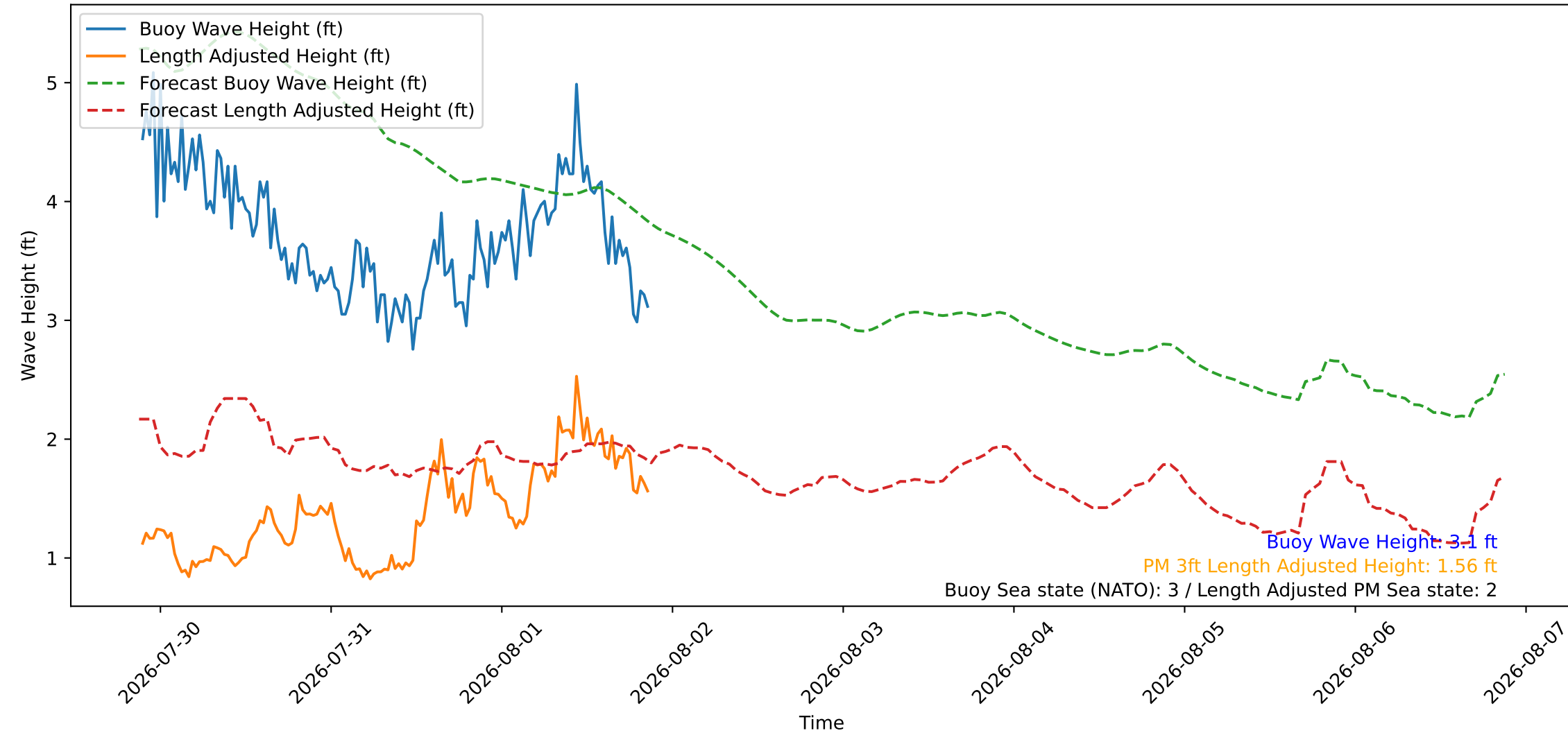
Wave Heights over Time for Green Beach at 2026-08-01 21:21:10
