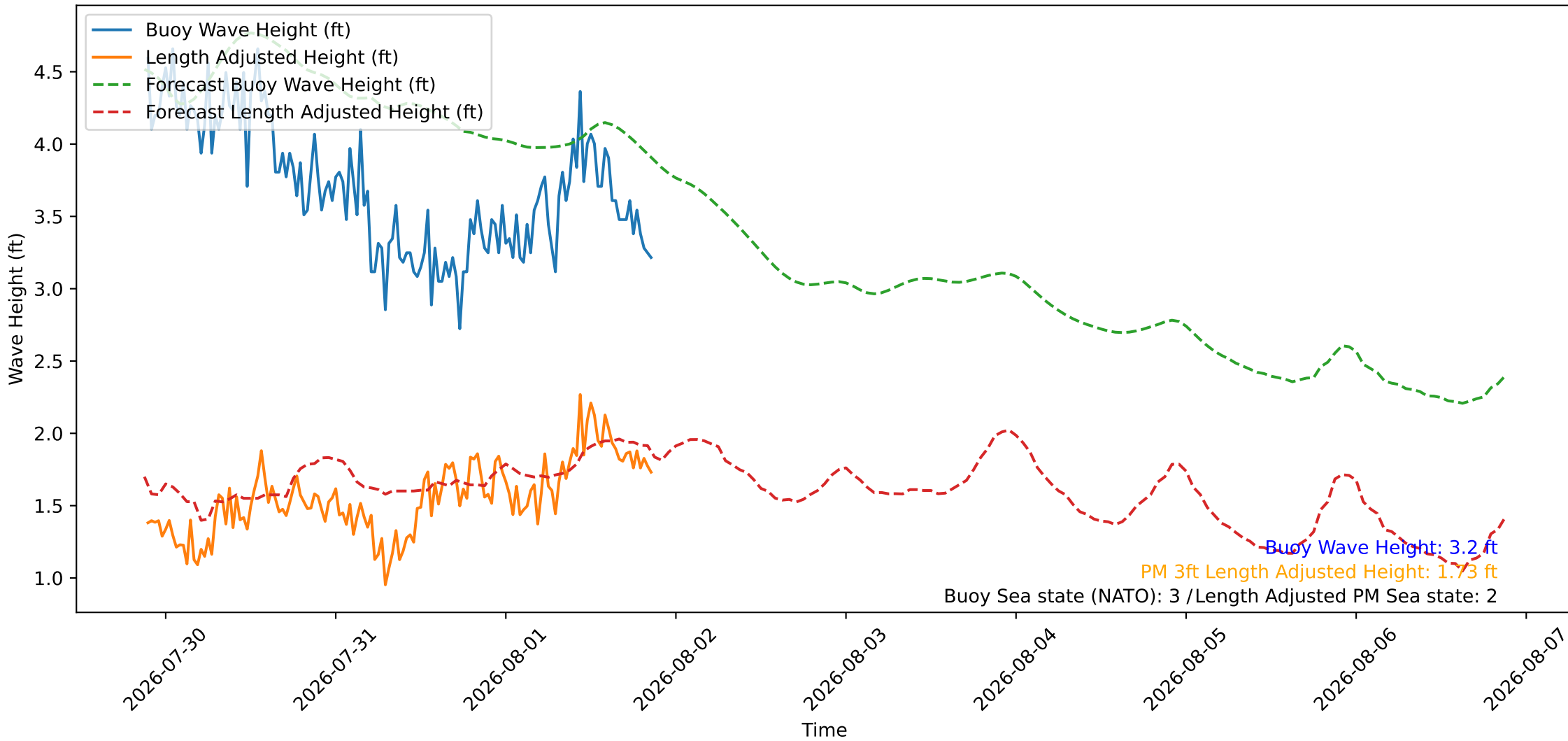
Wave Heights over Time for Oceanside Harbor at 2026-08-01 21:20:26
