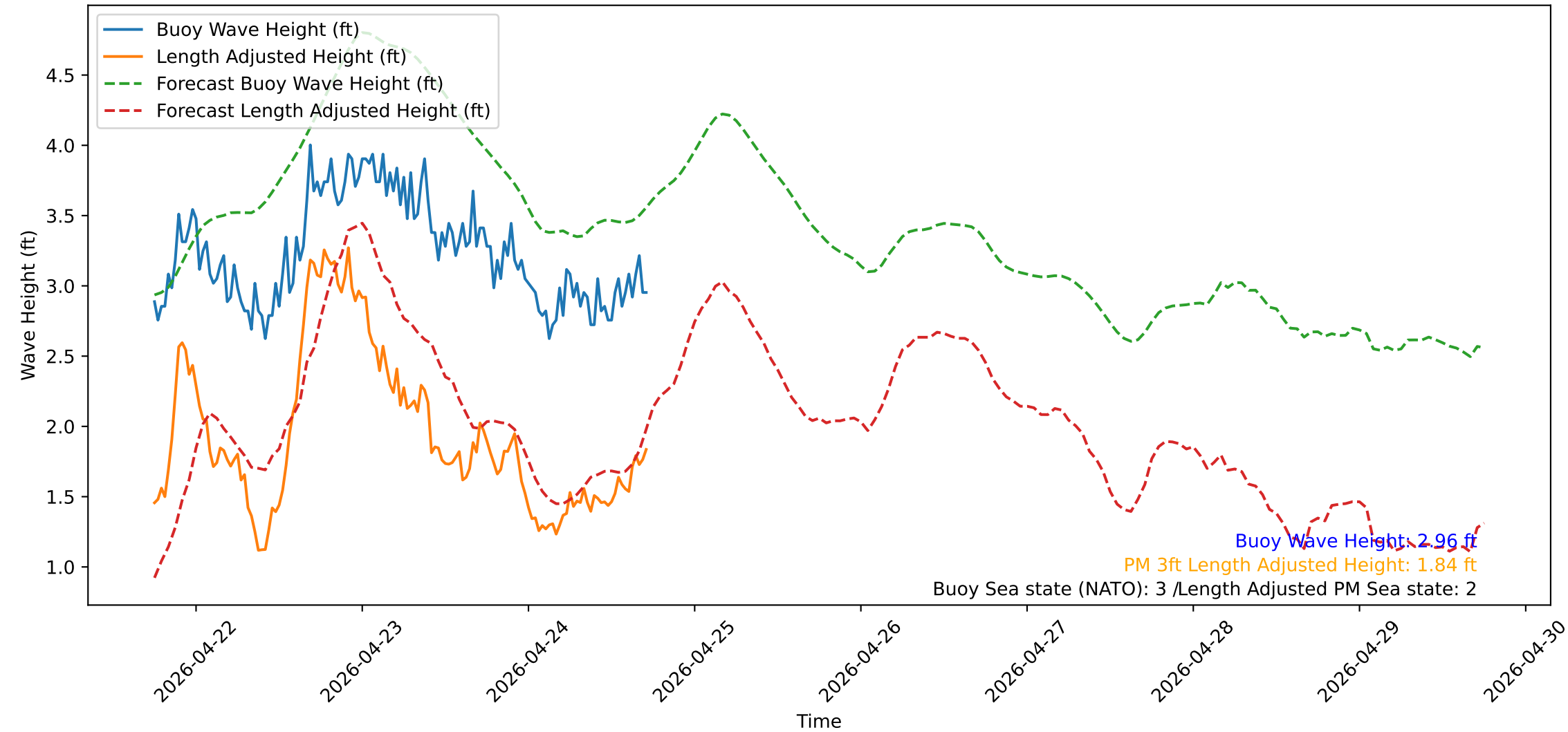
Wave Heights over Time for Green Beach at 2026-04-24 18:01:12
