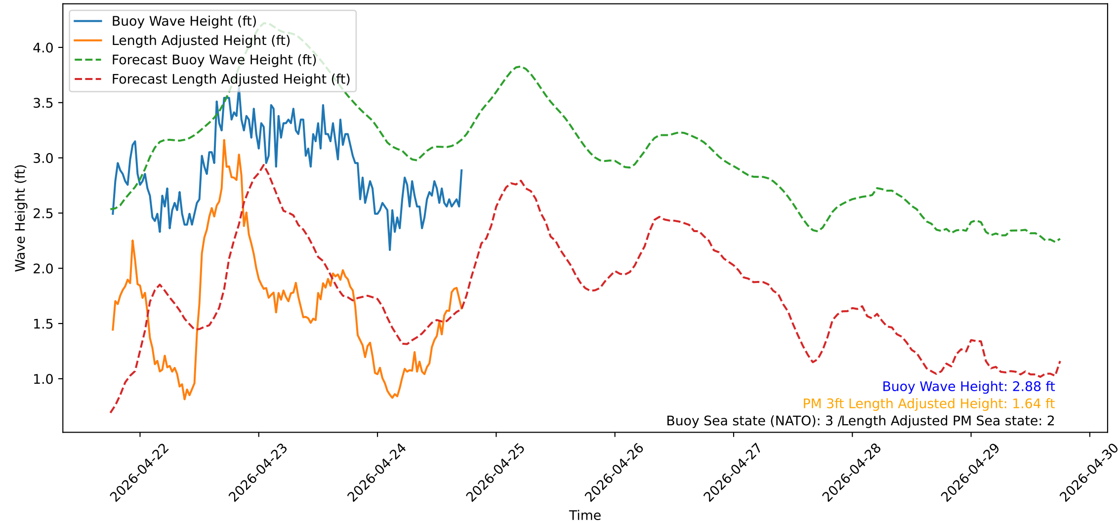
Wave Heights over Time for Red Beach at 2026-04-24 18:00:50
