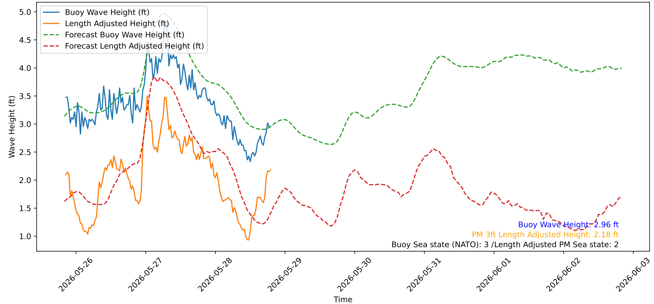
Wave Heights over Time for Red Beach at 2026-05-28 20:00:39
