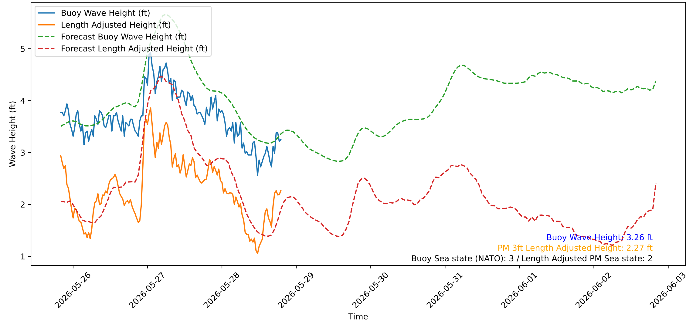
Wave Heights over Time for Green Beach at 2026-05-28 20:01:01
