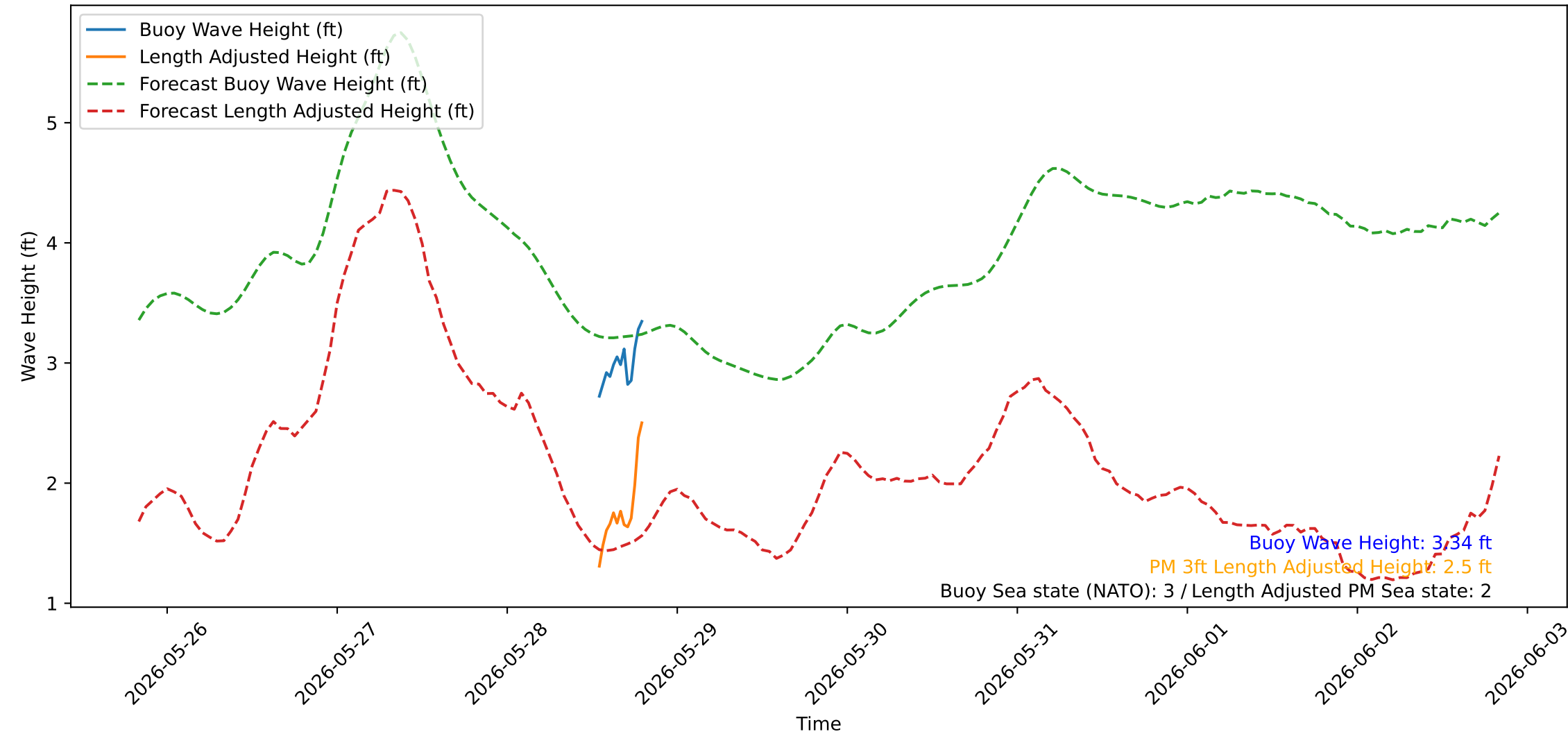
Wave Heights over Time for Oceanside Harbor at 2026-05-28 20:00:20
