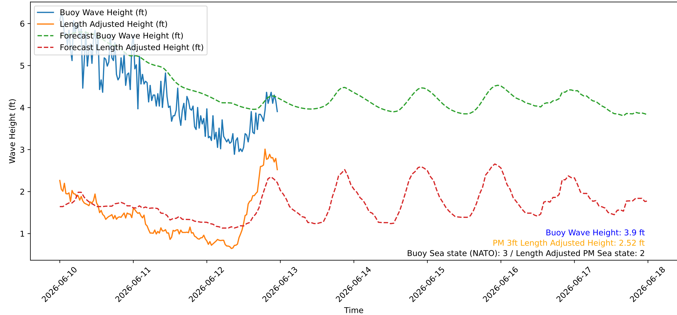
Wave Heights over Time for Green Beach at 2026-06-13 00:01:09
