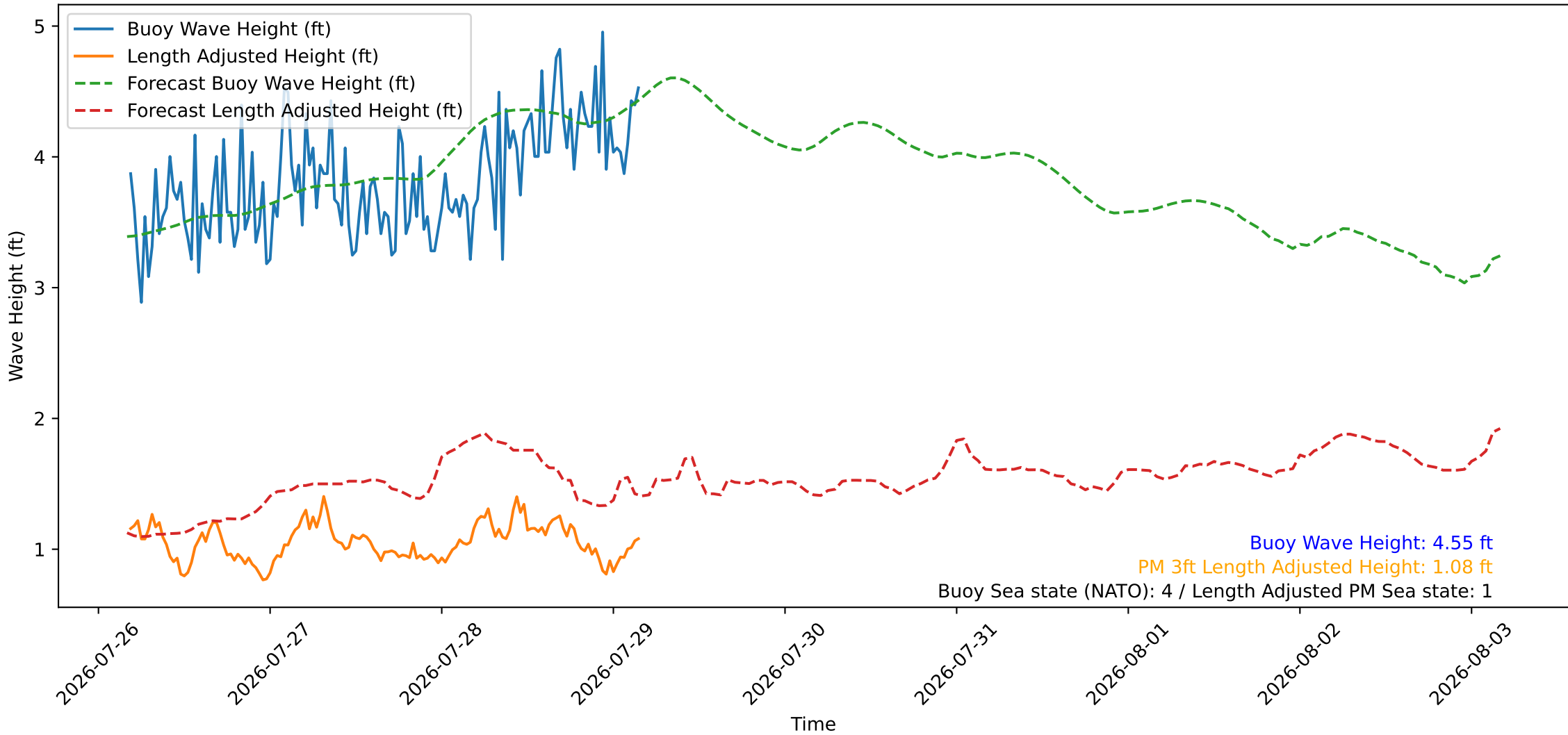
Wave Heights over Time for Red Beach at 2026-07-29 04:20:47
