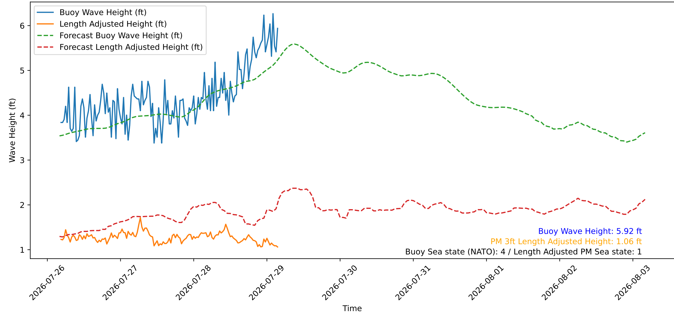
Wave Heights over Time for Green Beach at 2026-07-29 04:21:09
