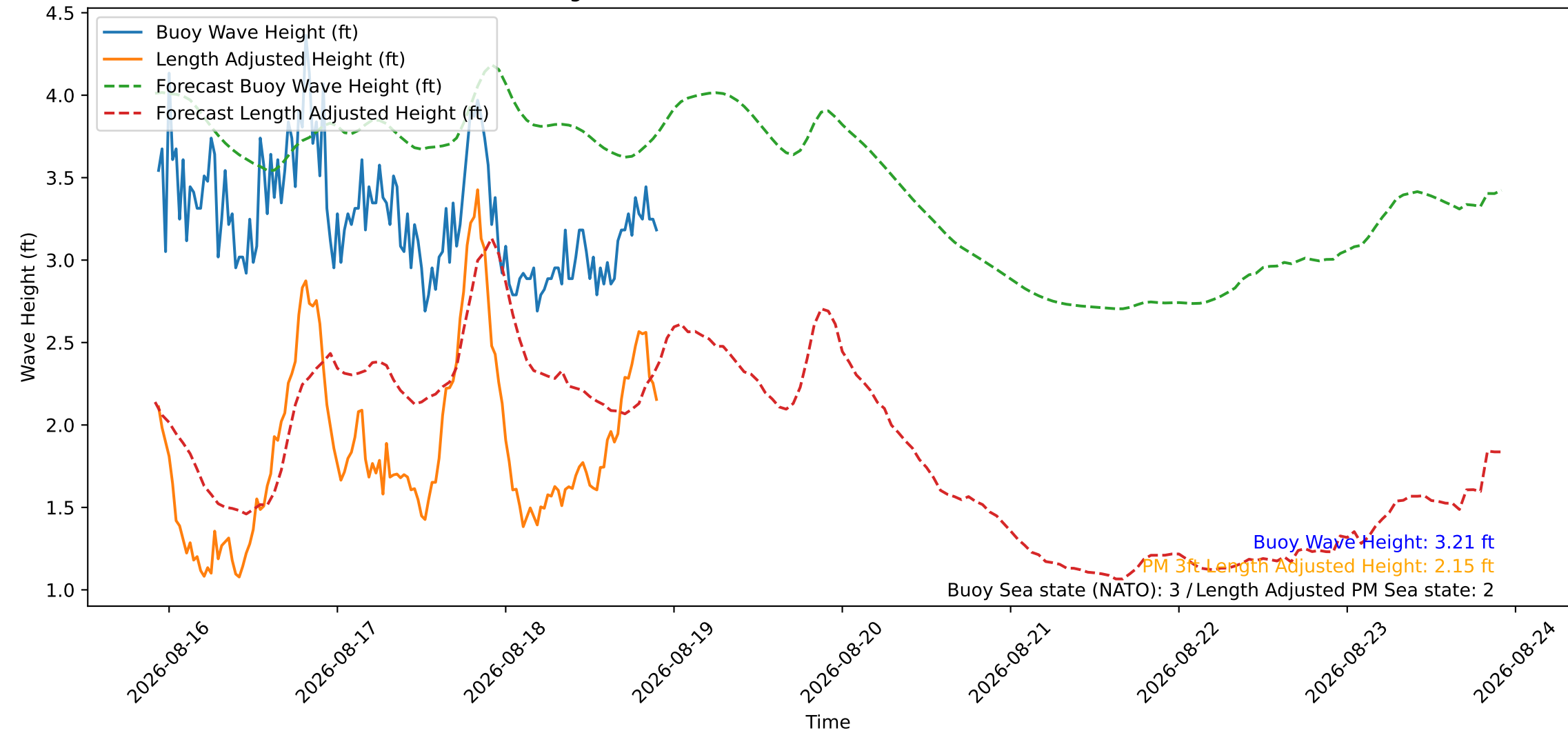
Wave Heights over Time for Green Beach at 2026-08-18 22:11:08
