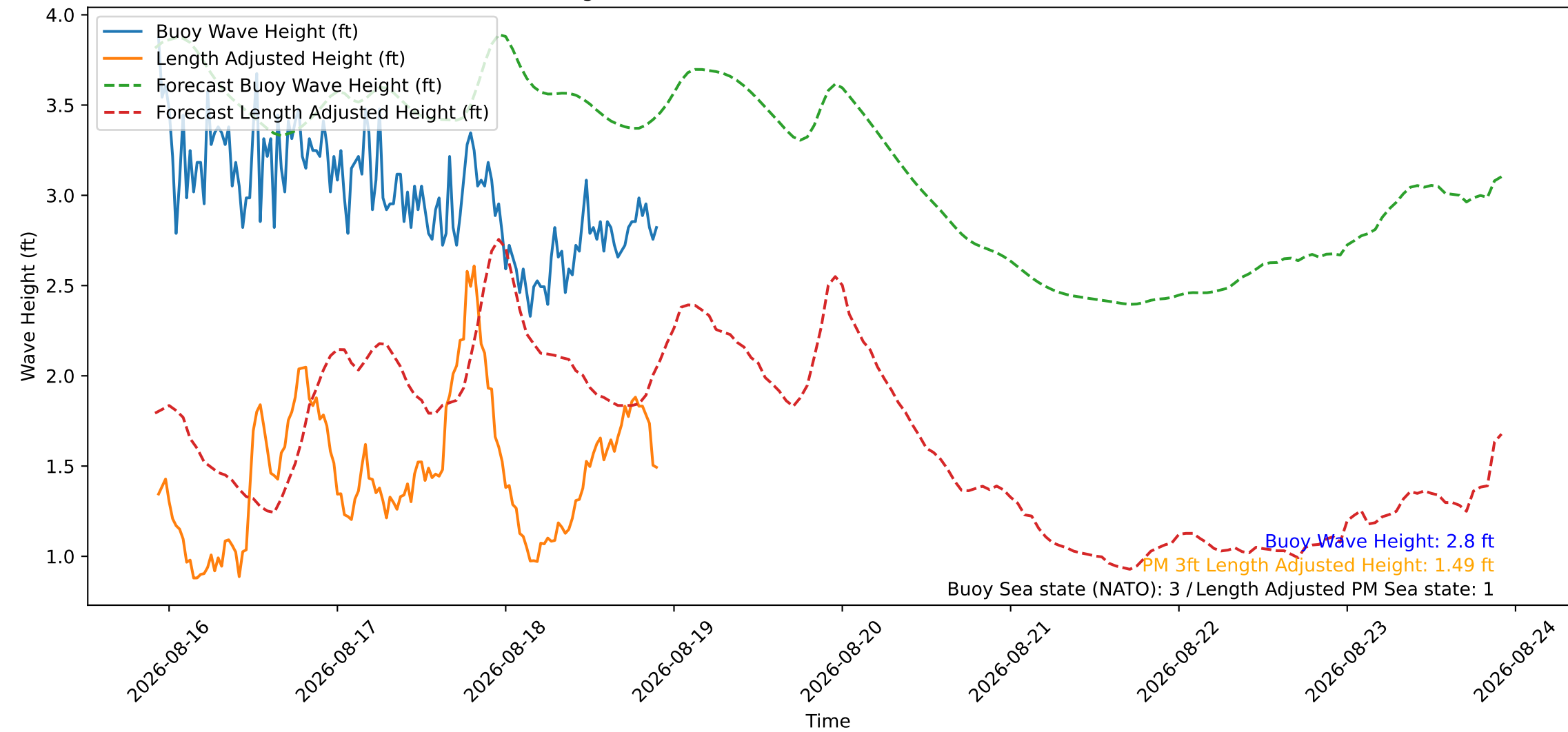
Wave Heights over Time for Red Beach at 2026-08-18 22:10:46
