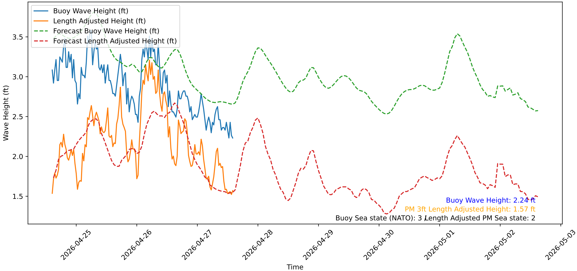
Wave Heights over Time for Green Beach at 2026-04-27 14:41:13
