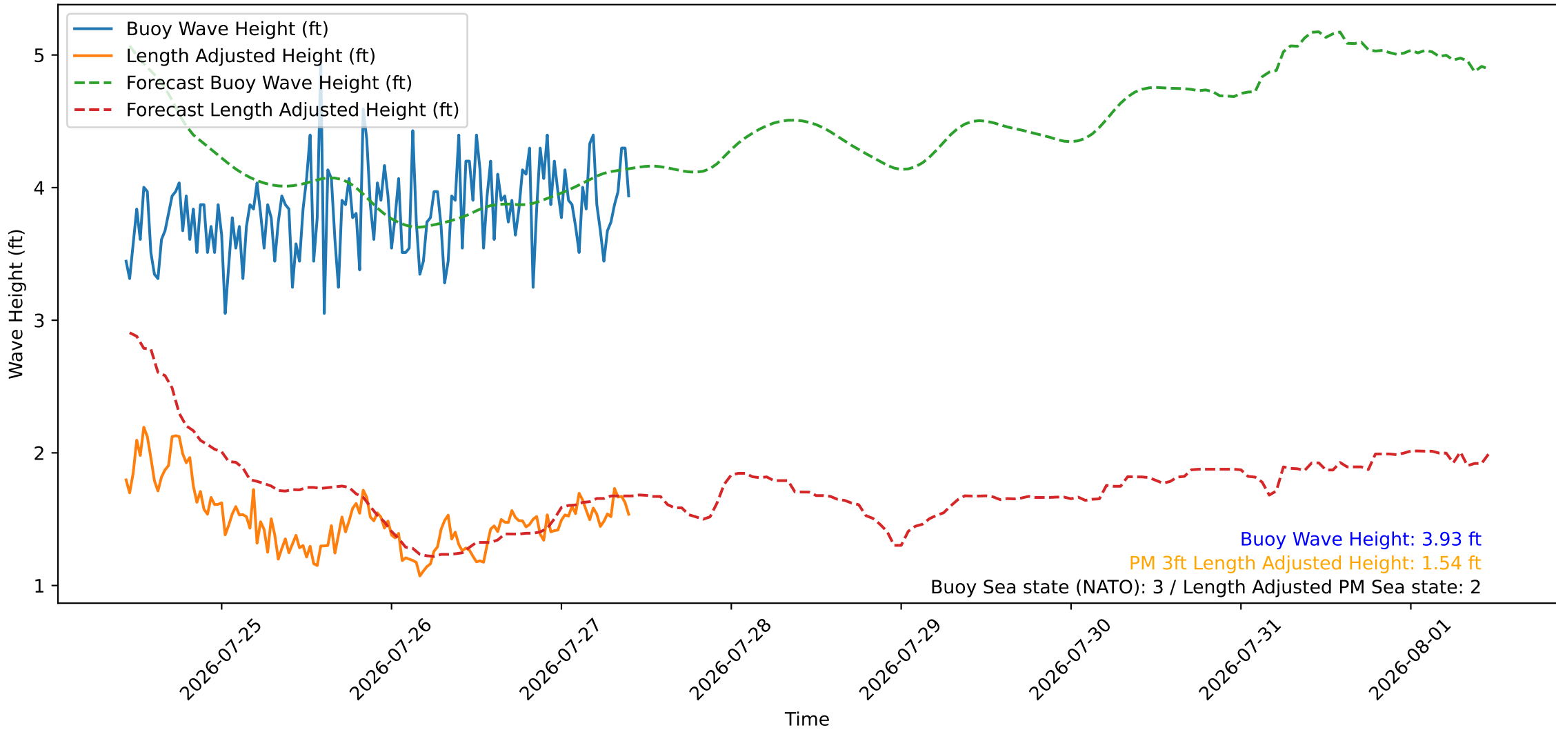
Wave Heights over Time for Oceanside Harbor at 2026-07-27 10:30:26
