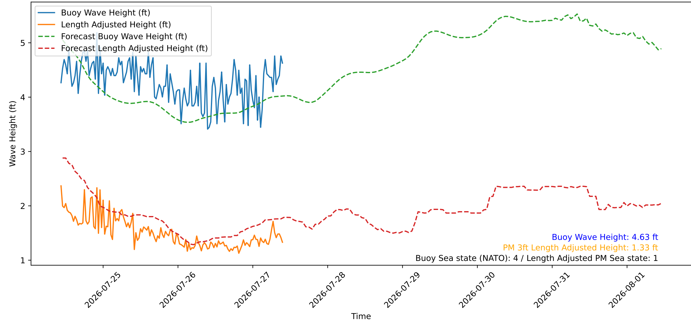
Wave Heights over Time for Green Beach at 2026-07-27 10:31:08
