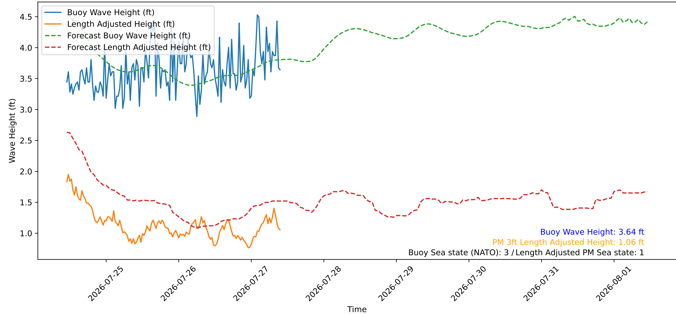
Wave Heights over Time for Red Beach at 2026-07-27 10:30:45
