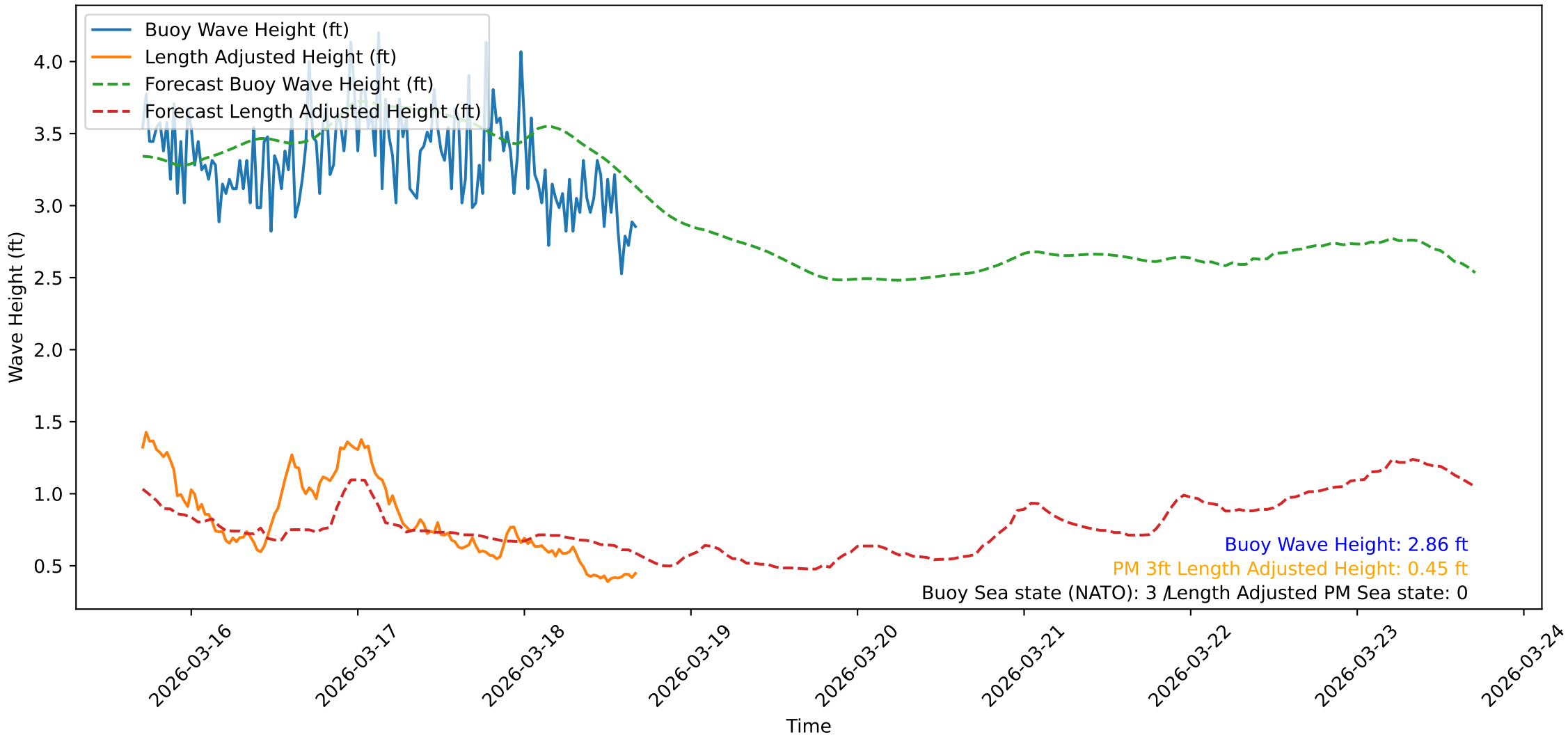
Wave Heights over Time for Green Beach at 2026-03-18 17:01:11
