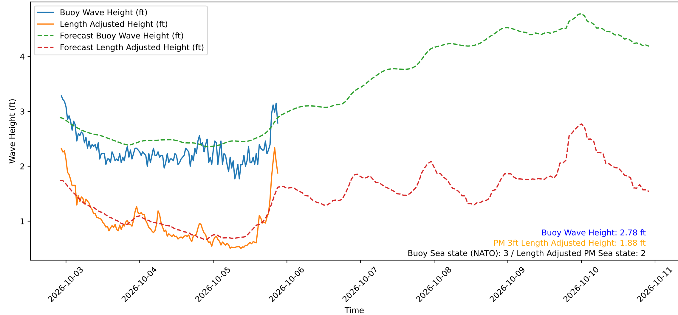
Wave Heights over Time for Green Beach at 2026-10-05 22:01:11
