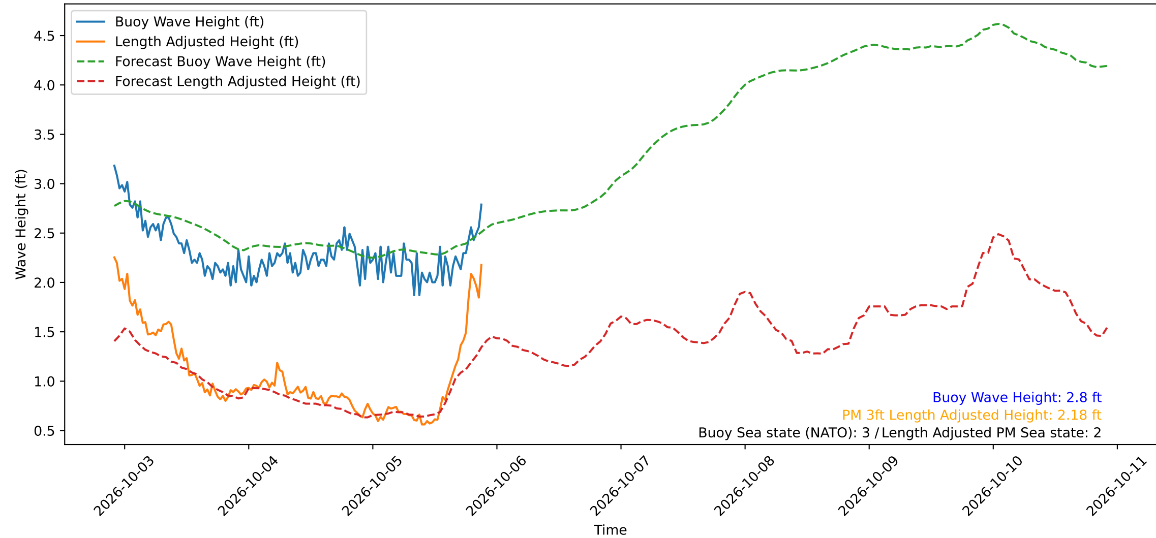
Wave Heights over Time for Oceanside Harbor at 2026-10-05 22:00:29
