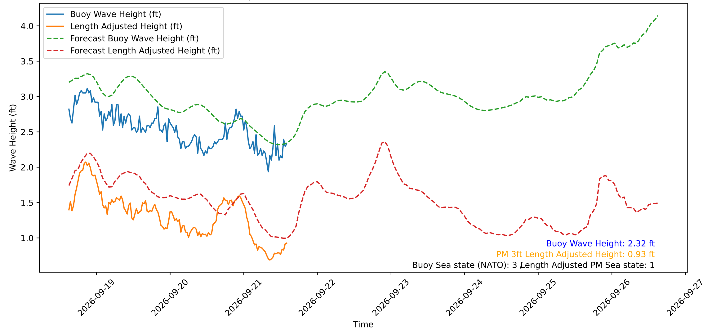
Wave Heights over Time for Green Beach at 2026-09-21 14:51:13
