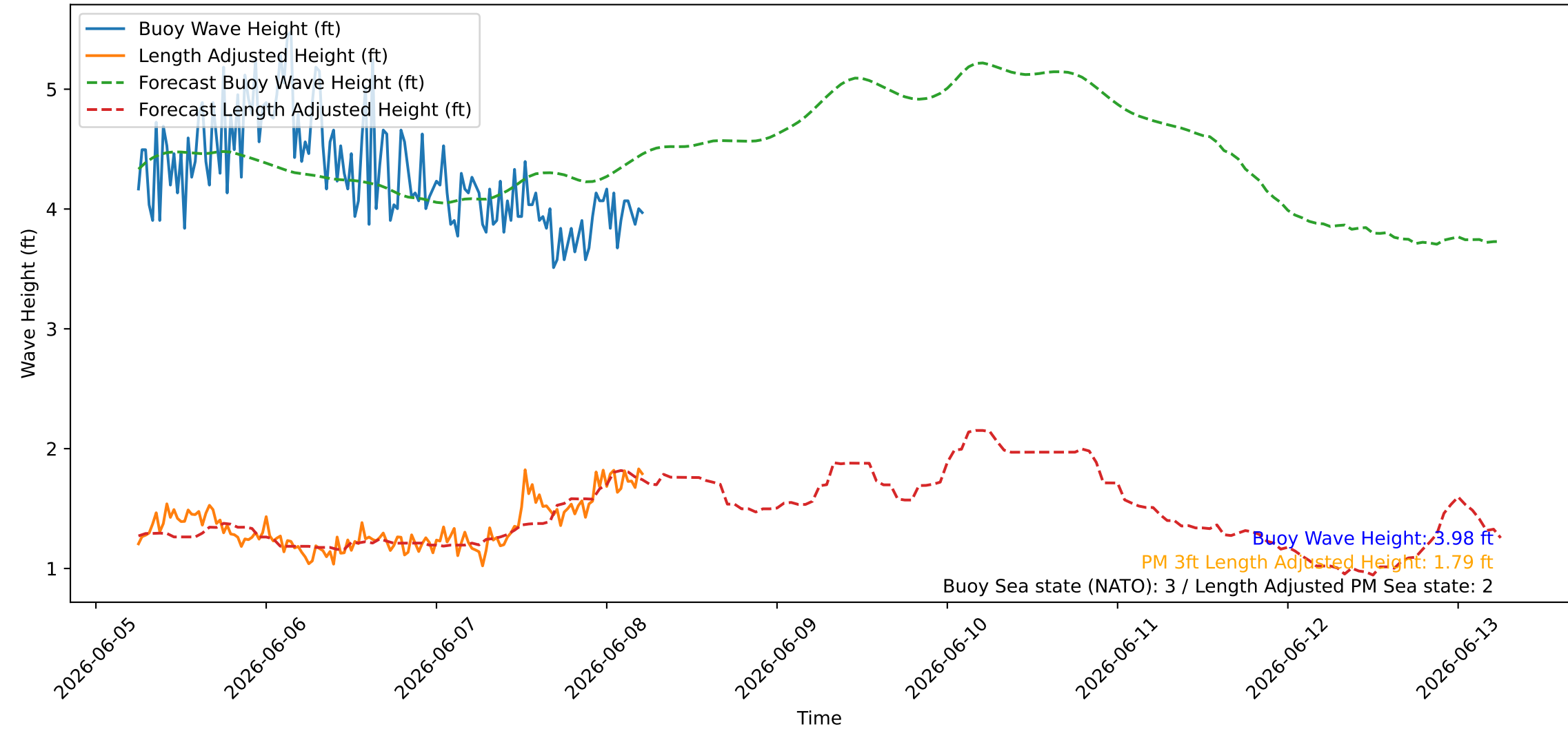
Wave Heights over Time for Oceanside Harbor at 2026-06-08 05:50:25
