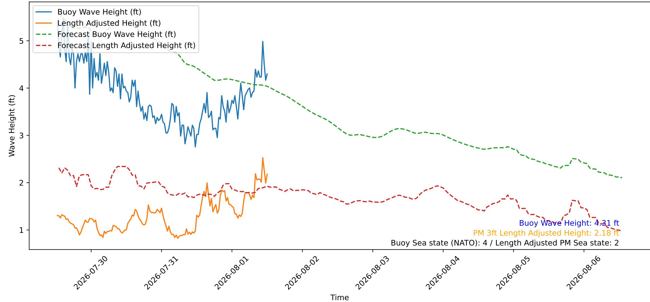
Wave Heights over Time for Green Beach at 2026-08-01 12:41:08
