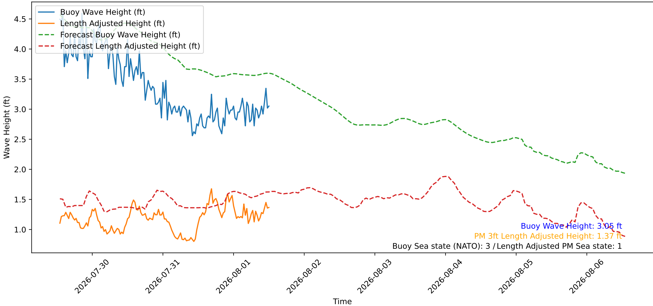
Wave Heights over Time for Red Beach at 2026-08-01 12:40:46
