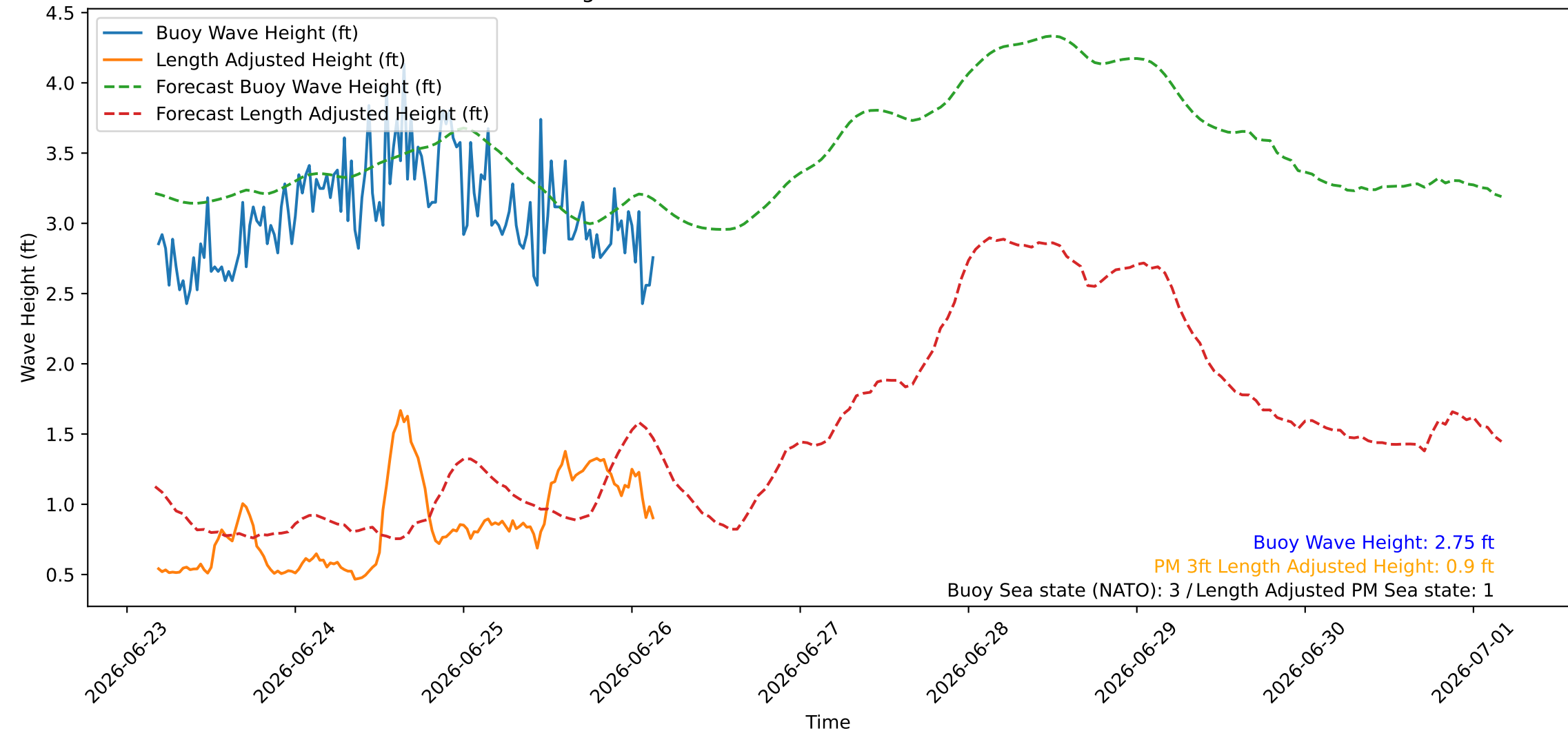
Wave Heights over Time for Red Beach at 2026-06-26 04:00:44
