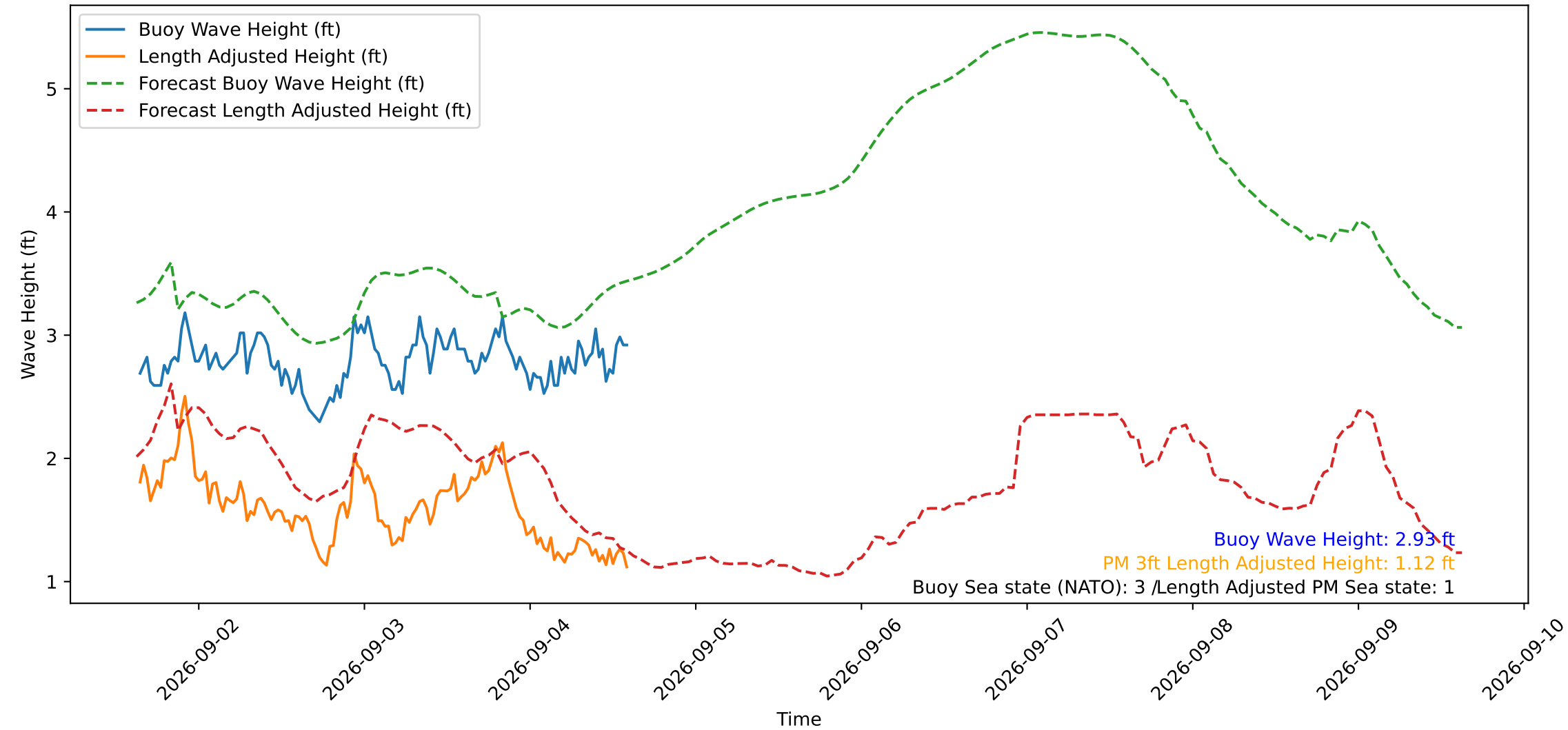
Wave Heights over Time for Red Beach at 2026-09-04 15:00:50
