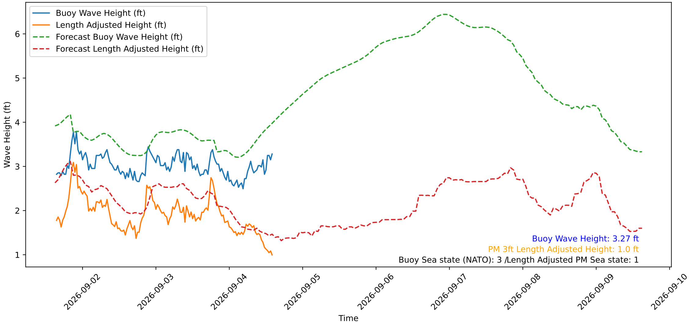
Wave Heights over Time for Green Beach at 2026-09-04 15:01:12
