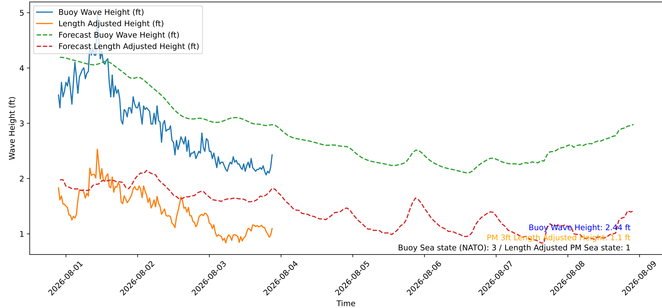
Wave Heights over Time for Green Beach at 2026-08-03 21:41:09
