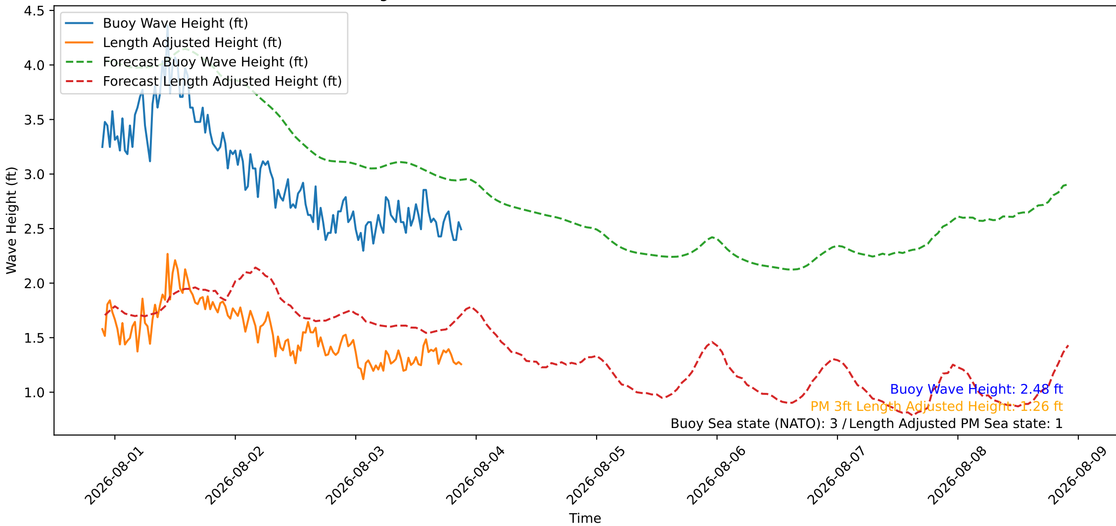
Wave Heights over Time for Oceanside Harbor at 2026-08-03 21:40:26
