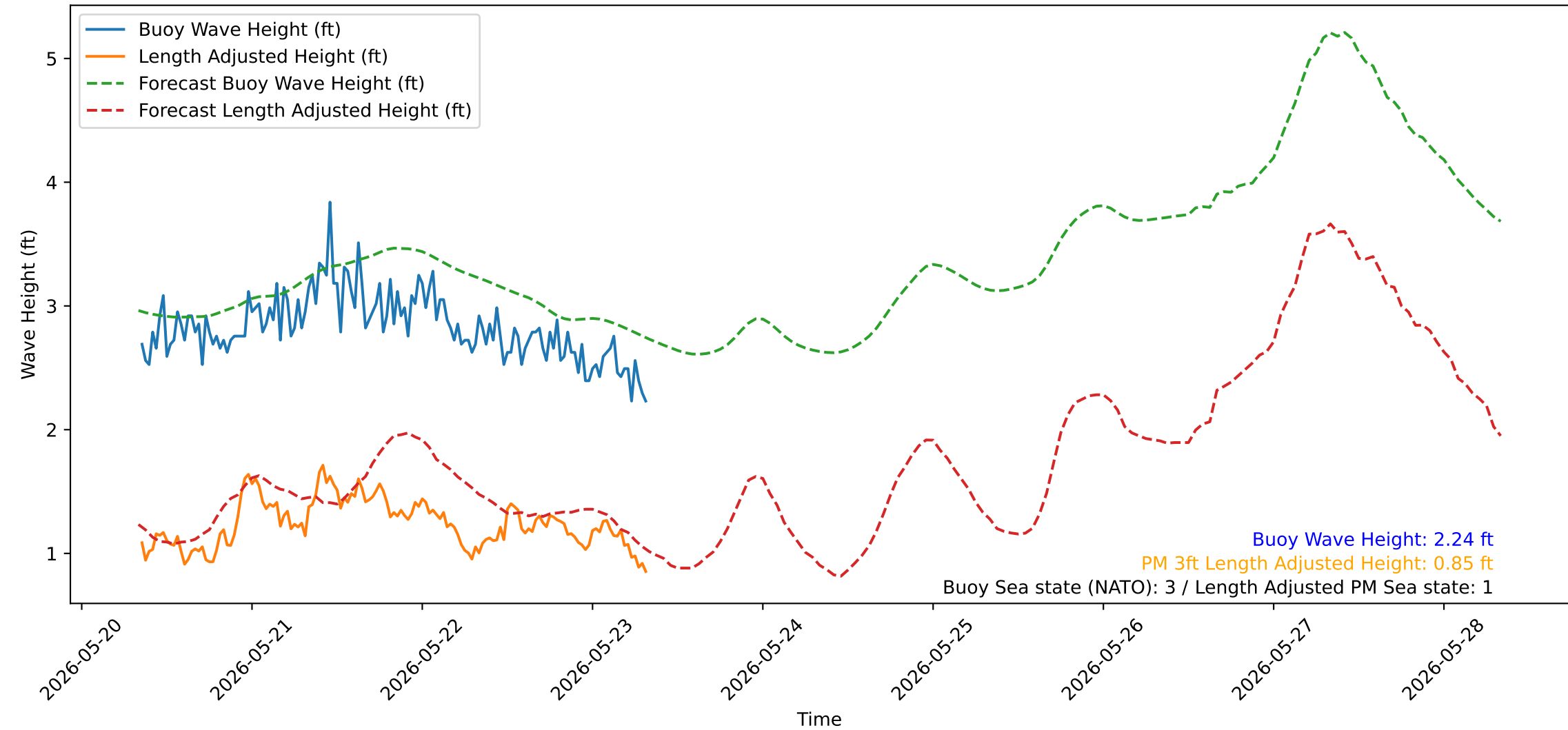
Wave Heights over Time for Oceanside Harbor at 2026-05-23 08:20:32
