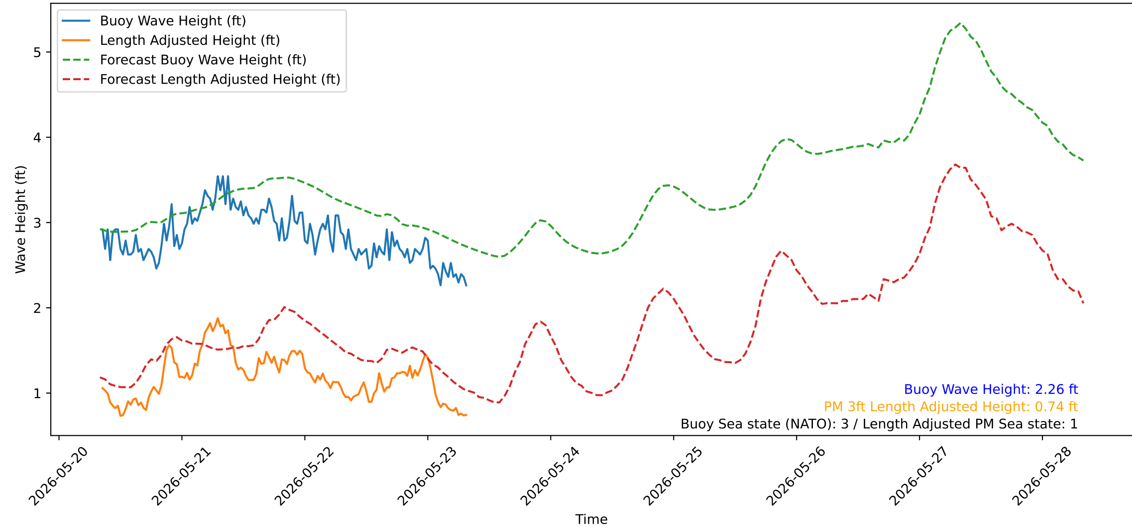
Wave Heights over Time for Green Beach at 2026-05-23 08:21:15
