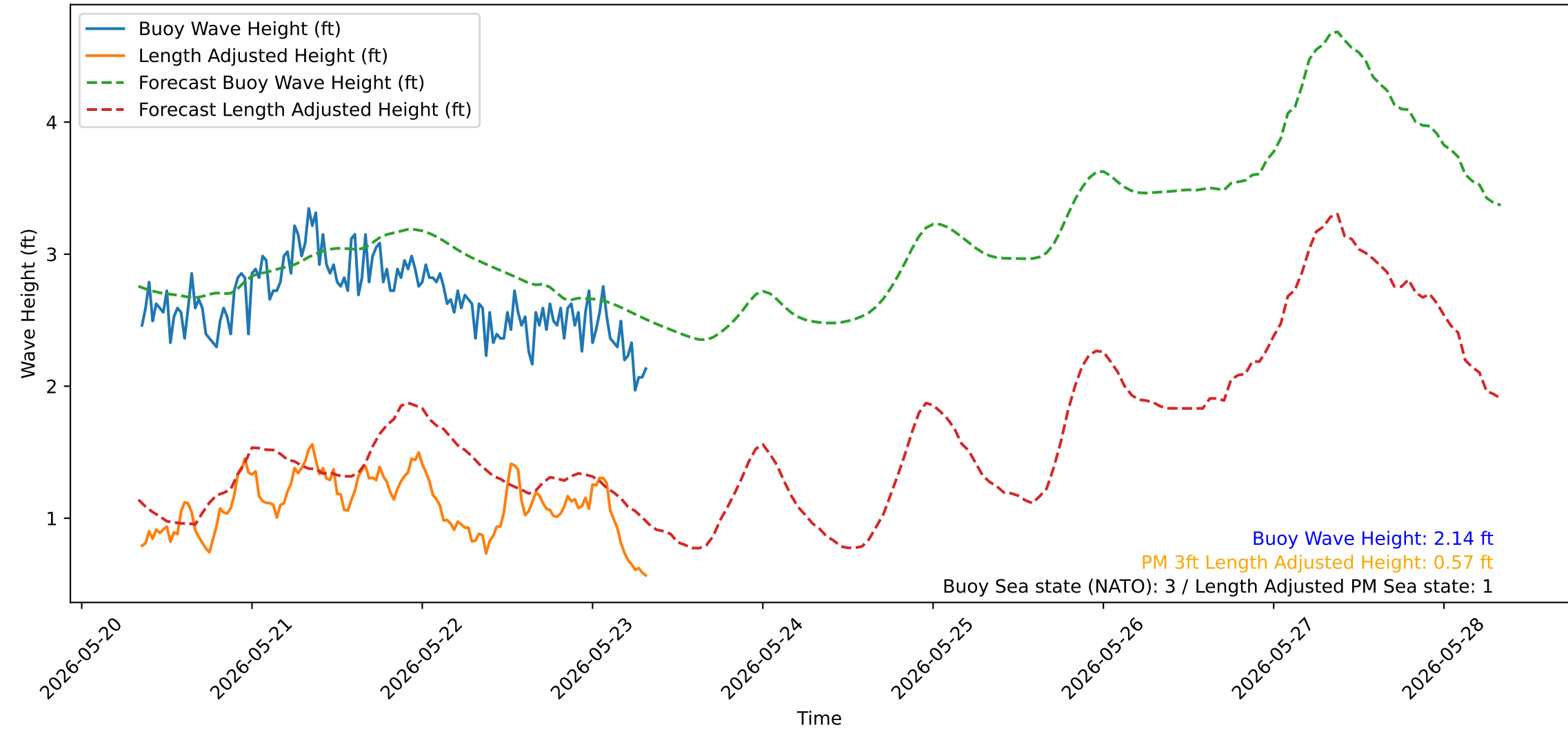
Wave Heights over Time for Red Beach at 2026-05-23 08:20:52
