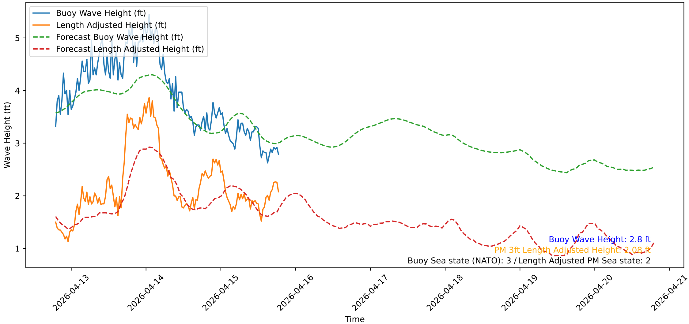
Wave Heights over Time for Oceanside Harbor at 2026-04-15 19:10:31
