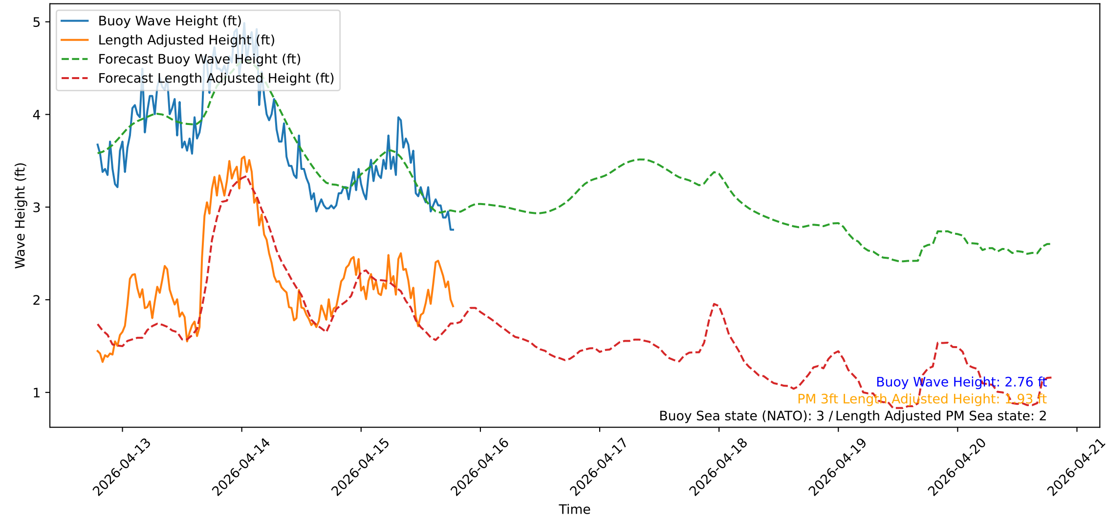
Wave Heights over Time for Green Beach at 2026-04-15 19:11:13
