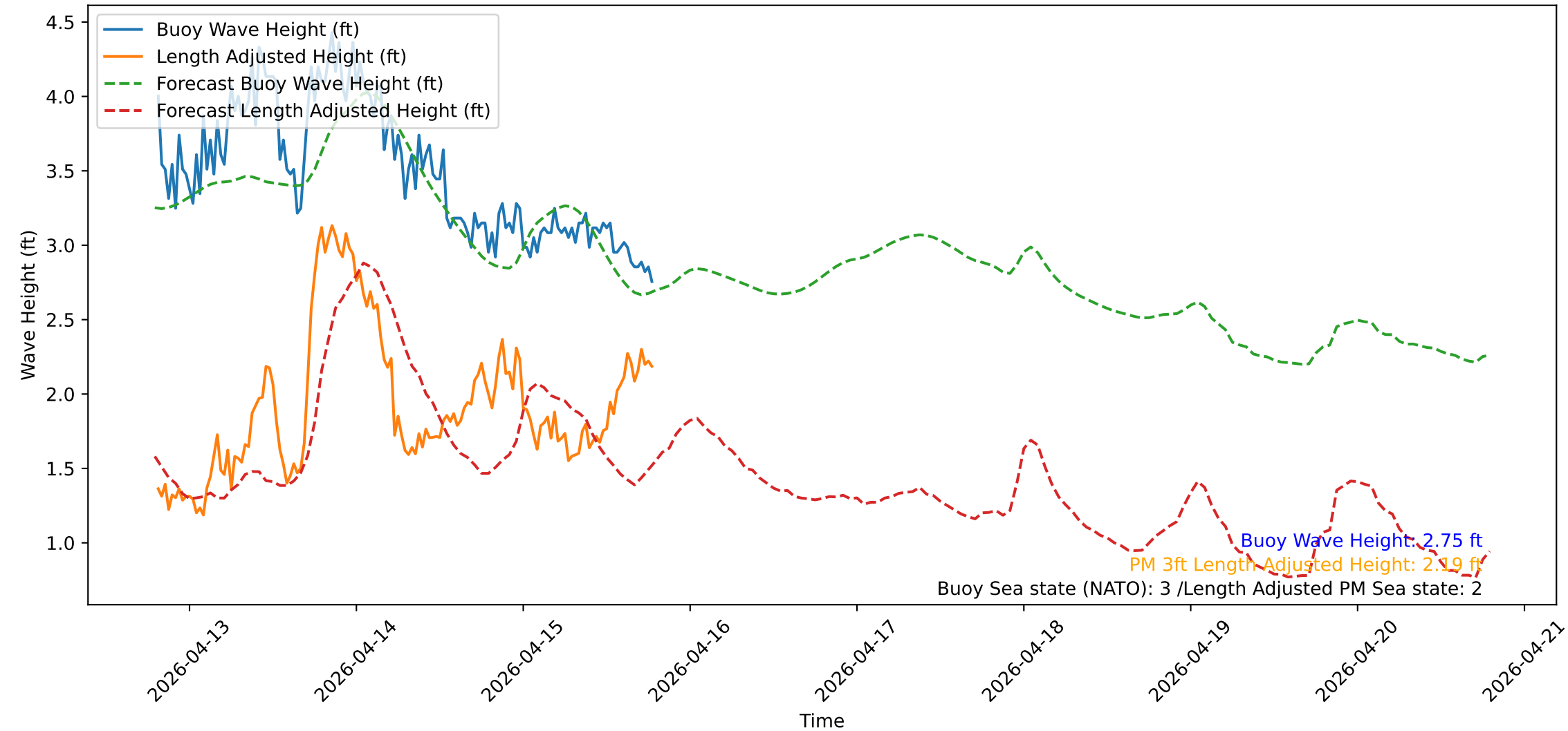
Wave Heights over Time for Red Beach at 2026-04-15 19:10:50
